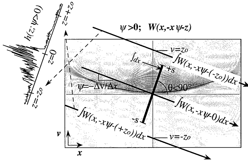
Figure 4.1. A Radon-Wigner transform for a Cubic-Phase Mask aperture function
