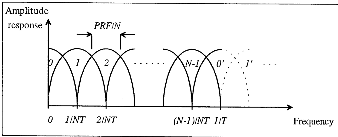
Figure 2.7. Doppler Filter Bank for N Pulses.
