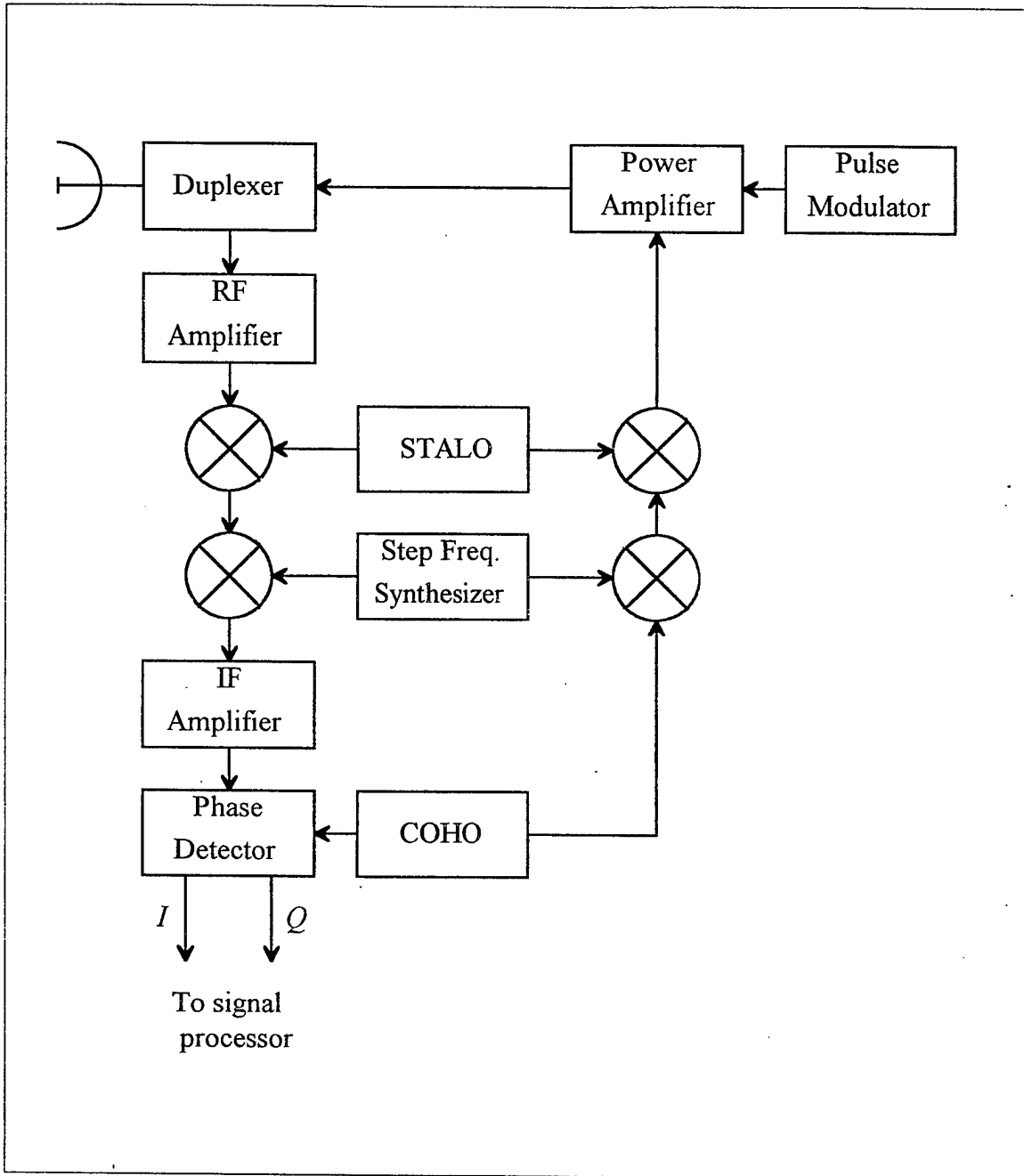
Figure 3.1. Block Diagram of the Step Frequency Radar.
