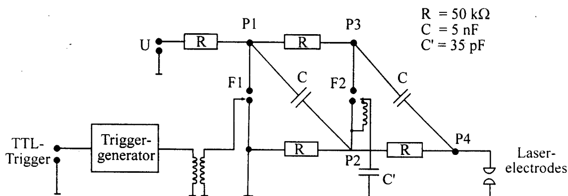
Fig. 11. Marx bank schematic.
