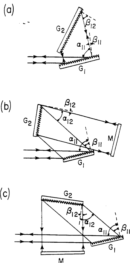
Fig. 12. Two-grating configurations.
