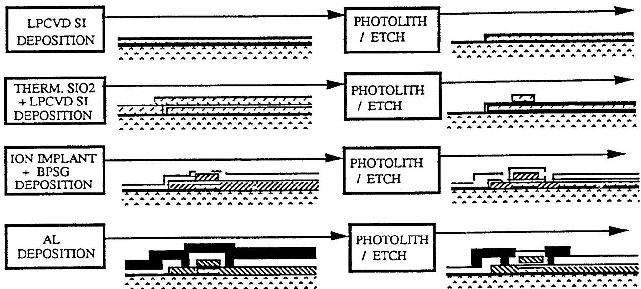
Figure 5 - Principal steps in the fabrication of p-Si AM TFTs.
