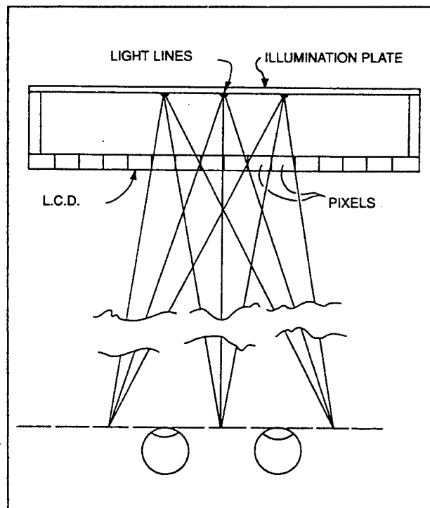
Figure 1 The Parallax Illumination Concept
