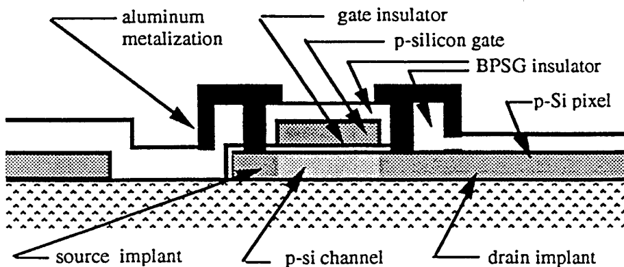
Figure 4 - Cross section of an AM TFT plate showing p-Si pixel
