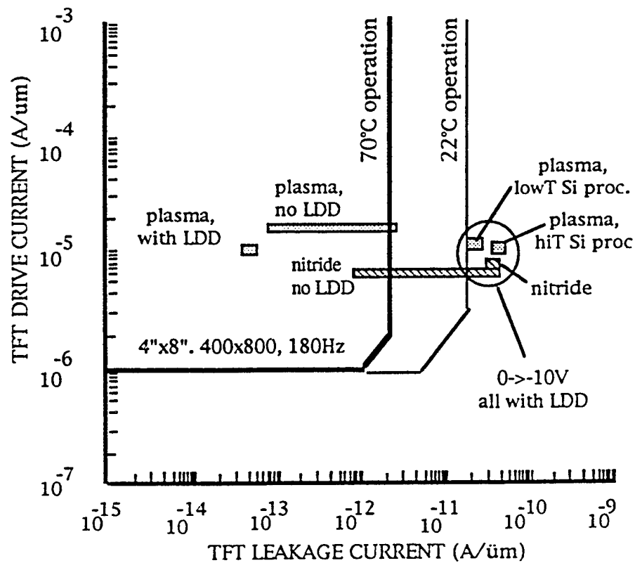
Figure 9 - Performance of TFTs fabricated in present program compared with previously processed devices. Those processed in the two present programs are shown in the ellipse.
