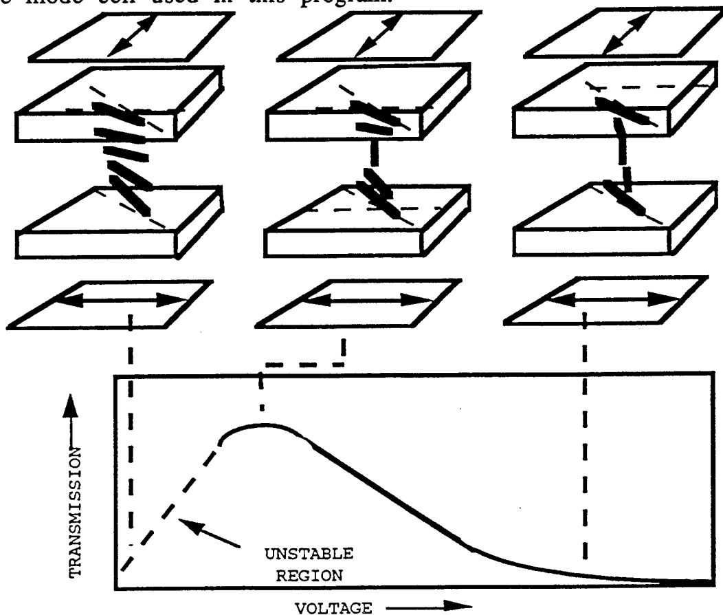
Figure 1 - "Surface mode cell" showing configuration of the liquid crystal molecules for representative voltages and the transfer curve ( light output vs voltage ).
