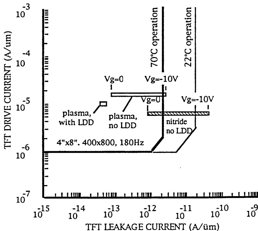
Figure 7 - Data from Figure 6 plotted on TFT performance requirements chart.
