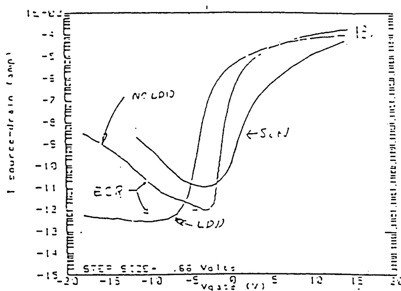
Figure 6 - Performance of TFTs processed on 4" diameter quartz wafers.
