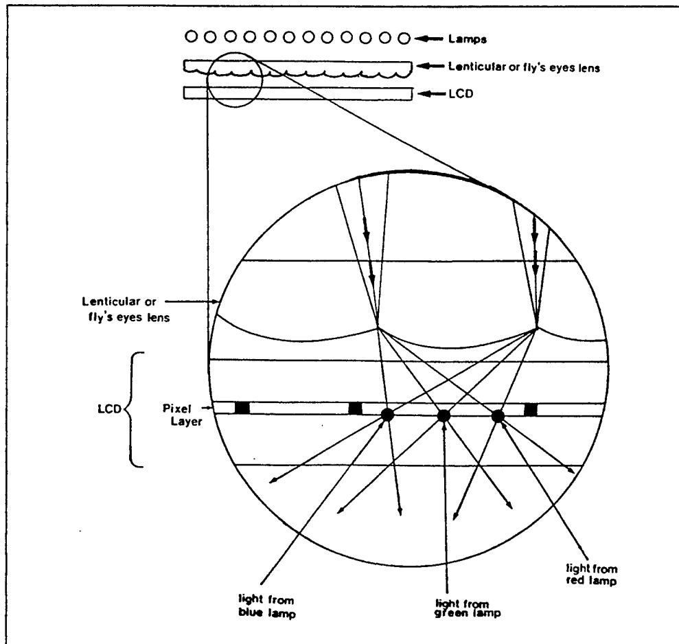
Figure 12 Creation of Field-Sequential-Color Illumination Patterns with a Fly's Eye Lens
