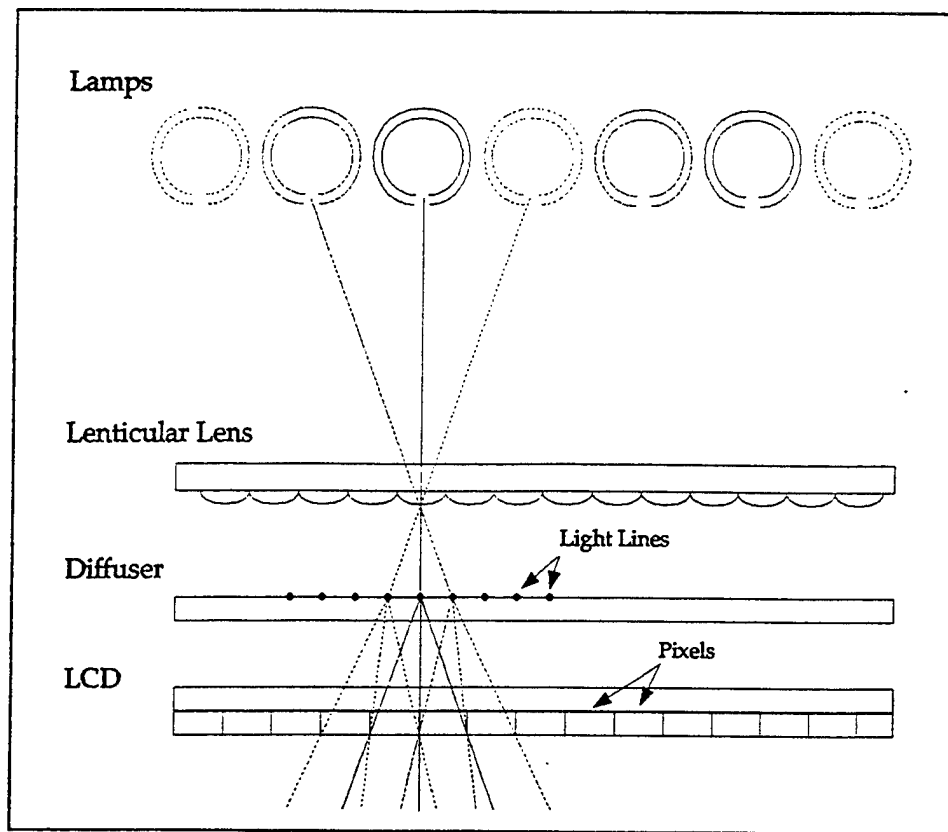
Figure 5 Electro-Optical Dynamic Parallax Illumination
