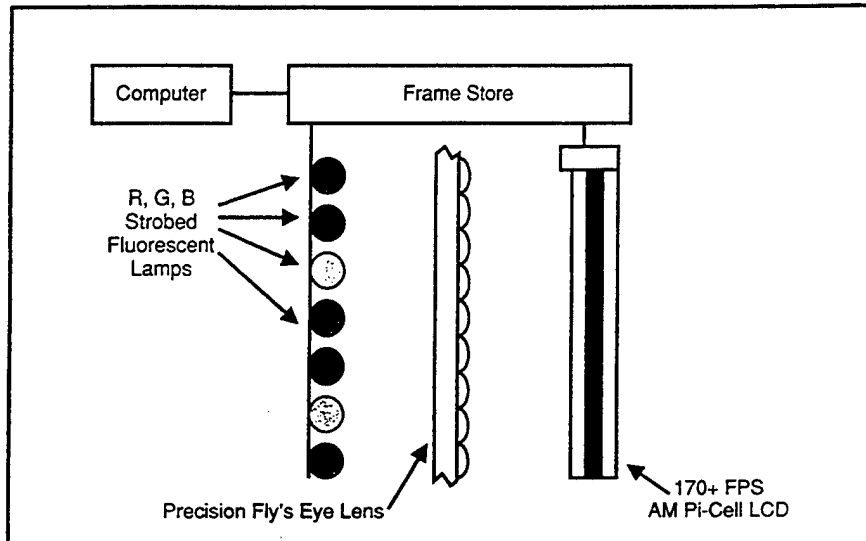
Figure 13 Breadboard System Major Components
