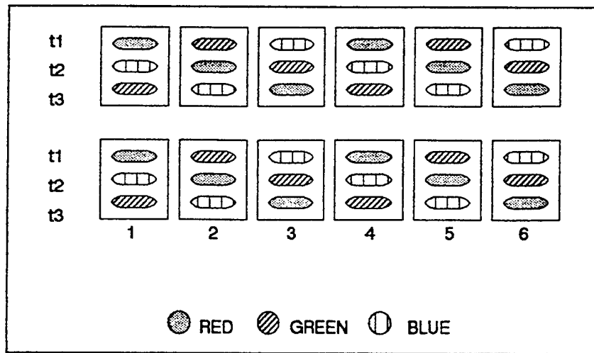
Figure 11 Field-Sequential-Color Illumination Pattern
