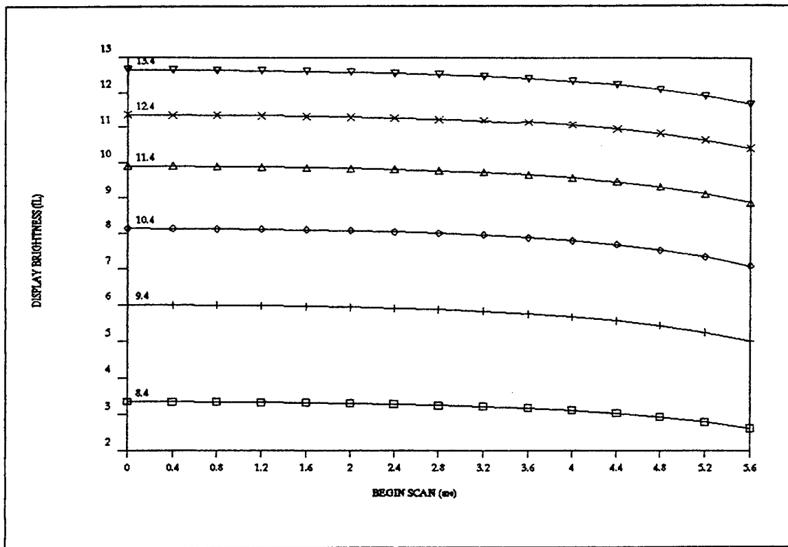
Figure 16 Screen Luminance Calculations versus the Frame Period
