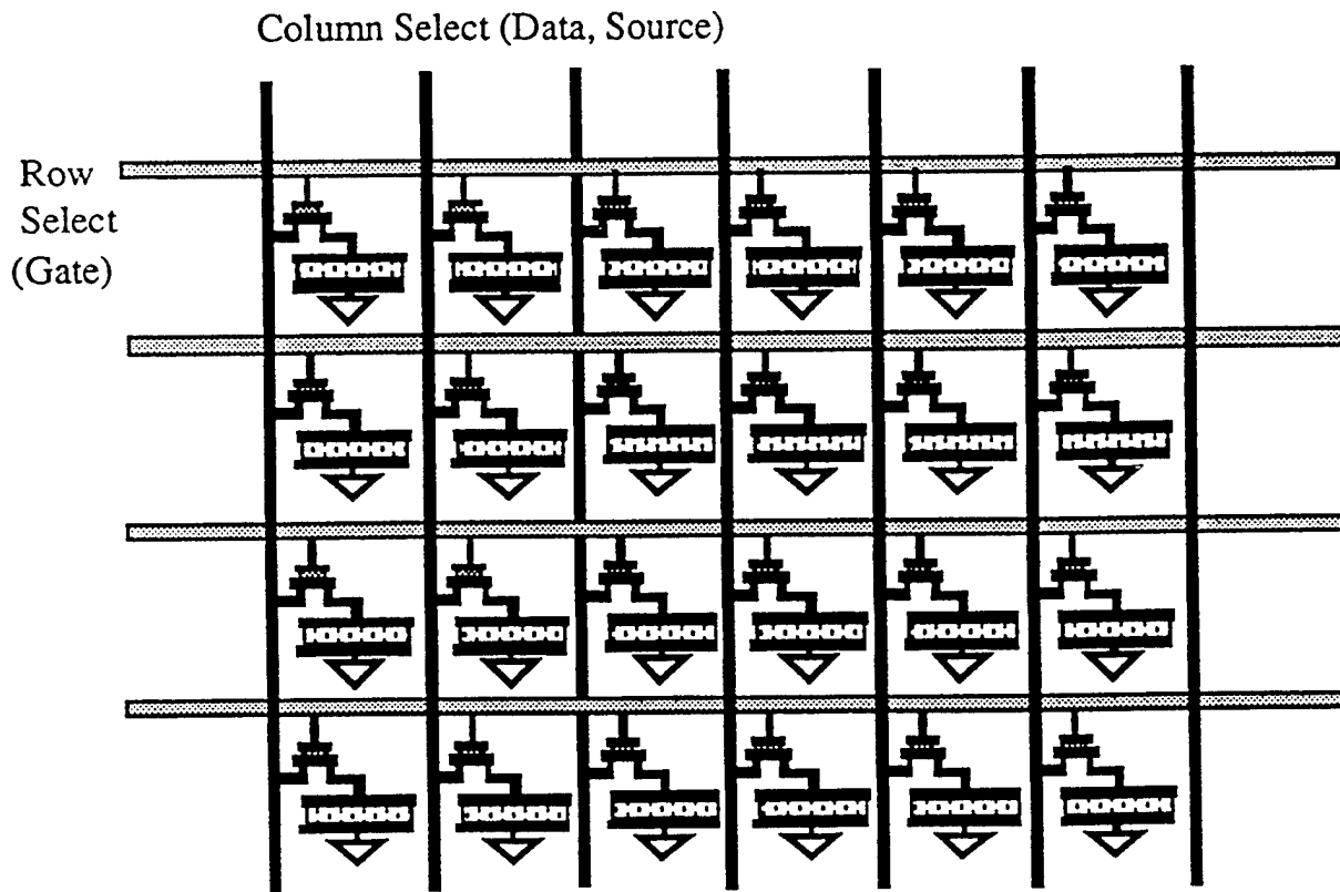
Figure 2 - Active matrix TFT array driving individual pixels, all connected to a common ground plane.
