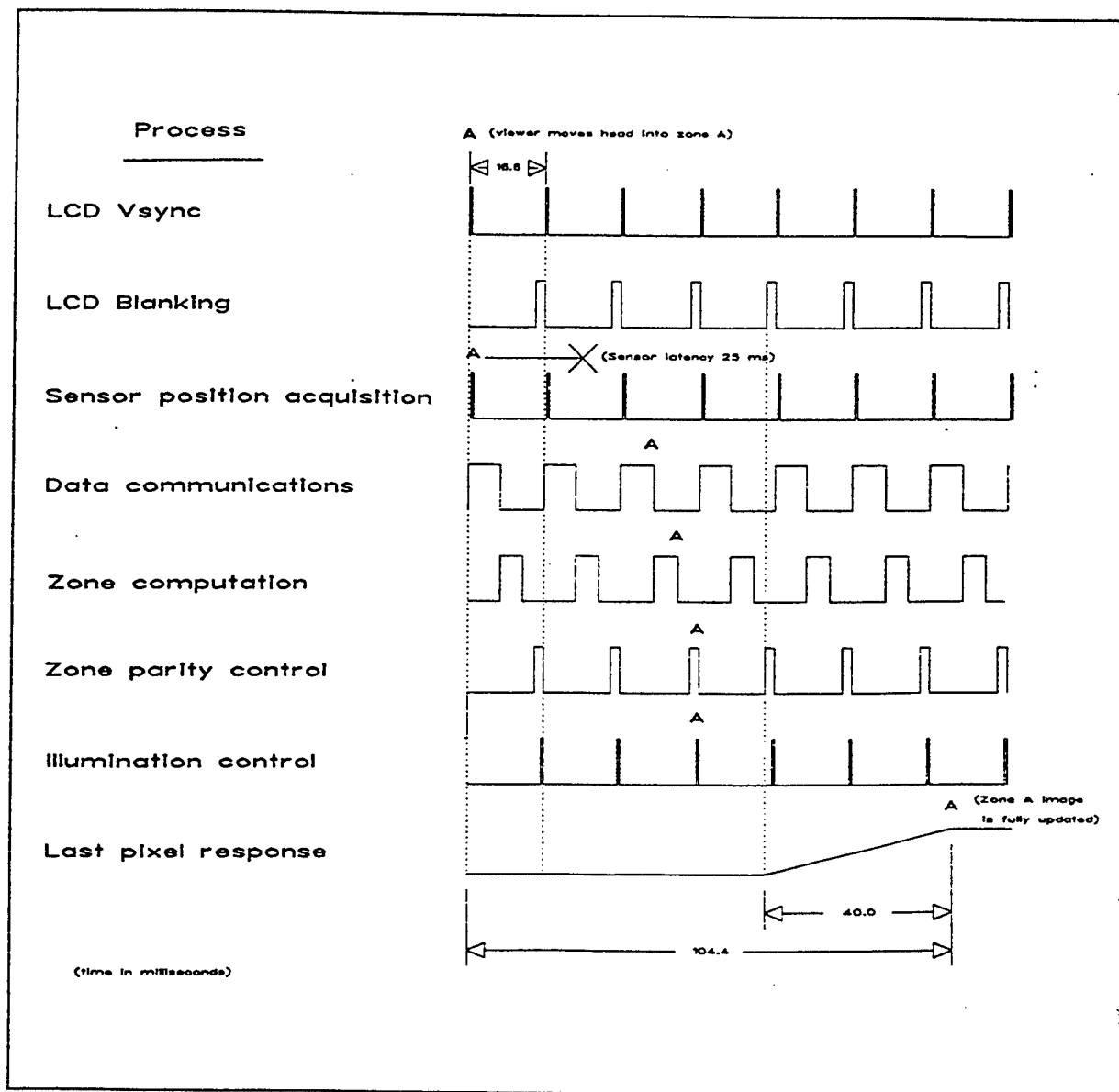
Figure 9 Head Tracking Display Update Timing
