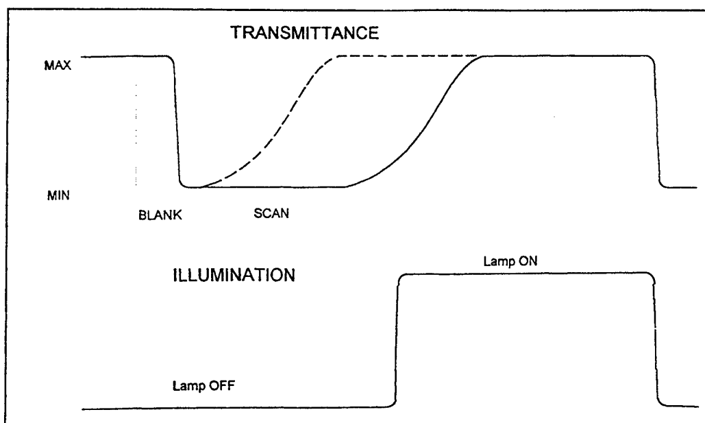
Figure 14 LCD and Light Source Operation
