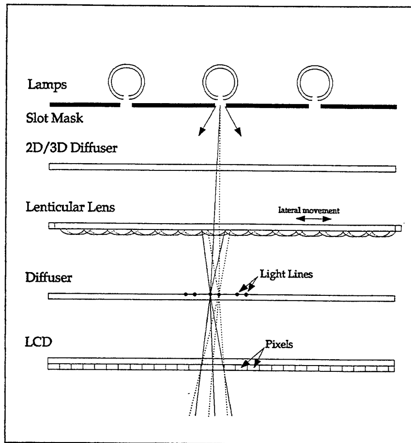
Figure 4 Electro-Mechanical Dynamic Parallax Illumination
