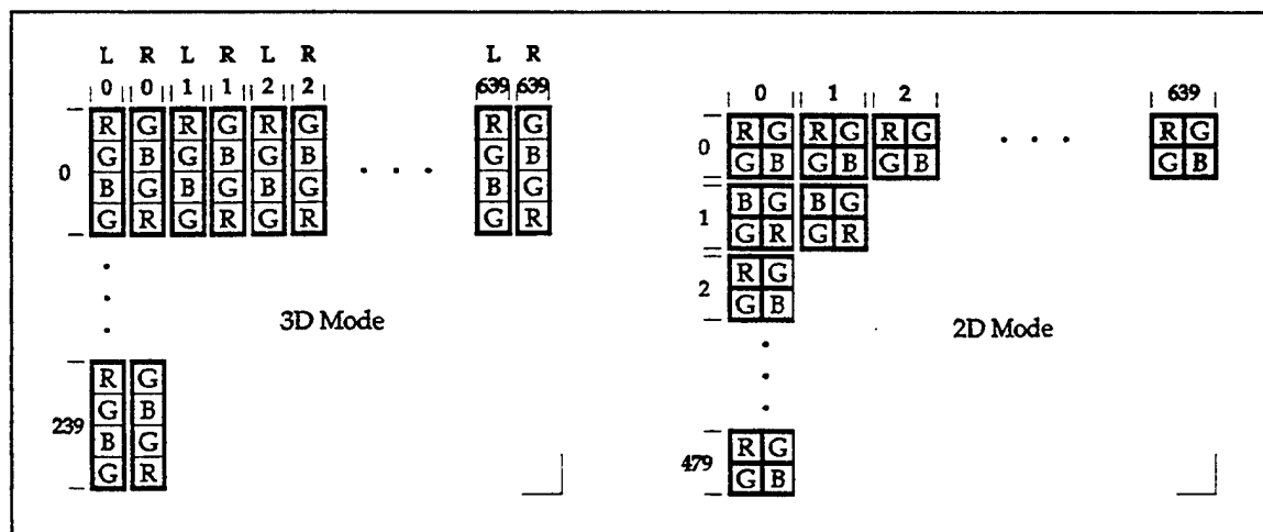
Figure 7 Cockpit Prototype LCD Pixel Structure
