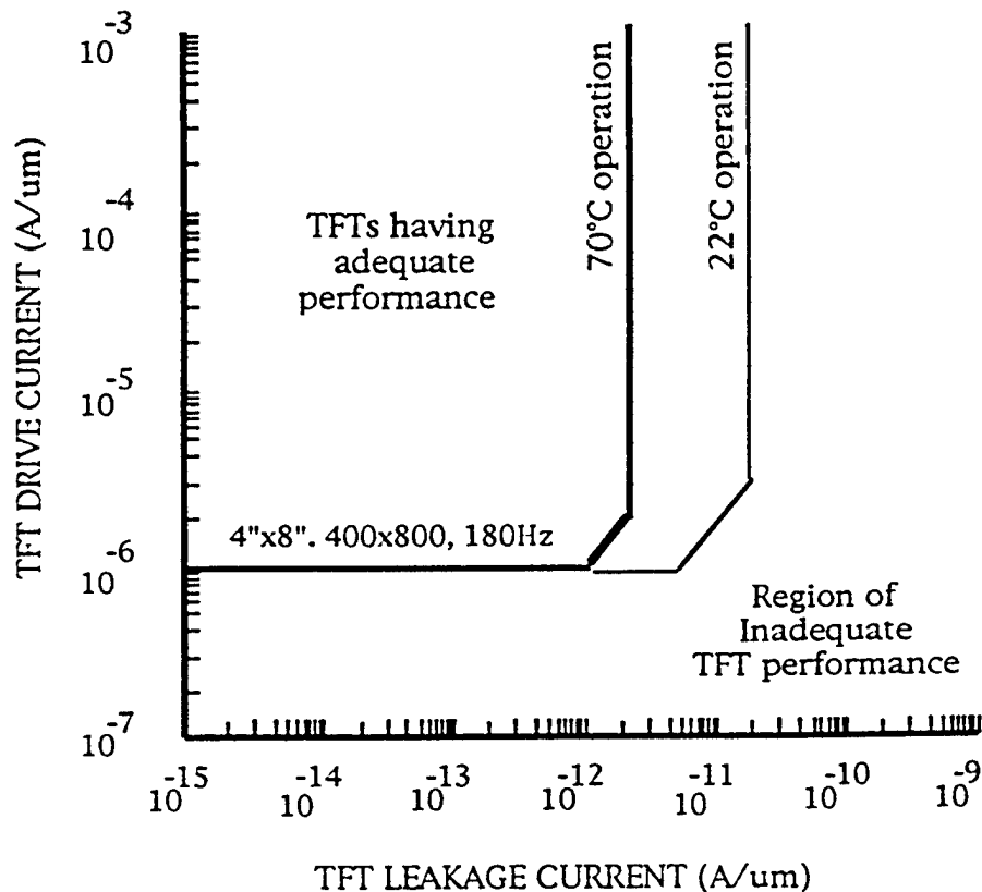
Figure 3 Performance requirements for TFTs used in an AM. Adequate performance occurs only for devices having drive and leakage in the region indicated
