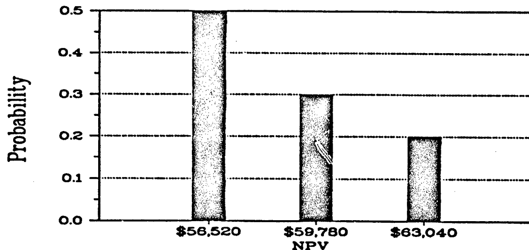
Figure 7I Histogram Graph
