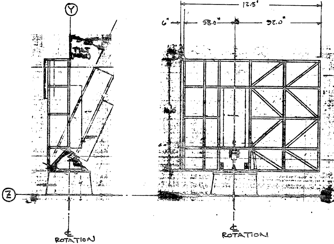
PEDESTAL-ANTENNA ASSEMBLY CONFIGURATION
