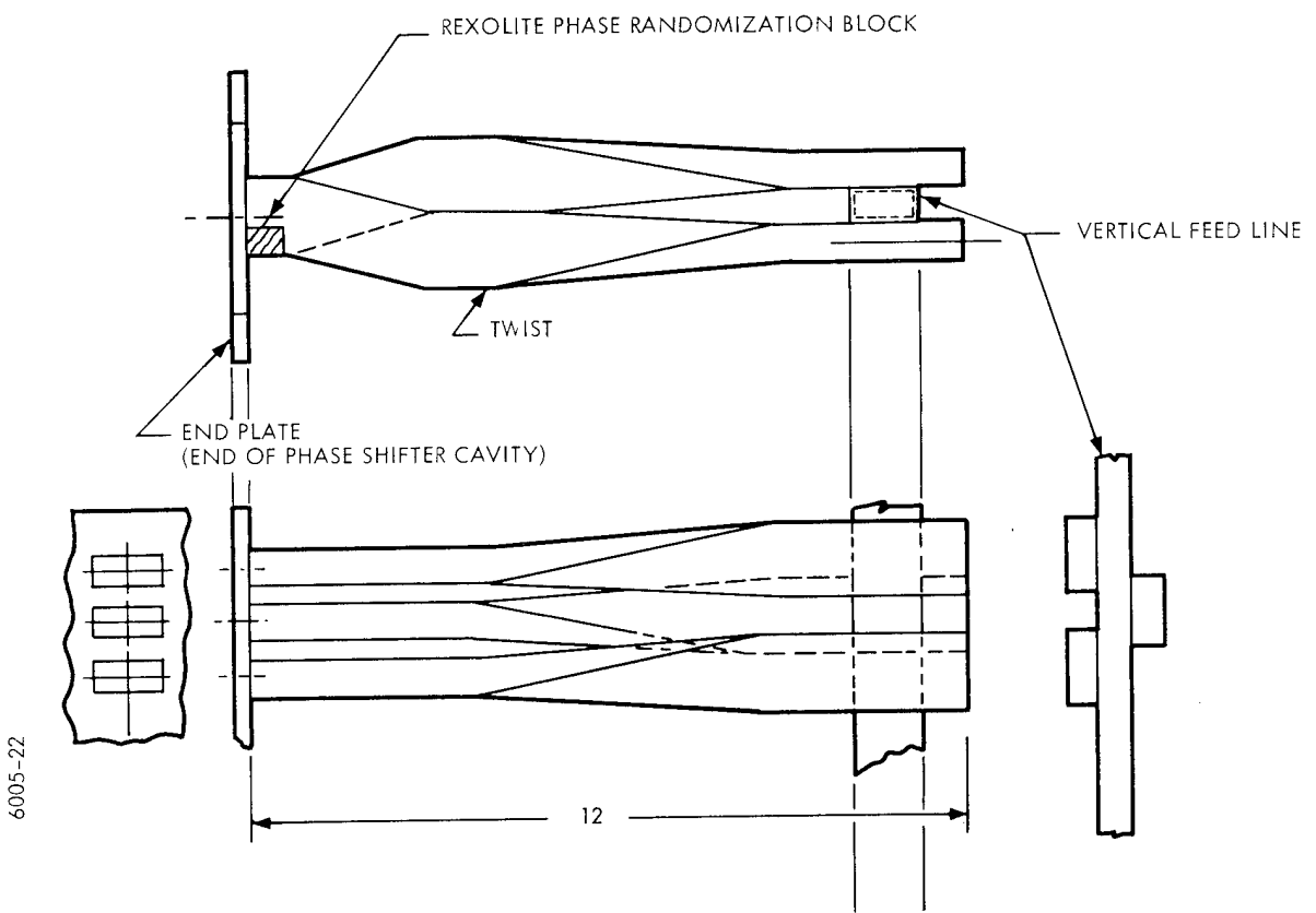
Figure 26. Phase Randomization Block Location in Coupler
