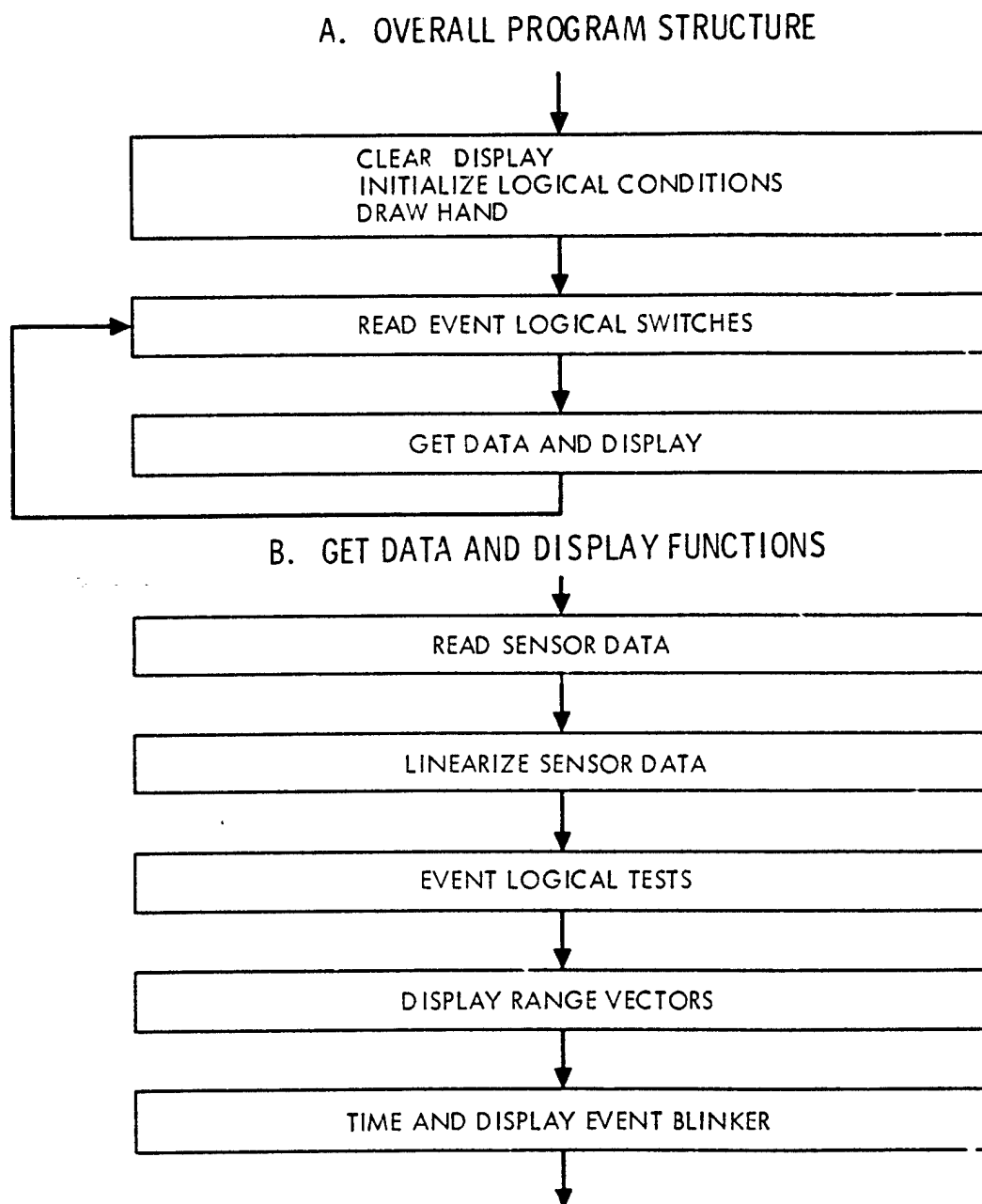
Figure 15. Software System Structure for Proximity Sensor Data Graphics Display in the JPL Teleoperator Project
