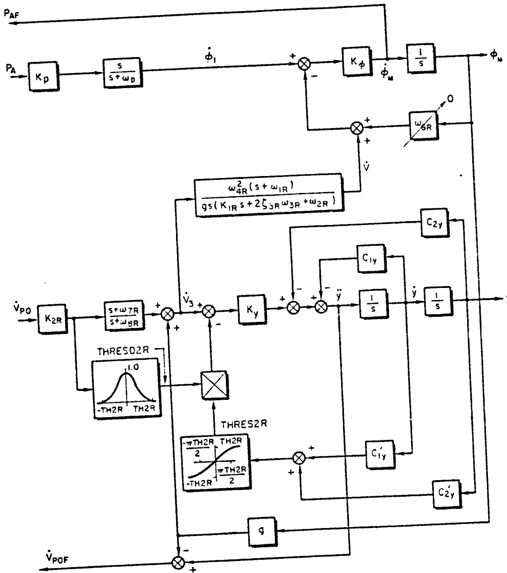
Figure 6. LAMARS Drive Logic Washout with Nonlinear Feedback Added to Specific Force Path Only
