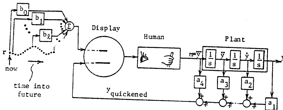
Fig. 3 Naive Combination of Quickened and Preview Displays
