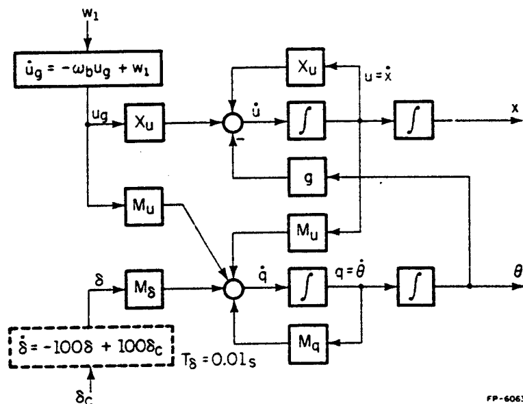
Figure 2: Block Diagram of the Aircraft Dynamics
