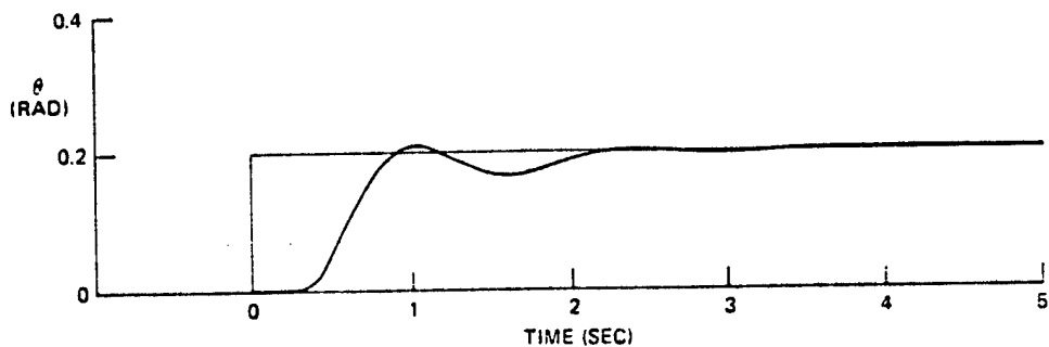
Figure 11. Step Target Tracking Response of Baseline YF-17
