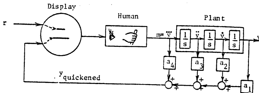
Fig. 1 Signal Quickening (Pursuit Type)
