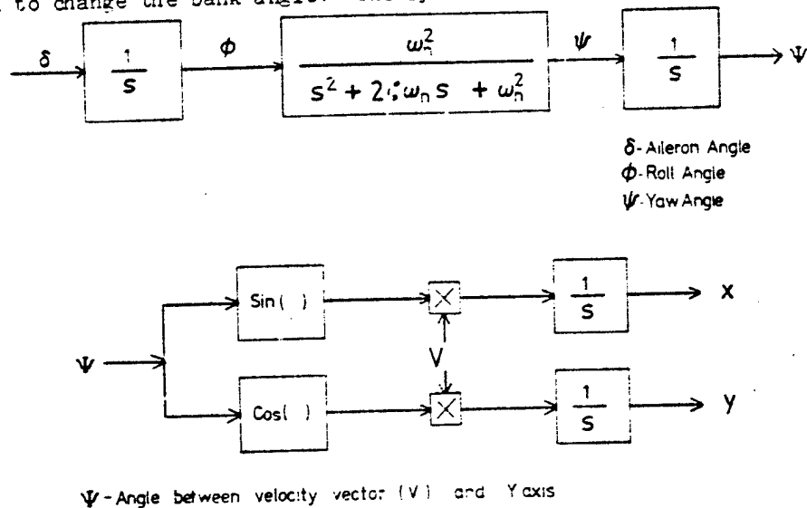
Fig 1 Simplified Lateral Dynamics
