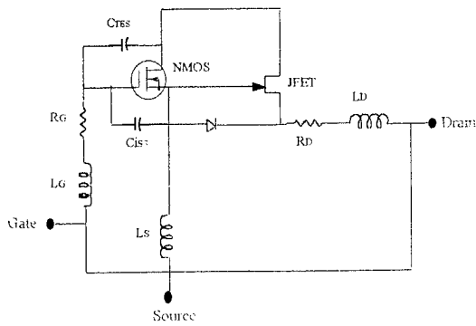
Fig. 7 Circuit model for LDMOSFET
