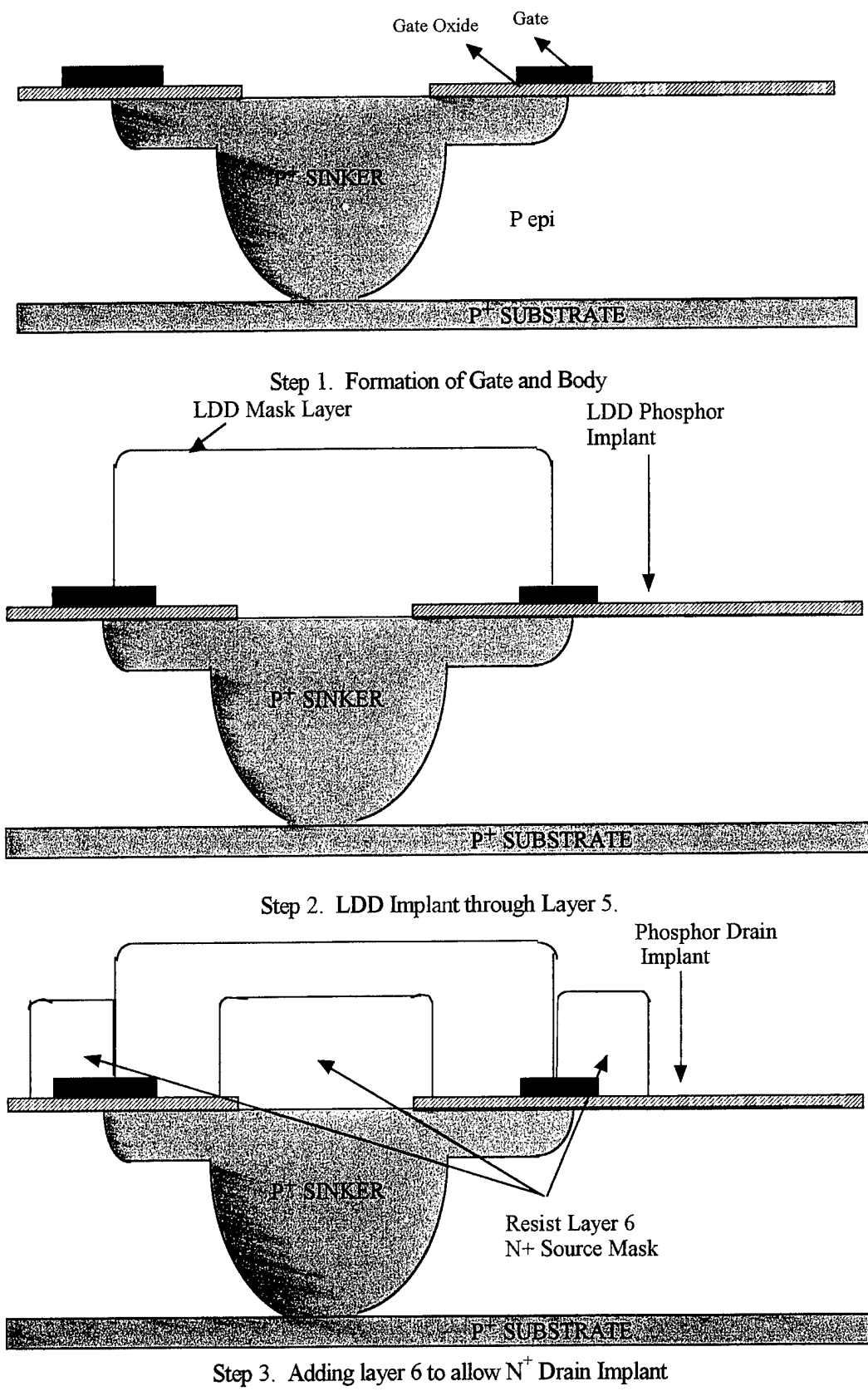
Fig. 1(a) Process sequence for 80V silicon RF LDMOSFET.
