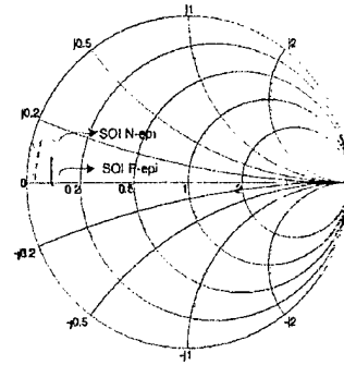
Fig.16(d) S22 data for SOI devices
