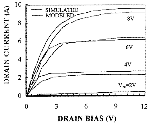
Fig.15(d) I-V curves for Str 4.
