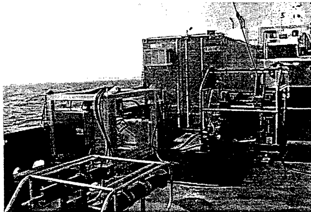
Figure 4. The winch (framework to the right) and the power pack assembly (framework left) on the deck of the Diane G.
