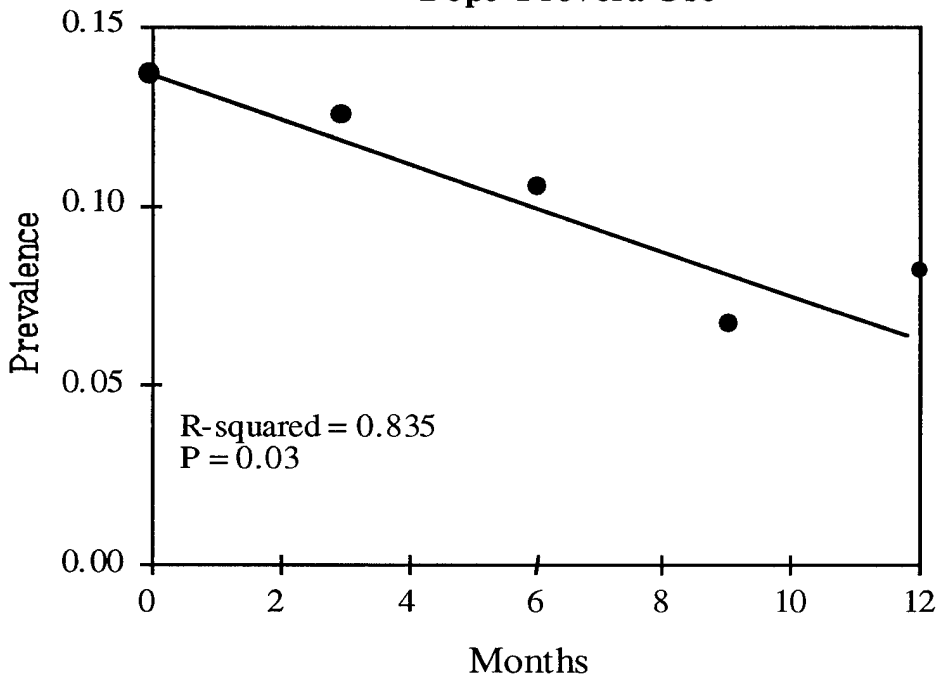
Figure 4 : Prevalence of Mastalgia by Duration of Depo-Provera Use
