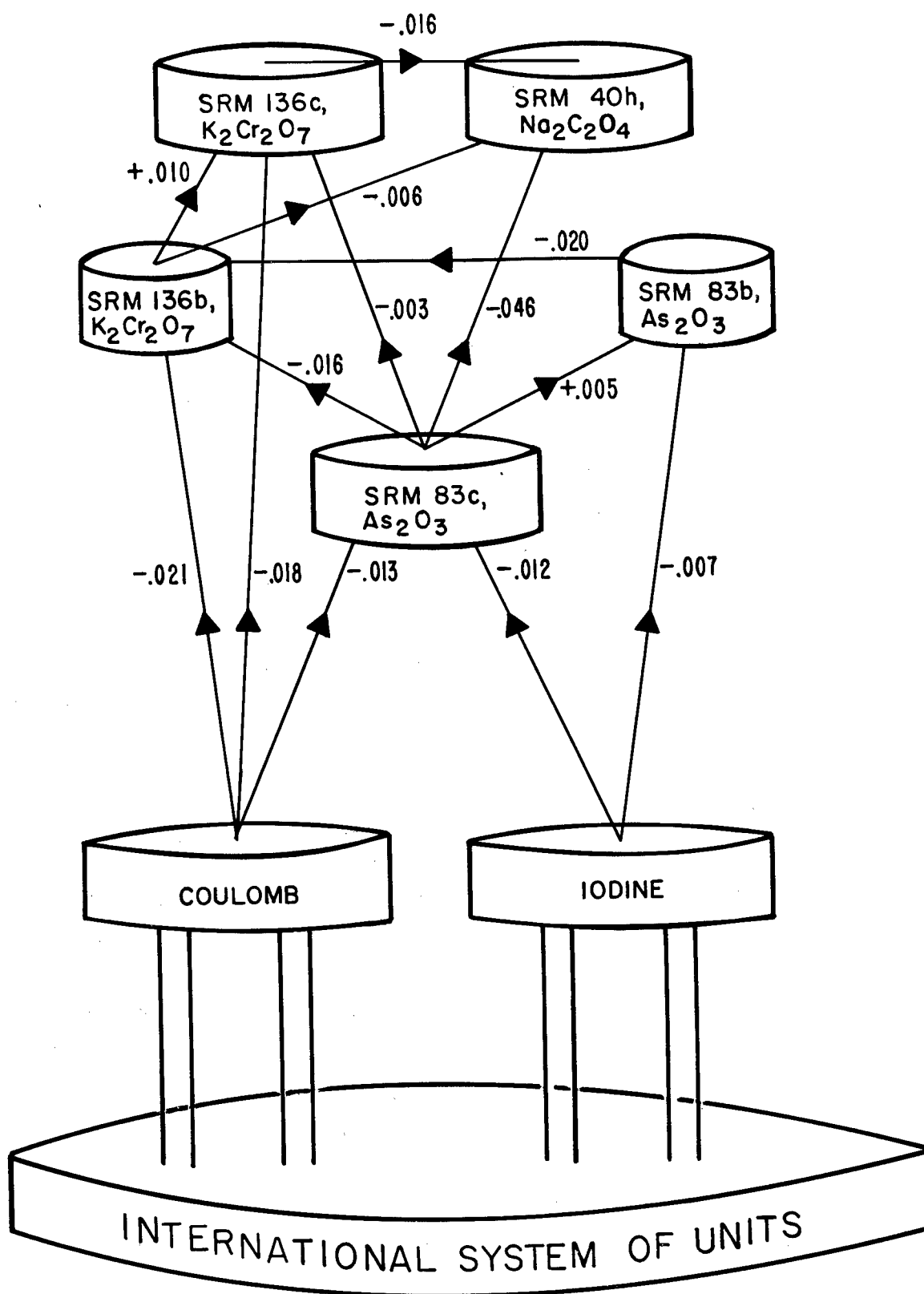
Figure 10. Intercomparison of redox Standard Reference Materials.
