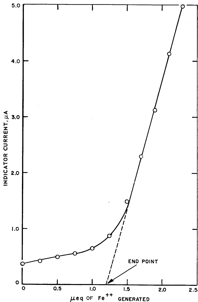
Figure 7. Typical end-point determination.
