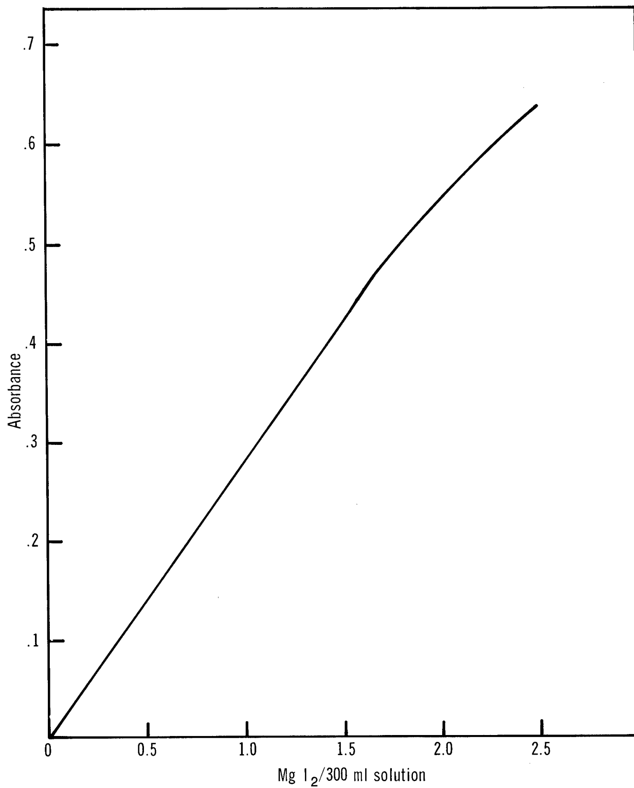
Figure 11. Photometric calibration curve for excess iodine.
