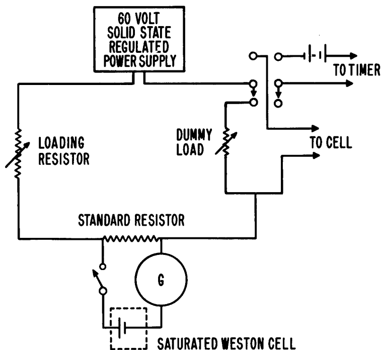
Figure 2. High accuracy constant-current and timing circuit.
