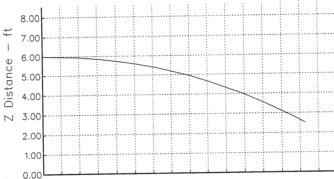
a. Altitude vs Distance Traveled ( Gravity drop )
