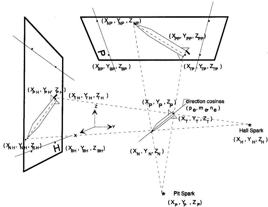
Figure 5.4 Projectile Attitude / Positioning Scheme
