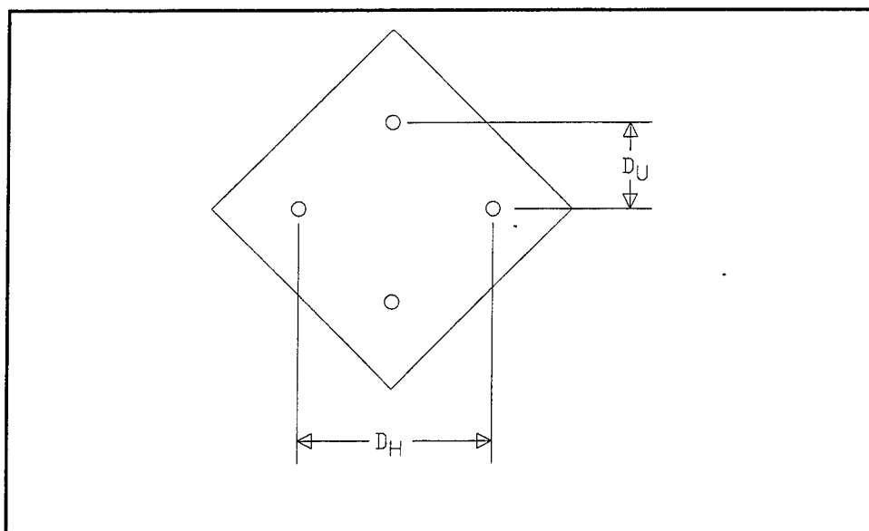
Figure 8. Schematic of core-loc placement grid
