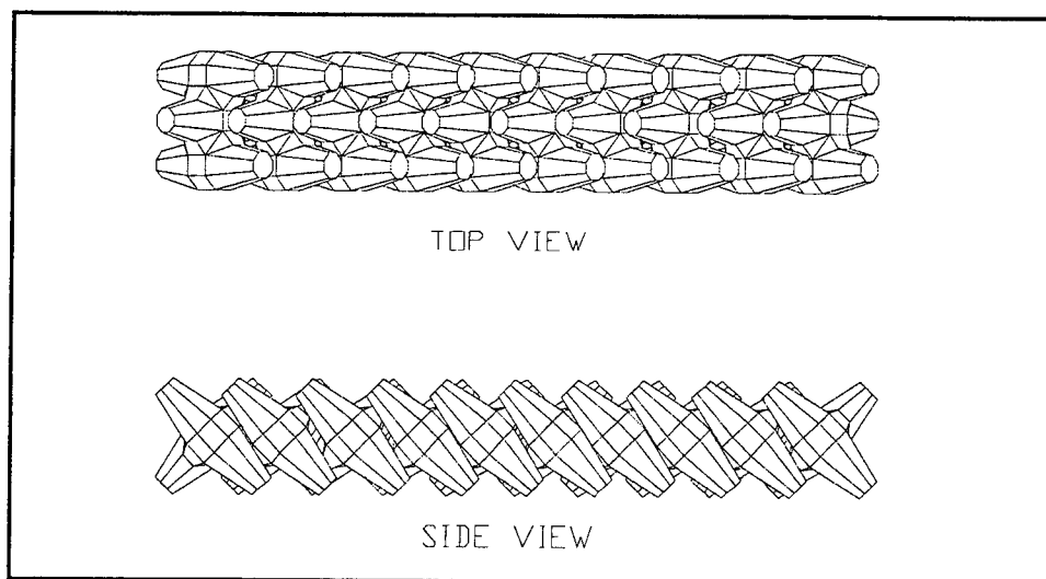
Figure 4. Efficient storage pattern for core-loc in casting yard
