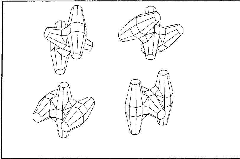
Figure 1. Four views of core-loc
