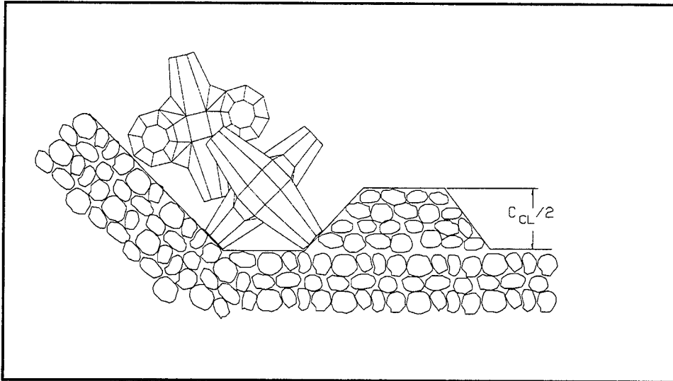
Figure 7. Possible method for toe and second course placement
