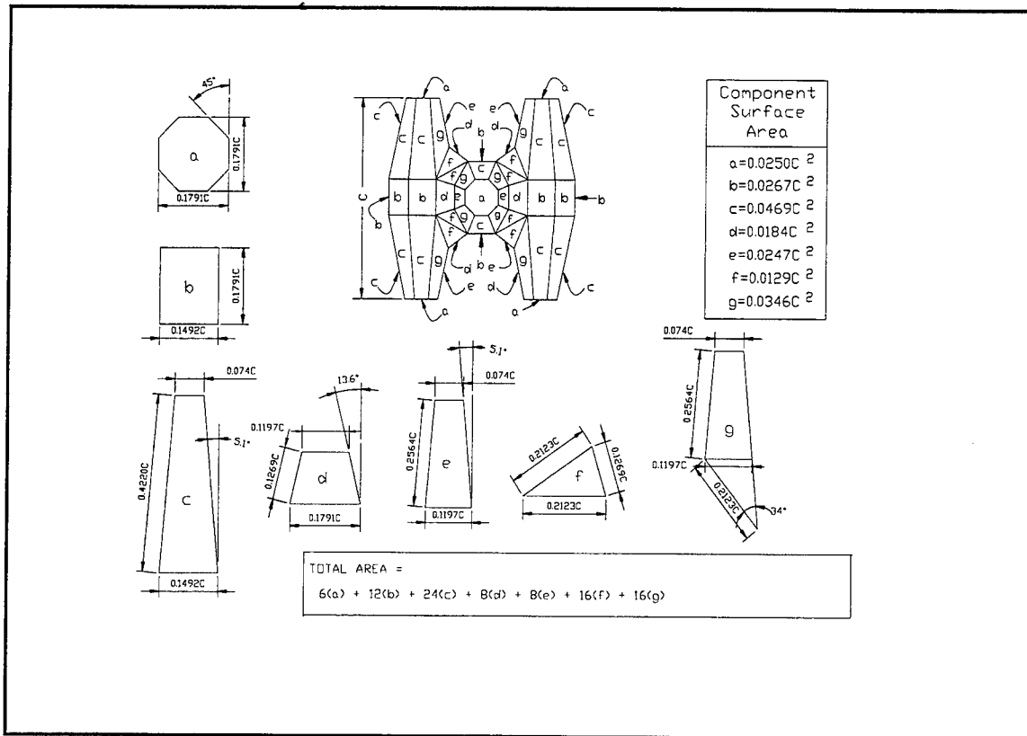
Figure 3. Nondimensional schematic of core-loc surface area
