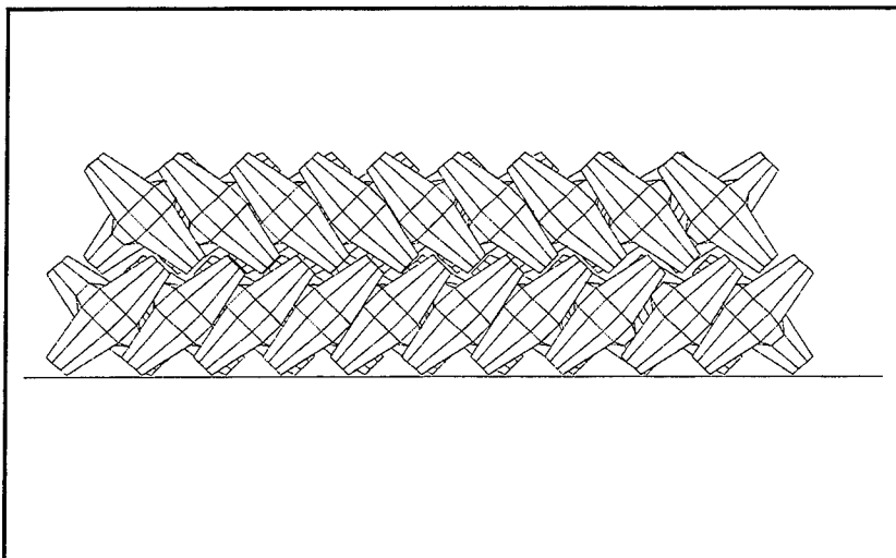
Figure 5. Core-loc stacked two courses in height
