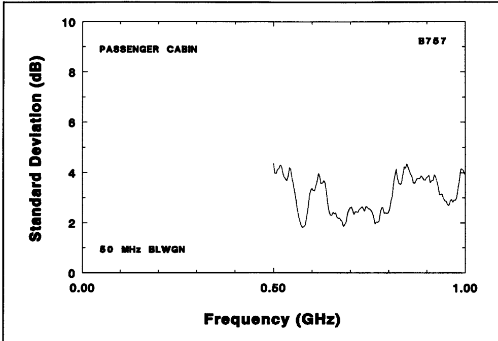
FIGURE 14. B757 PASSENGER CABIN LOW FREQUENCY STANDARD DEVIATION DATA
