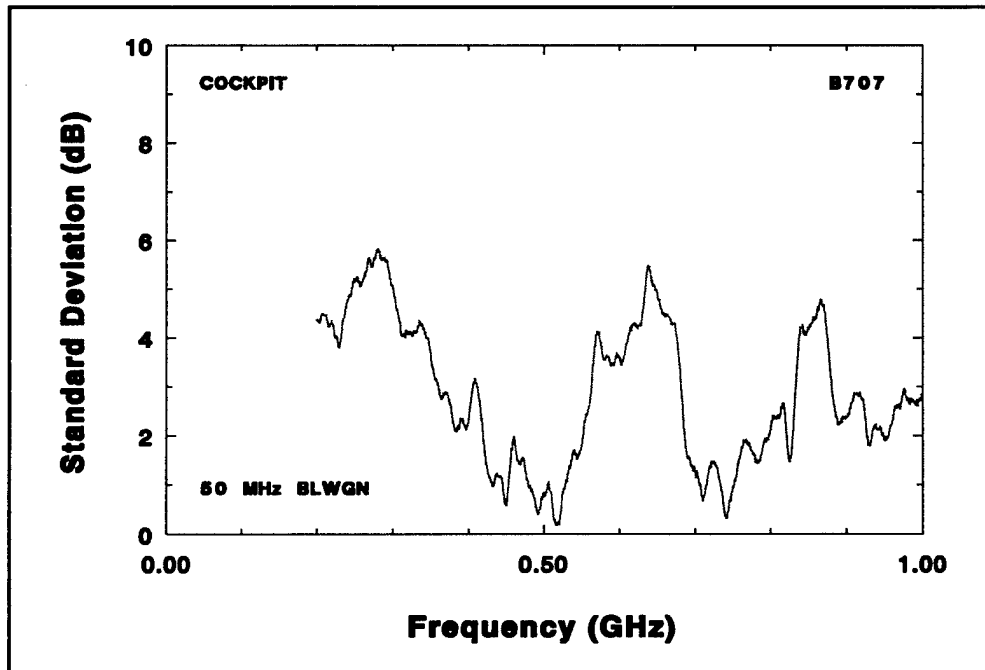
FIGURE 11. B707 COCKPIT LOW FREQUENCY STANDARD DEVIATION DATA
