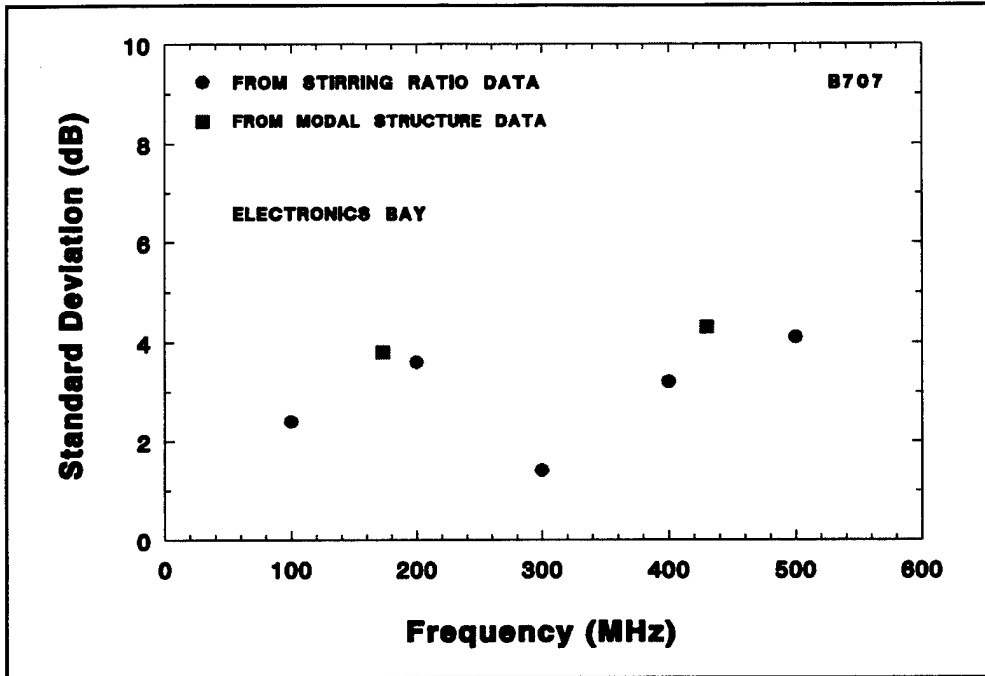
FIGURE 7. B707 ELECTRONICS BAY LOW FREQUENCY BOUNDARY CONDITION EFFECTS
