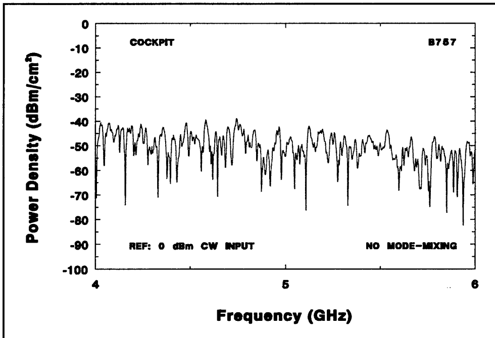
FIGURE 4. B757 COCKPIT HIGH FREQUENCY MODAL STRUCTURE DATA
