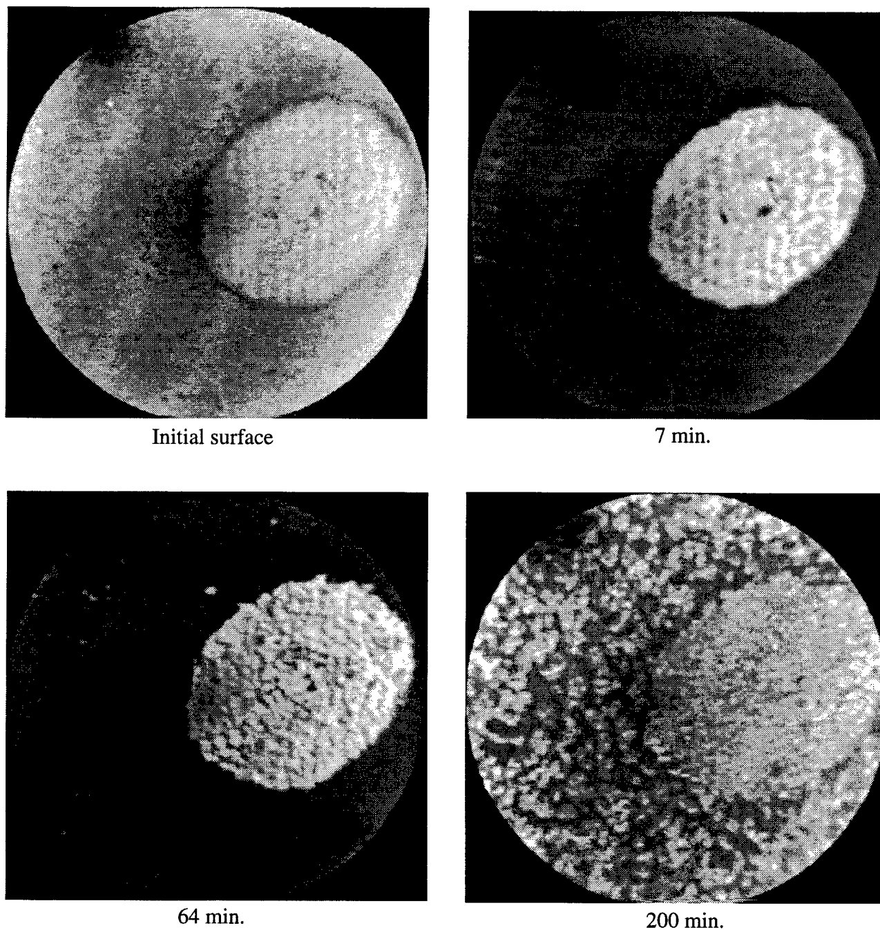
Figure 4. LEEM images of GaN during growth with seeded beam. Time elapsed during deposition is indicated in minutes. Electron energy is 7.0 eV. Field of view is 4.8 \mu\text{m} .
