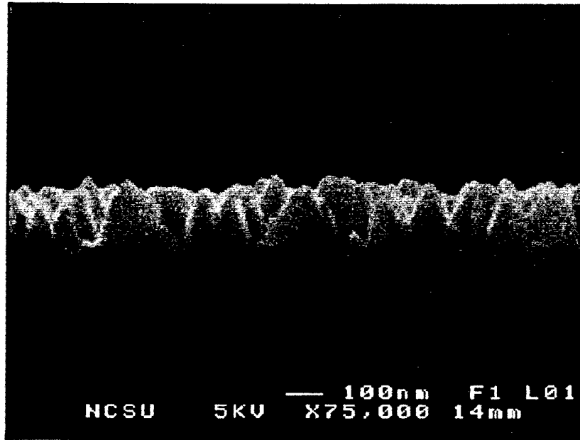
Figure 3. GaN grown 600°C, 60 sccm NH 3 and 10°C TEG.
