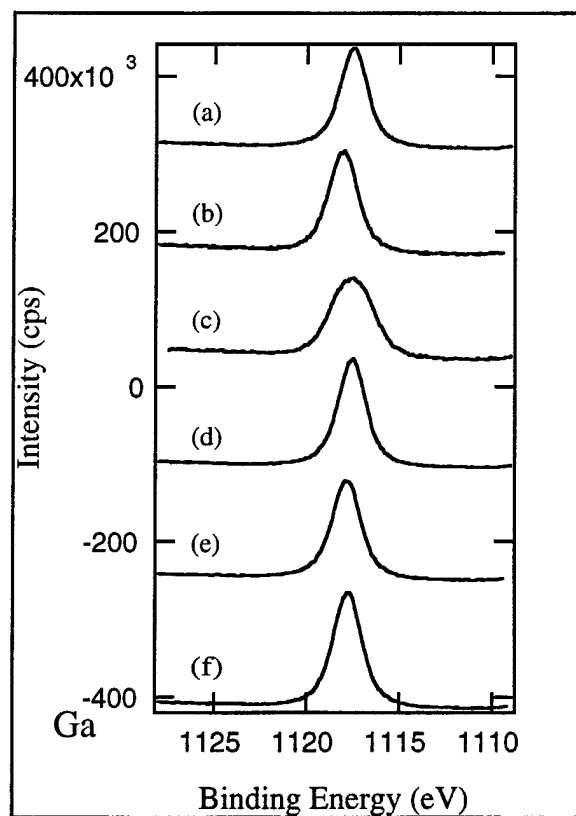
Figure 1. From top to bottom (a-f): a) GaN substrate without cleaning, b) ammonia treatment at 850°C for 15 mins., c) heating at 850°C for 15 mins., d) GaN substrate without cleaning, e) heating at 800°C for 15 mins., f) ammonia treatment at 800°C for 15 mins. Note: a-c, d-f are taken from the same substrate.
