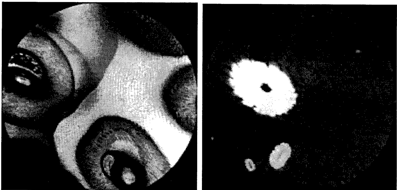
Figure 3. LEEM images showing the heterogeneity of the 6H-SiC(0001) surface in two different crystals. Electron energy is 33.6 eV (a) and 11.0 eV (b). Field of view is 20.6 \mu\text{m} .
