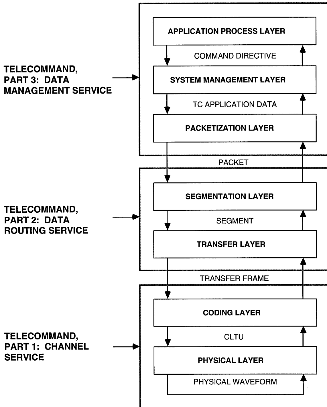
Figure 2-1: Telecommand System
