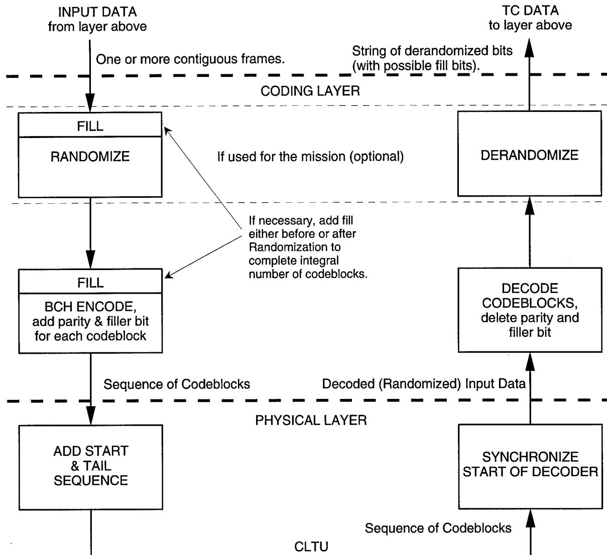
Figure B-2: Sequence of Functions
