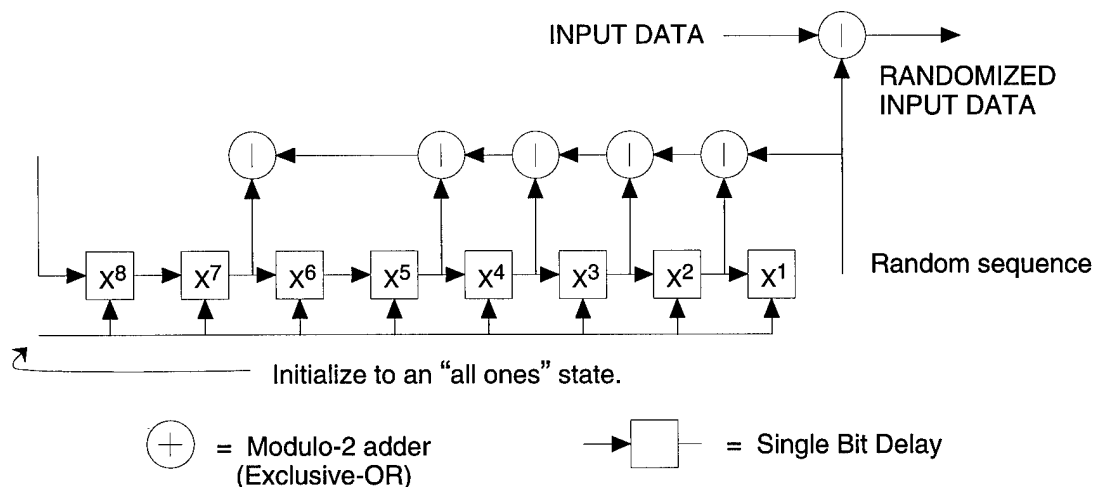
Figure 3-3: Bit Transition Generator Logic Diagram
