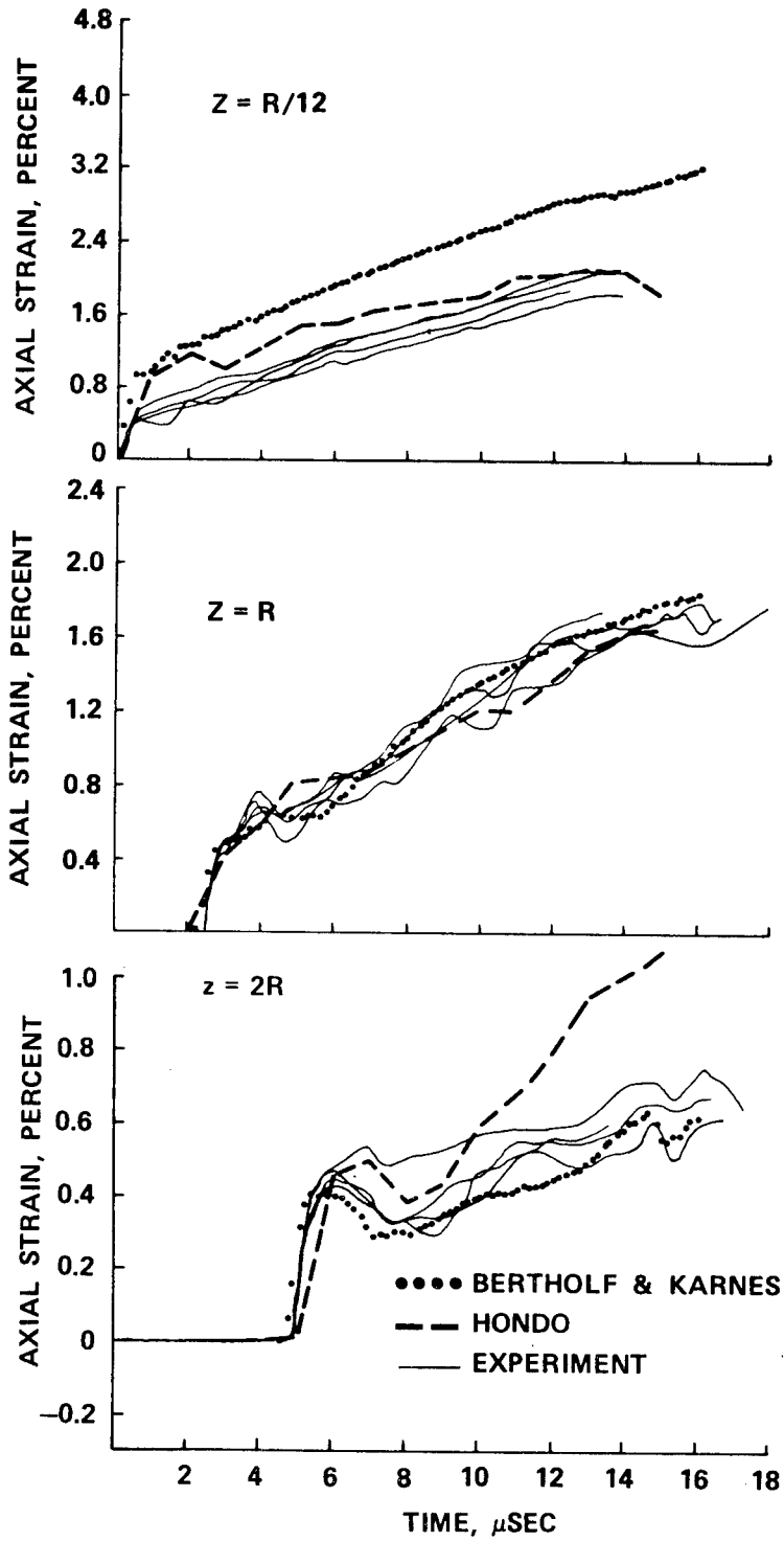
FIGURE 7. Elastic-Plastic Rod With Transverse Inertia, Axial Strain at Free Surface Versus Axial Distance.
