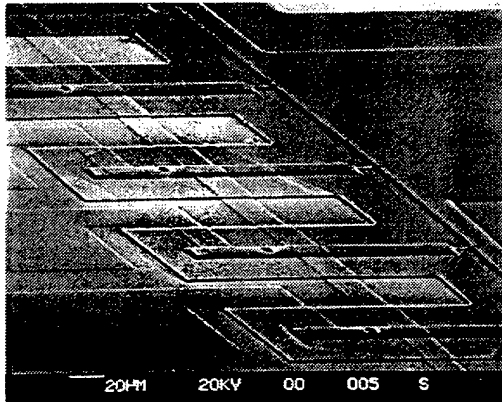
a. An array of micro injector
