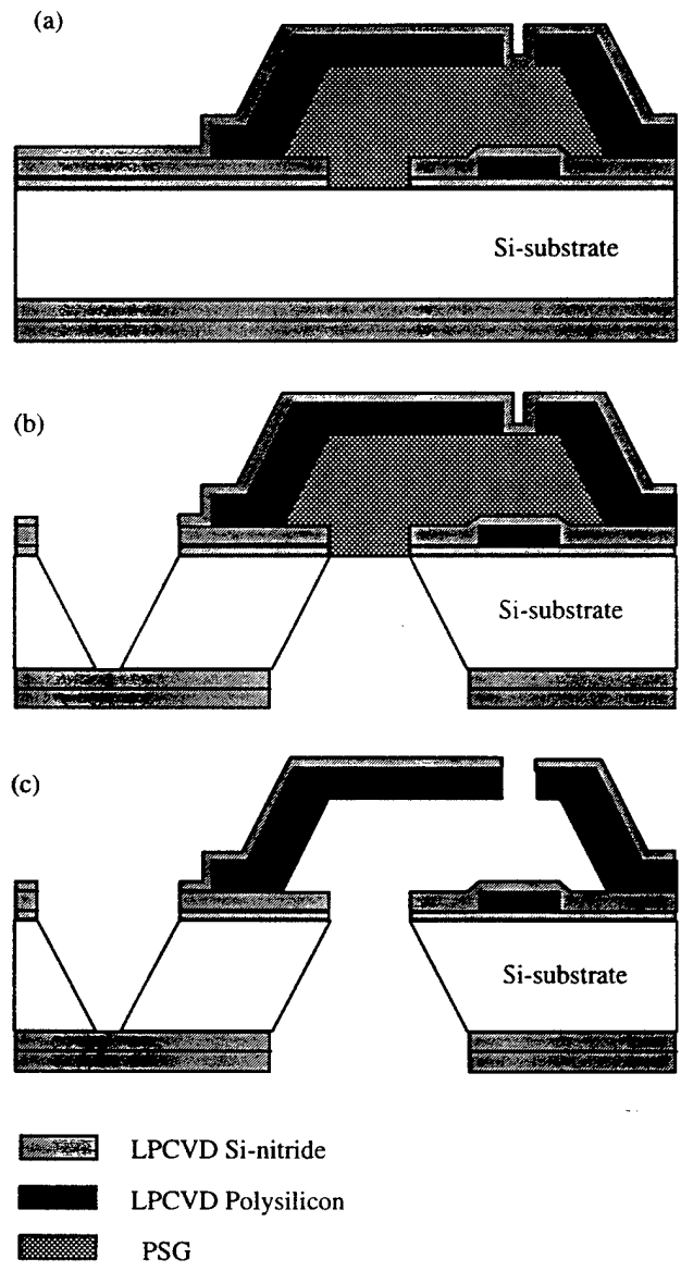
Fig. 5 Fabrication Process
