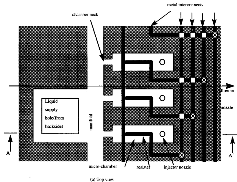
Fig. 3 Design of Micro Injectors.
