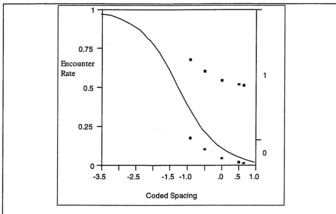
Figure 11. Logistic Regression Prediction Curve.
