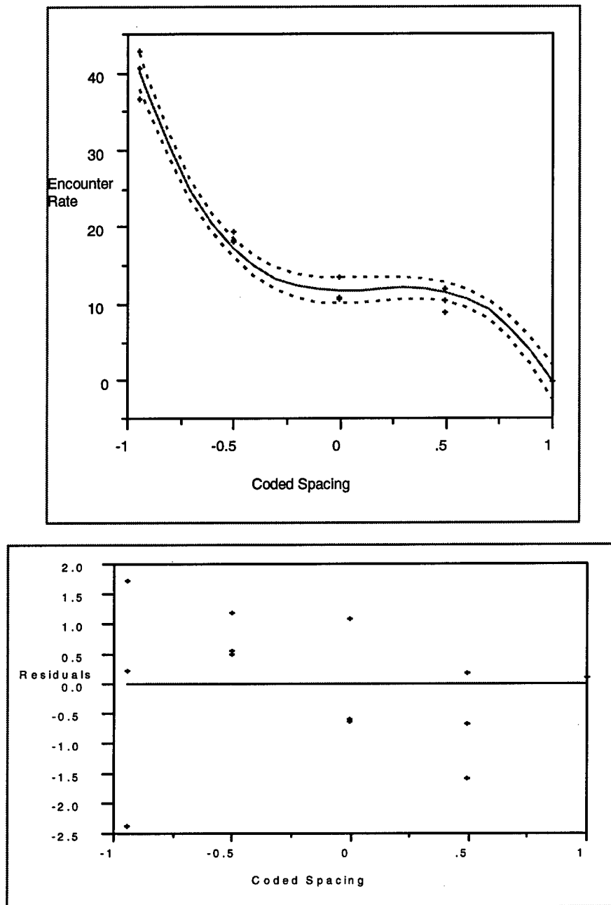
Figure 17. Reduced Third Order Curve with Confidence Interval and Residuals.
