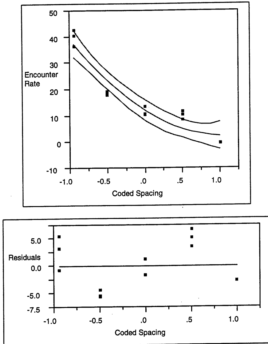
Figure 14 . Second Order Regression with Confidence Interval and Residuals.
