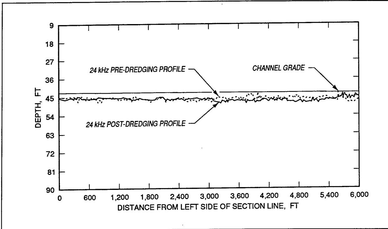
Figure 11. Pre- and post-dredging low-frequency acoustic data along the same profile line shown in Figures 12 and 13
