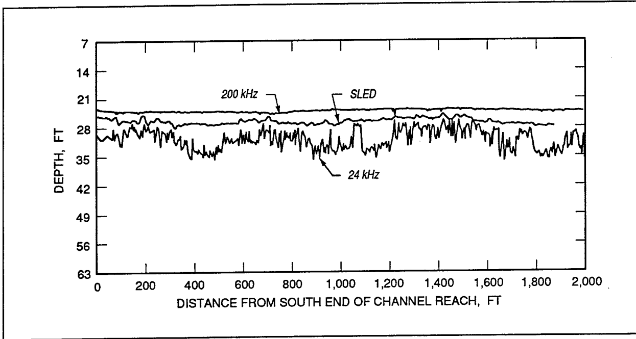
Figure 17. Gulfport Channel sounding comparison (see Figure 16, line 3)
