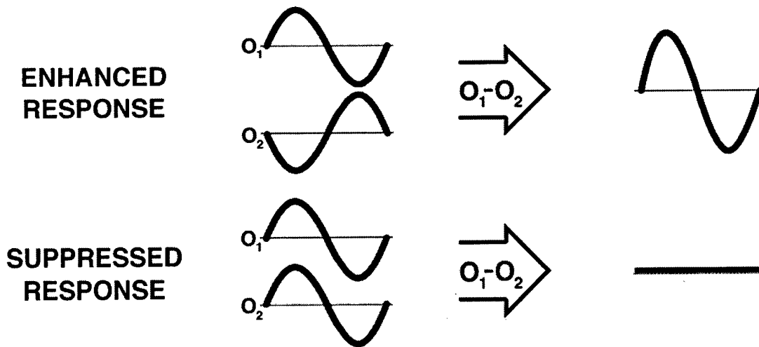
Figure 4. Illustration of the two possible mechanisms for self-regulating the steady-state visual evoked response, recorded with bipolar techniques.
