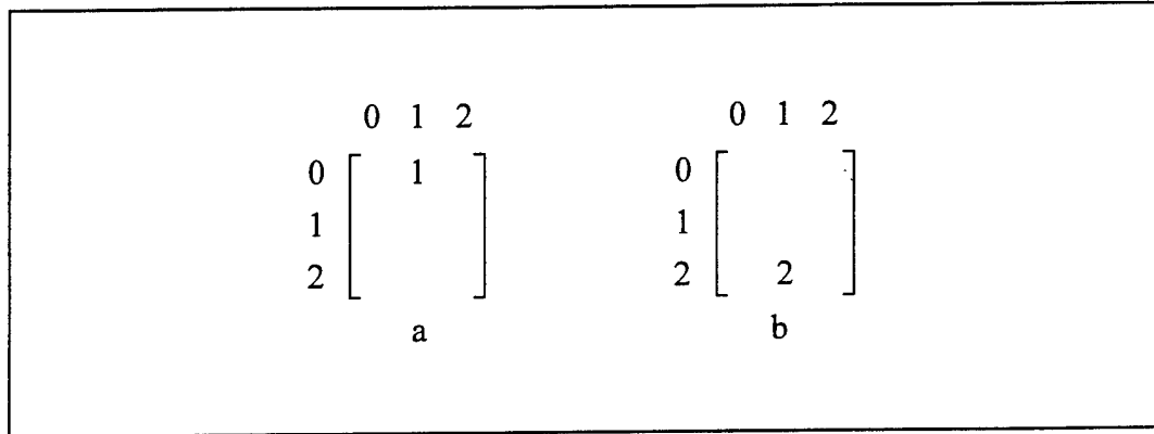
Figure 10. Filling the 0^\circ GLCM of the target image. Panel (a) is the result of counting the number of (0→1) grey levels separated by a distance of 1 pixel in the horizontal direction (=1), while panel (b) is populated from the number of (2→1) occurrences (=2). The completed matrix is given in equation (14).
