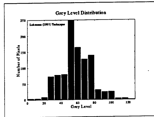
(h) GLCM
