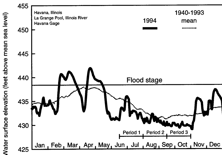
Figure 6.1. Daily water surface elevation from Havana Gage for La Grange Pool, Illinois River, during 1994 and mean elevation since 1940. The U.S. Army Corps of Engineers discharge data were obtained from the Environmental Management Technical Center (Wlosinski et al. 1995).
