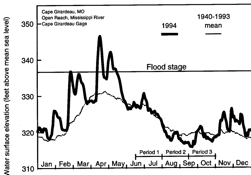
Figure 5.1. Daily water surface elevation from Cape Girardeau Gage for the Upper Mississippi River Open Reach, during 1994 and mean elevation since 1940. The U.S. Army Corps of Engineers discharge data were obtained from the Environmental Management Technical Center (Wlosinski et al. 1995).
