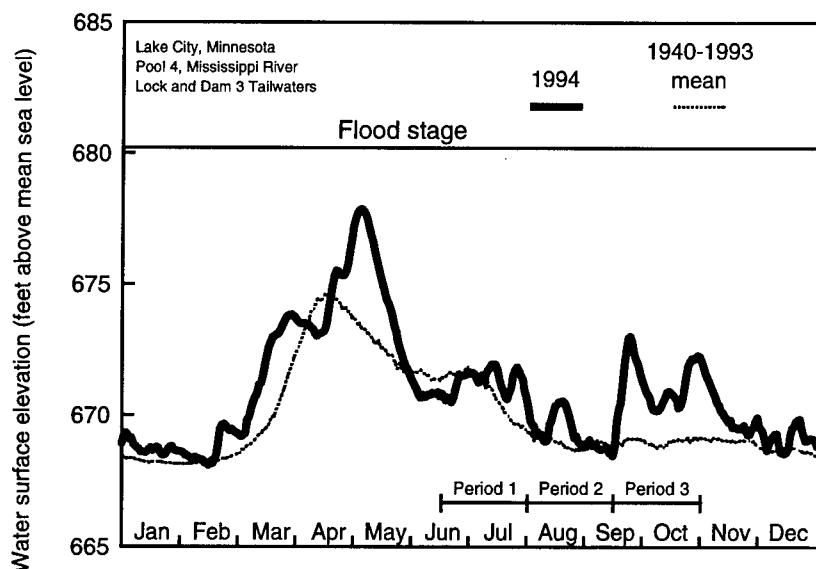
Figure 1.1. Daily water surface elevation from Lock and Dam 3 for Pool 4, Upper Mississippi River, during 1994 and mean elevation since 1940. The U.S. Army Corps of Engineers discharge data were obtained from the Environmental Management Technical Center (Wlosinski et al. 1995).
