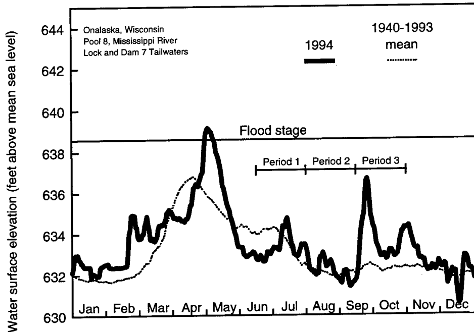
Figure 2.1. Daily water surface elevation from Lock and Dam 7 for Pool 8, Upper Mississippi River, during 1994 and mean elevation since 1940. The U.S. Army Corps of Engineers discharge data were obtained from the Environmental Management Technical Center (Wlosinski et al. 1995).
