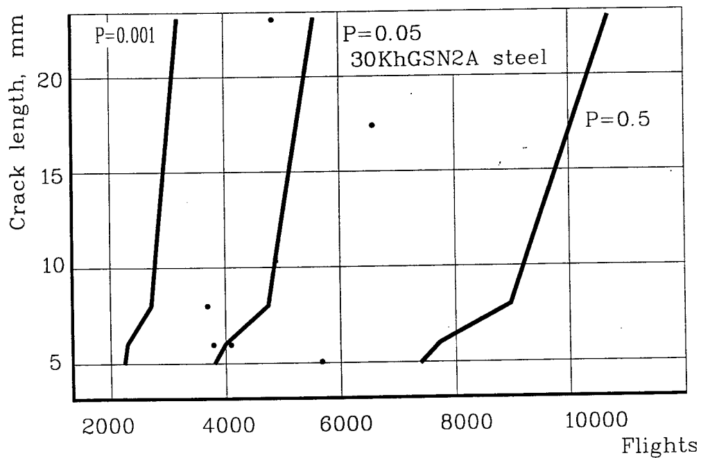
Figure 8 Corrosion-fatigue damage growth in landing gear cylinder
