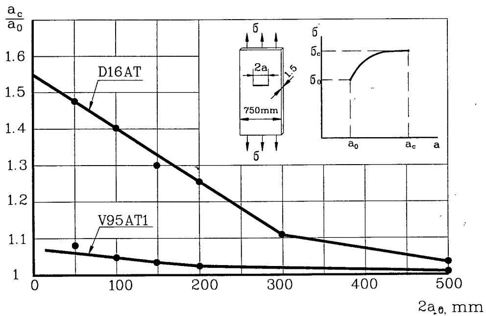
Figure 2 Stable crack growth from sheet cutouts
