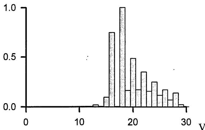
Fig.5.9. Overtone laser spectrum calculated taking into account the atmospheric water vapor absorption: \text{CO}:\text{N}_2 = 1:9 ; N = 0.3 \text{ Amagat} ; T_0 = 105 \text{ K} ; Q_{in} = 364 \text{ J/l Amagat} .
