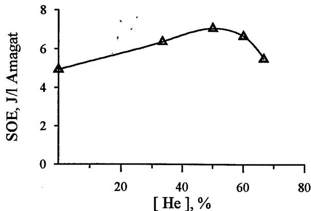
Fig.3.28. Specific FO CO laser output energy (SOE) versus He content 100x/(1+9+x) in gas mixture CO:N 2 :He=1:9:x. N = 0.15 Amagat. Other parameters correspond to data from Table 3.1.
