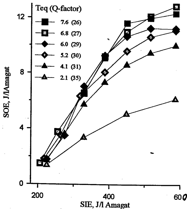
Fig.3.8. Specific FO CO laser output energy (SOE) versus specific EBCD input energy (SIE) for various equivalent output coupling T_{eq} (Q-factor Q_{2L} ) of the laser resonator. N=0.15 Amagat. Other parameters correspond to data from Table 3.1.
