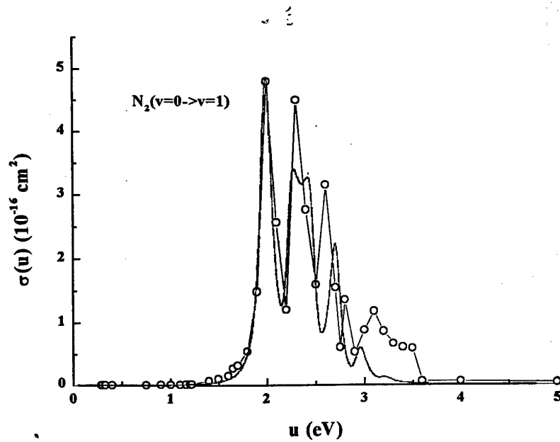
Fig.2.5. Comparison of experimental (Schulz, 1979) and calculated (Aleksandrov et al, 1979) cross sections for excitation of N_2 molecule by electron impact: v=0 \rightarrow v=1
