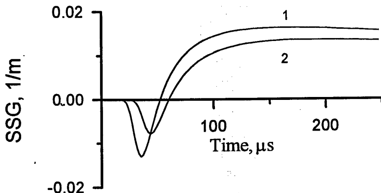
Fig.5.10. The absorption/gain coefficients vs time for transitions P(16, 12), P(18, 13): \text{CO:N}_2 = 1:9 ; N = 0.3 \text{ Amagat} ; T_0 = 105 \text{ K} ; Q_{in} = 45 \text{ J/l Amagat}
