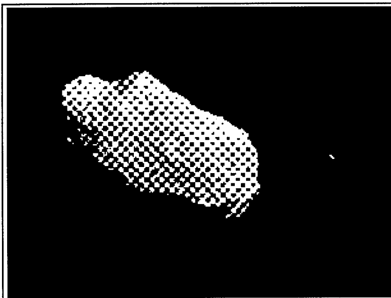
Figure 2-3. Asteroid Ida (56 Km Long) and its Moon (1 km Diameter)
