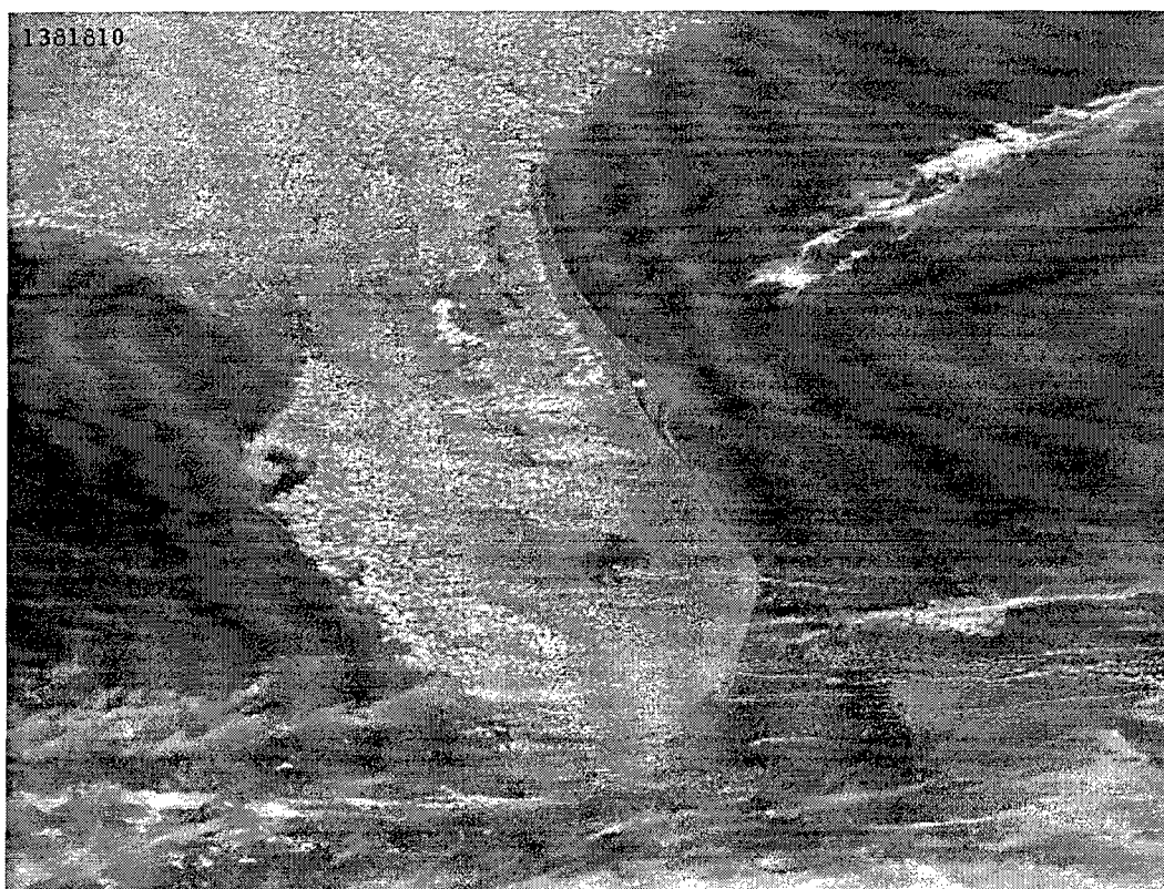
Fig. 5. GOES 1 km visible image for 1810 UTC 17 May 1996. The Atlantic sea breeze is apparent along the east coast of Florida.
