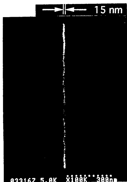
FIG. 1. SEM image of a high aspect ratio isolated Ni bar that is 1\ \mu\text{m} long and 15 nm wide.
