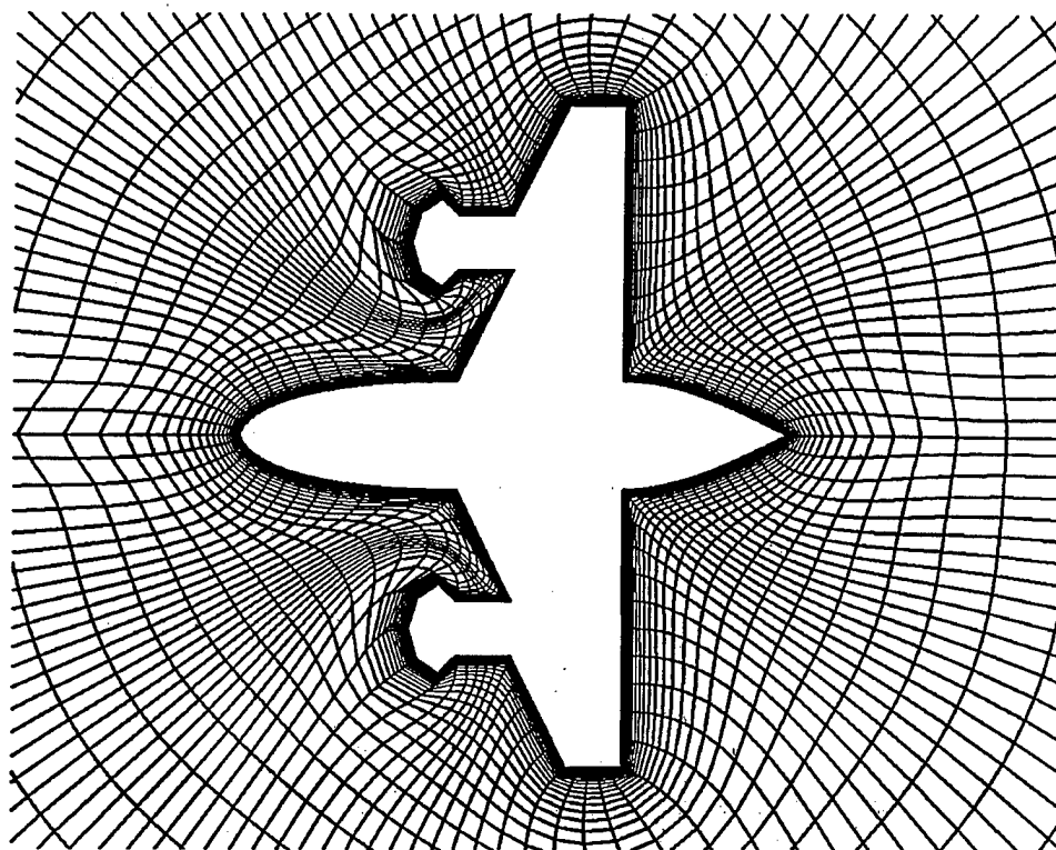
Figure 4.12 Side view of entire geometry
