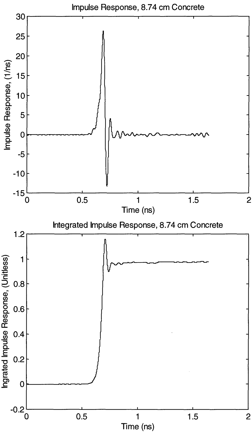
Figure 8.5. The impulse response (top) and its integral (bottom) of 8.74cm concrete.
