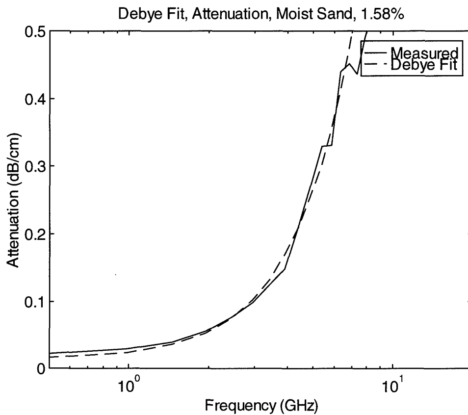
Figure 12.5. Attenuation constant of moist sand 1.58%, measured and Debye model fit, including conductivity.
