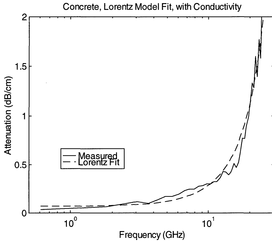
Figure 14.4. Comparison of concrete attenuation to Lorentz fit, with conductivity.
