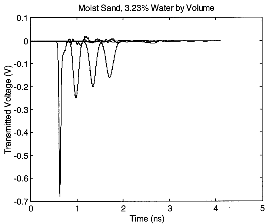
Figure 11.2. Impulse propagation through moist sand (3.23%), lengths 0, 14.1, 28.2 and 42.2 cm.
