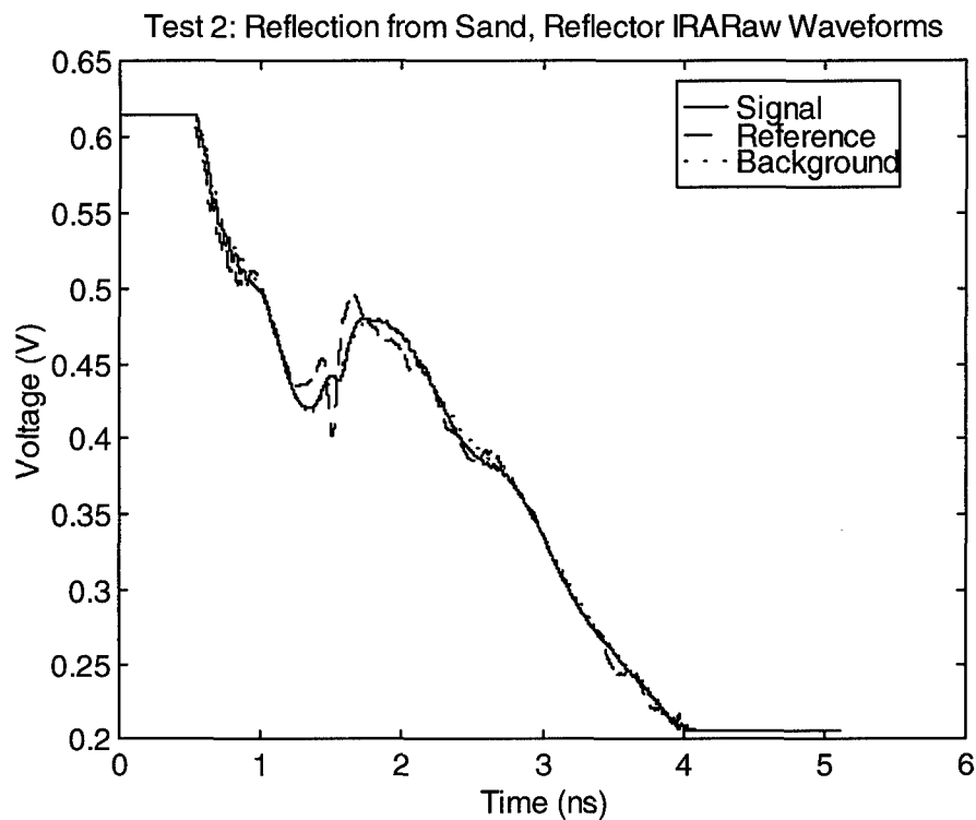
Figure 15.7. Raw data for reflection from sand with a reflector IRA.
