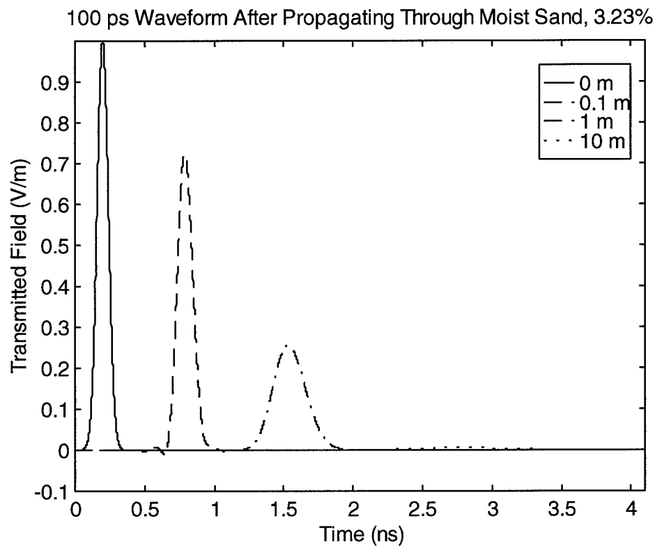
Figure 13.2. The propagated field of the 100 ps pulse at 0, 0.1, 1, and 10 meters, 1.58% top and 3.23% bottom. (Starting times shifted for clarity.)
