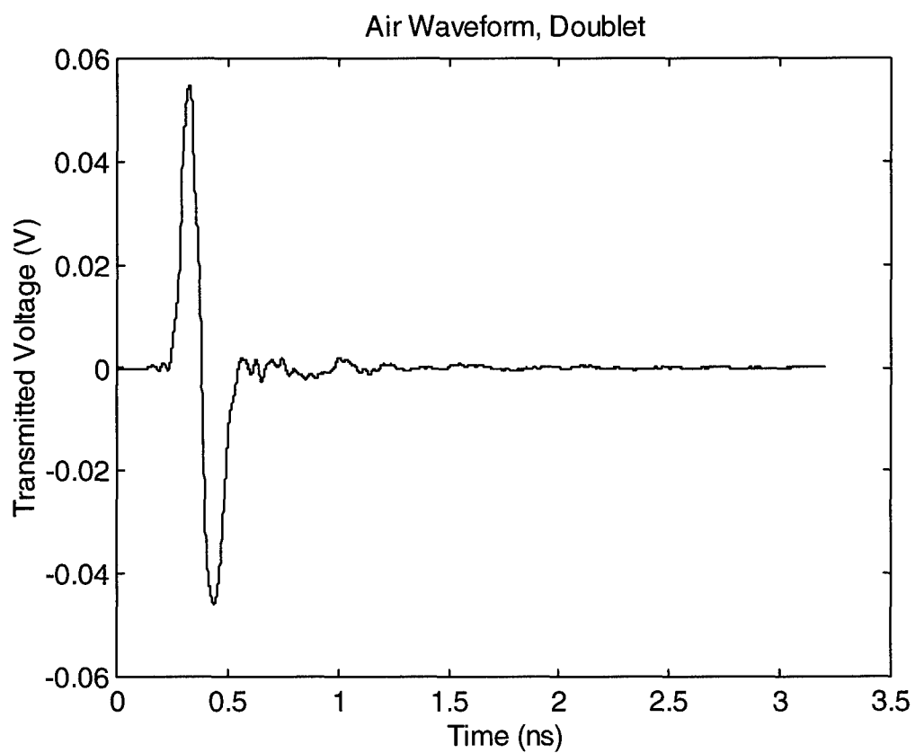
Figure 5.3. Air waveform for the doublet waveshape.
