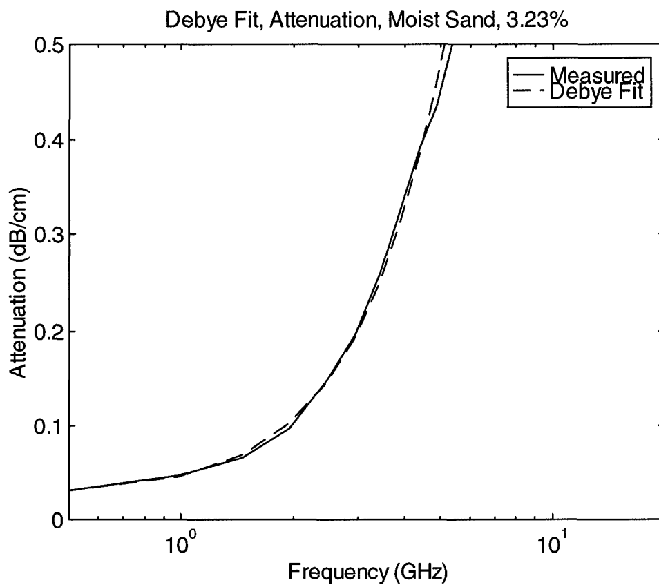
Figure 12.11. Attenuation constant of moist sand, 3.23%, measured and Debye model fit, including conductivity.
