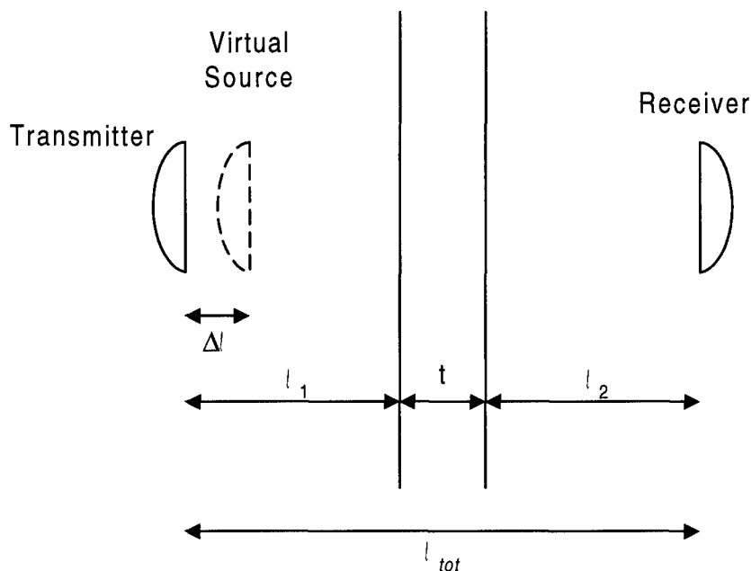
Figure B.1. Two antennas on either side of a dielectric slab, with the virtual source.
