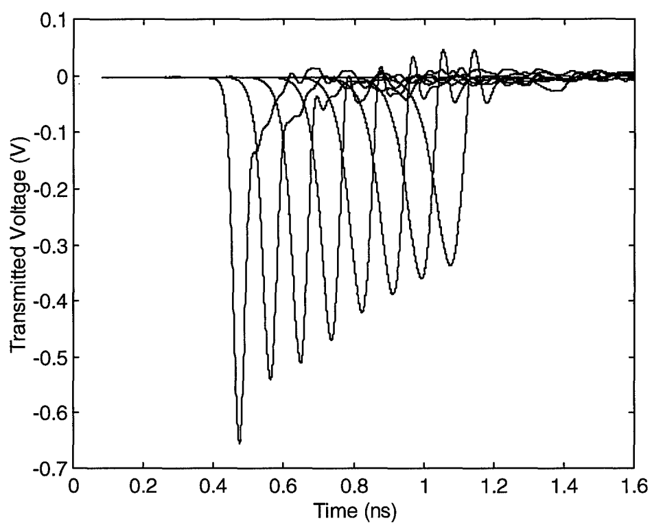
Figure 8.1. Propagation through concrete, with thicknesses of 0, 2.87, 5.77, 8.66, 11.53, 14.45, 17.34, and 20.27 cm.
