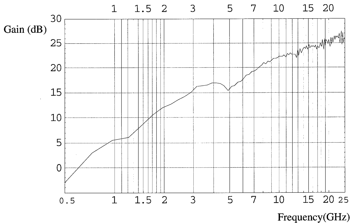
Figure A.2. Gain of the nine-inch lens IRA.
