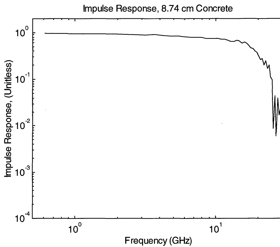
Figure 8.4. The impulse response of 8.74 cm of concrete.
