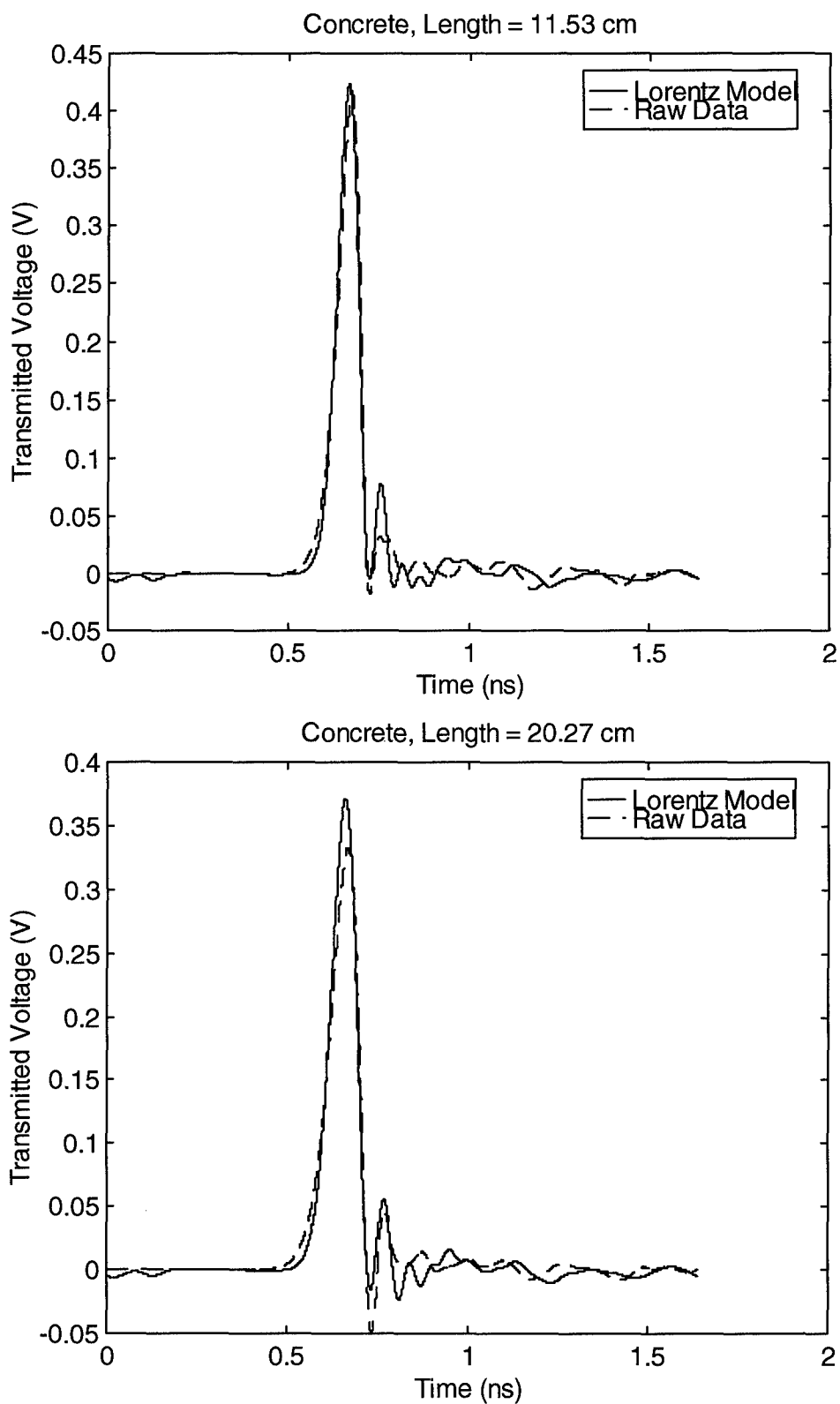
Figure 8.8. Propagation of the impulse through 11.53 cm and 20.27 cm of concrete, raw data and prediction with Lorentz model convolved with the air waveform.
