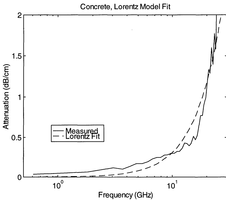
Figure 8.7. Attenuation constant of concrete, measured and Lorentz model fit.
