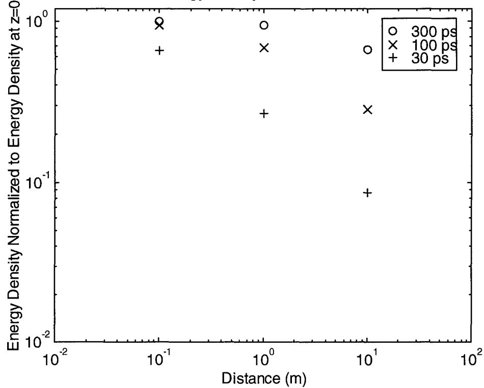
Figure 10.7. Normalized Energy density as a function of input FWHM and propagation distance.
