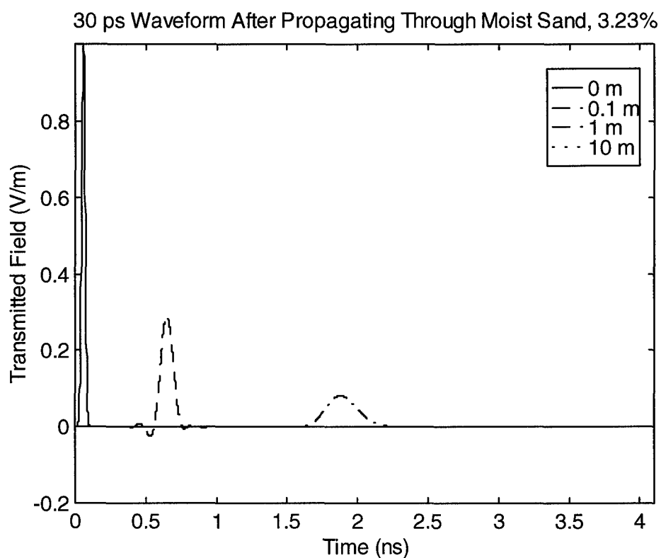
Figure 13.1. The propagated field of the 30 ps pulse at 0, 0.1, 1, and 10 meters, 1.58% top and 3.23% bottom. Note that the 10-meter pulse on the bottom is invisible. (Starting times shifted for clarity.)
