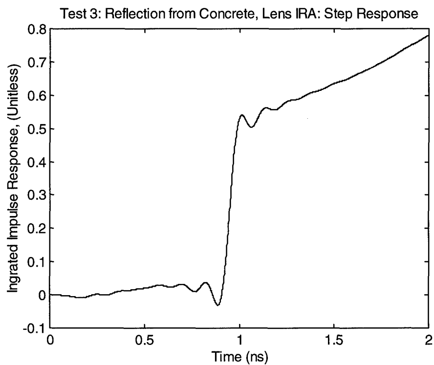
Figure 15.14. Step response for concrete reflection.
