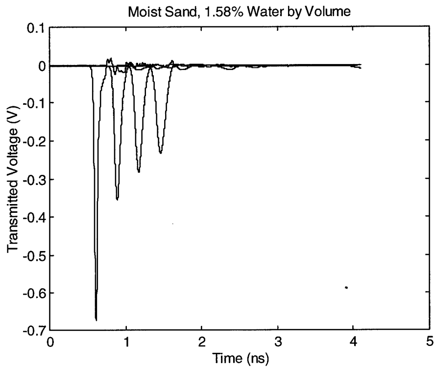
Figure 11.1. Impulse propagation through moist sand (1.58%), lengths 0, 13.5, 27.0 and 40.4 cm.
