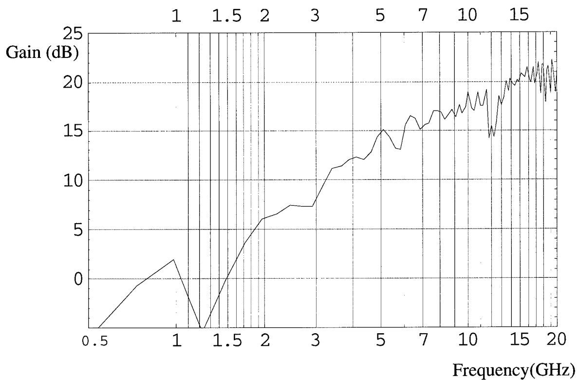
Figure A.1. Gain of the nine-inch reflector IRA.
