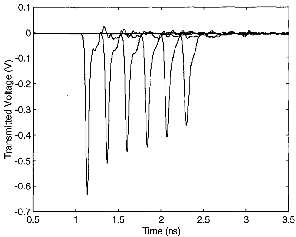
Figure 4.1. Propagation through dry sand, with thicknesses of 0, 11.9, 23.86, 35.79, 47.72, and 59.65 cm.
