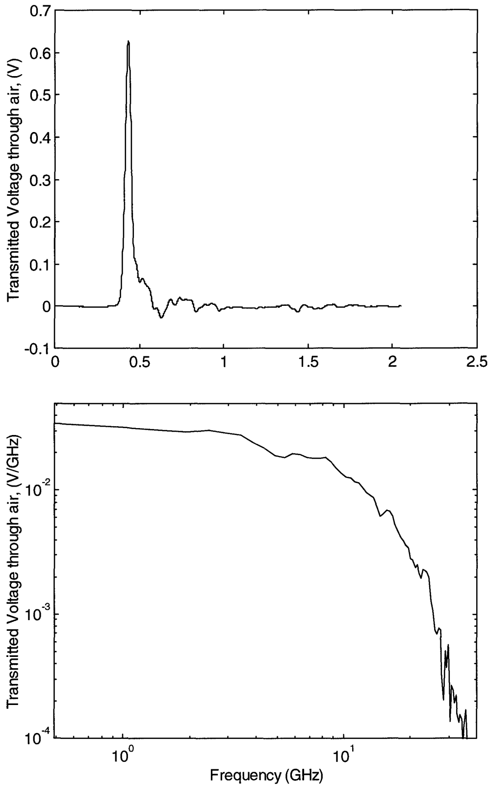
Figure 4.2. Air waveform for the dry sand measurements, time domain (top) and frequency domain (bottom).
