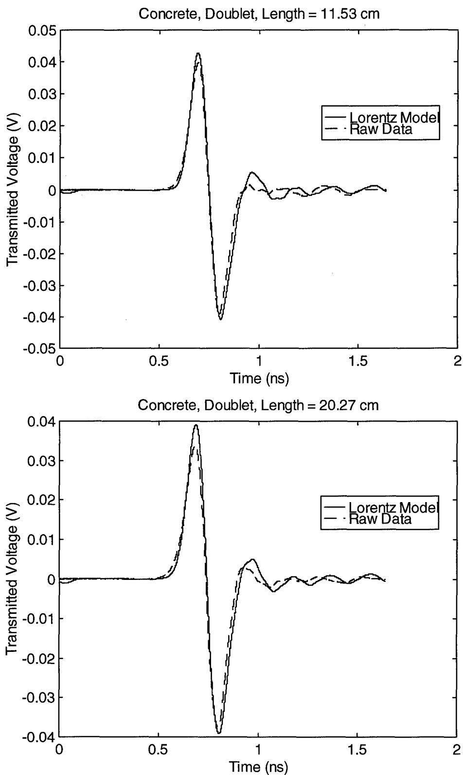
Figure 9.2. Propagation of the doublet through 11.53 cm and 20.27 cm of concrete, raw data and prediction with Lorentz model.
