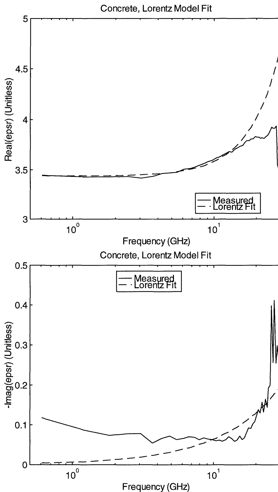
Figure 8.6. Measured dielectric constant of concrete, and the Lorentz model fit, real and imaginary parts.
