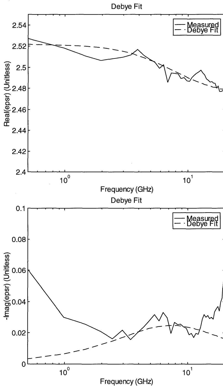
Figure 4.6. Measured dielectric constant of dry sand, and the Debye fit, real and imaginary parts.
