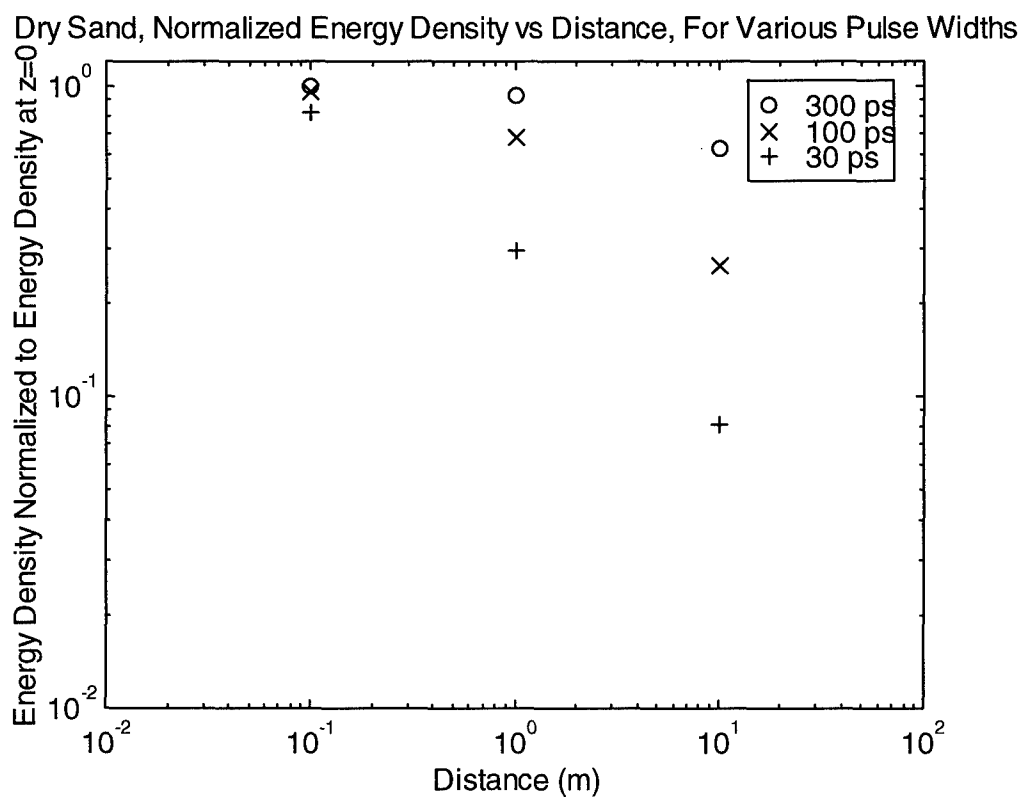
Figure 6.8. Normalized Energy density as a function of input FWHM and propagation distance.
