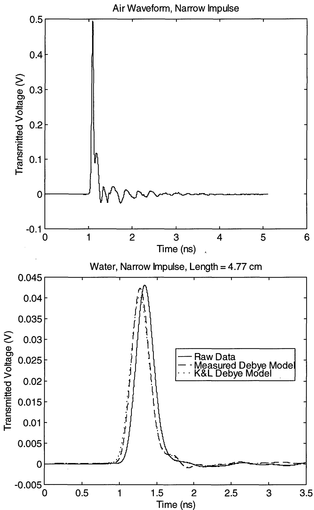
Figure 3.9. Narrow impulse air waveform, and transmission through 4.77 cm water.
