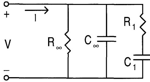
Figure 2.2. Circuit model of the Debye Model, with conductivity included.
