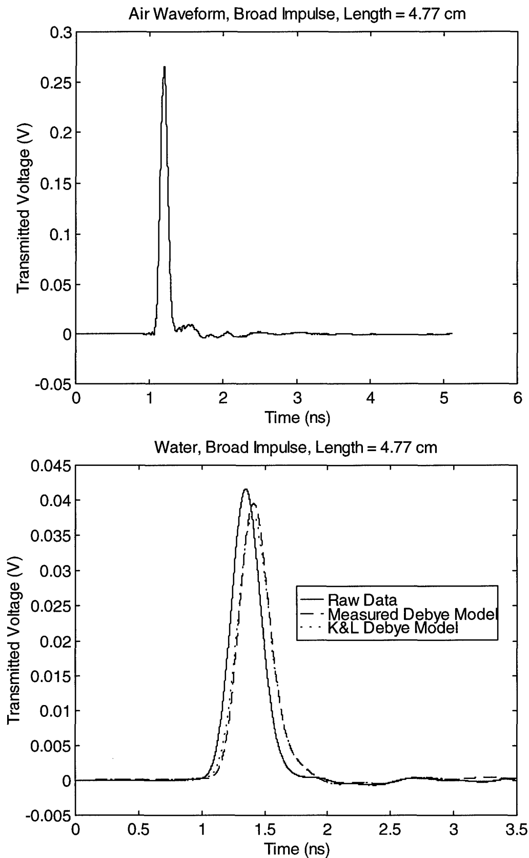
Figure 3.3. Broad impulse air waveform, and transmission through 4.77 cm water.
