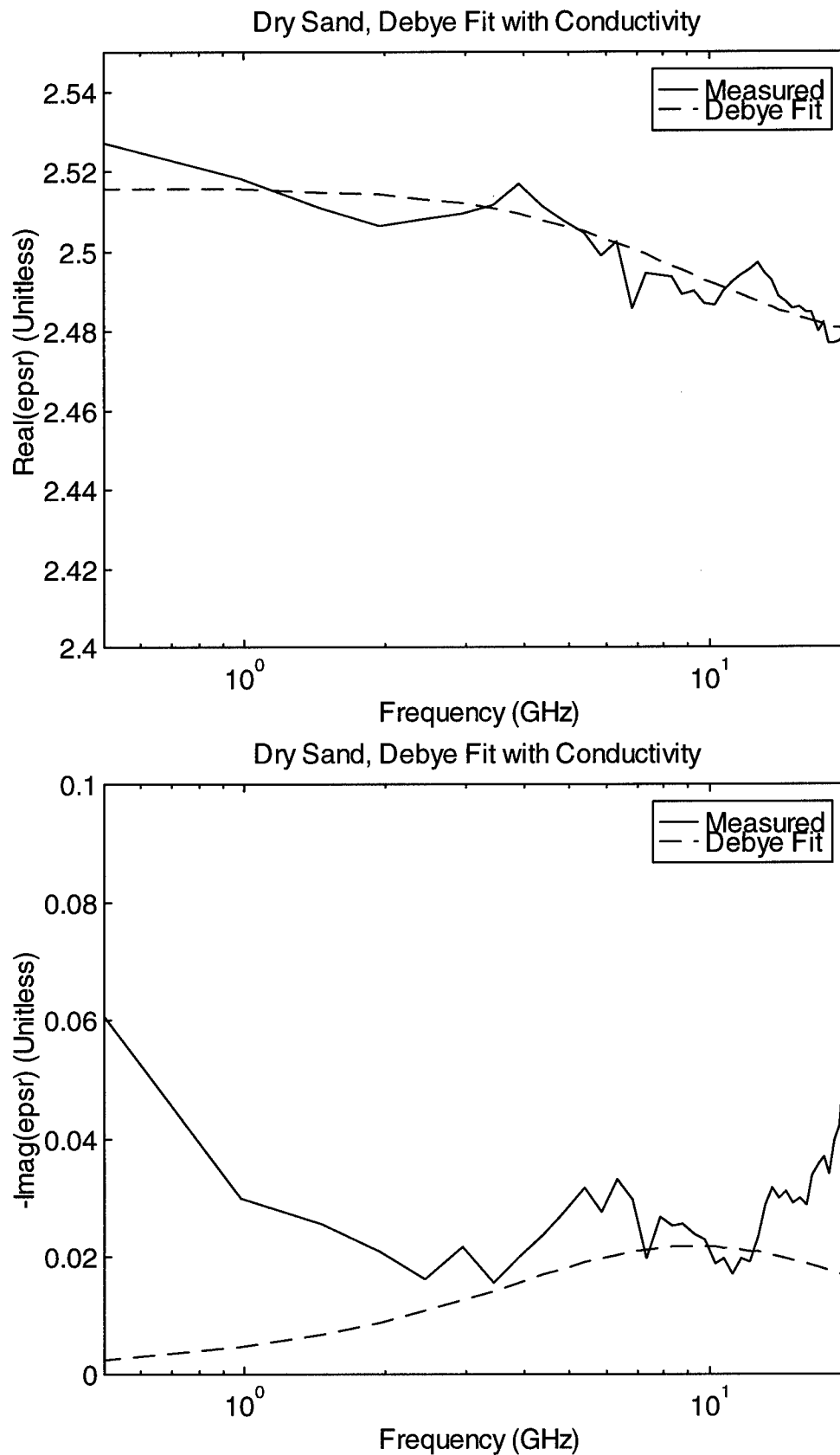
Figure 14.1. Comparison of dry sand dielectric constant to Debye fit, with conductivity.
