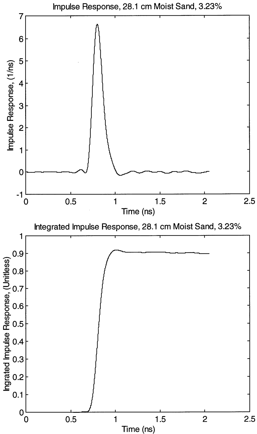
Figure 12.9. The impulse response (top) and its integral (bottom) of 28.1 cm moist sand, 3.23%.
