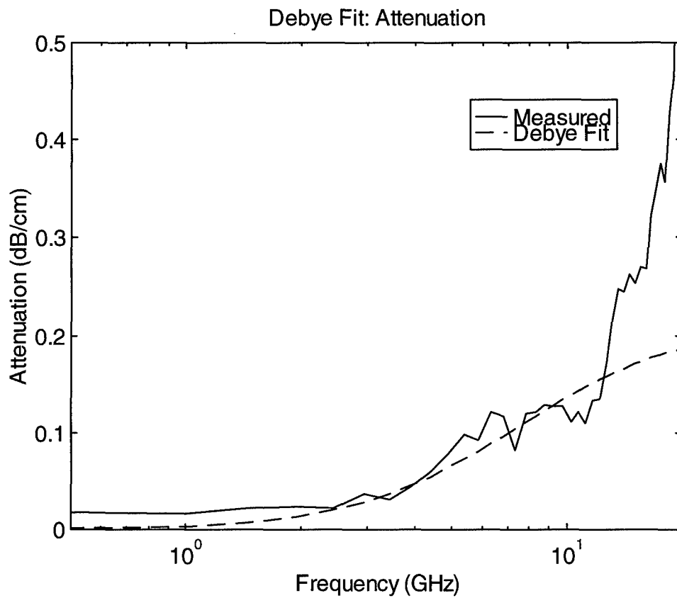
Figure 4.7. Attenuation constant of dry sand, measured and Debye fit.
