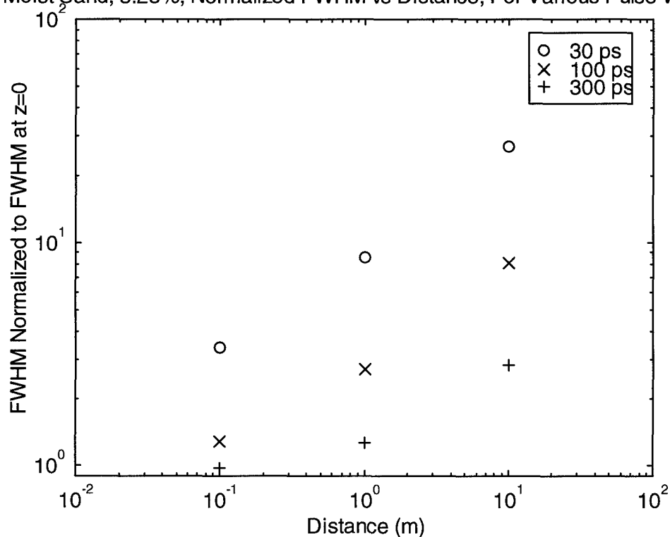
Figure 13.5. Normalized FWHM as a function of input FWHM and propagation distance, 1.58% top and 3.23% bottom.
