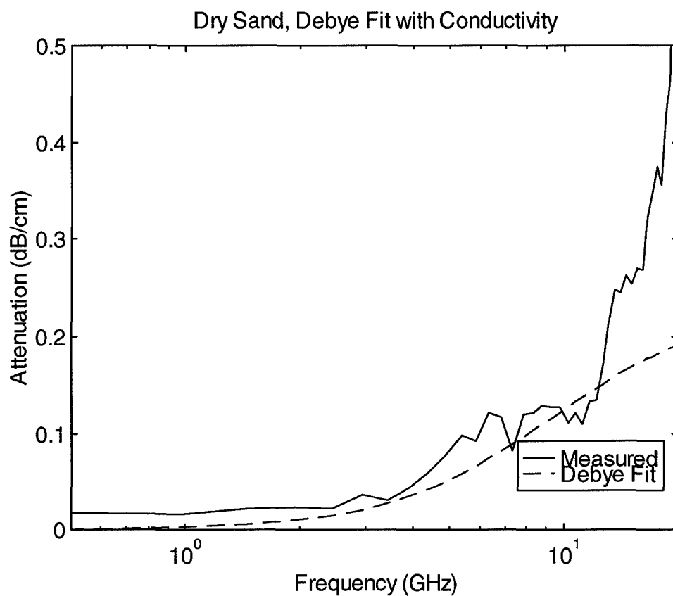
Figure 14.2. Comparison of dry sand attenuation to Debye fit, with conductivity.
