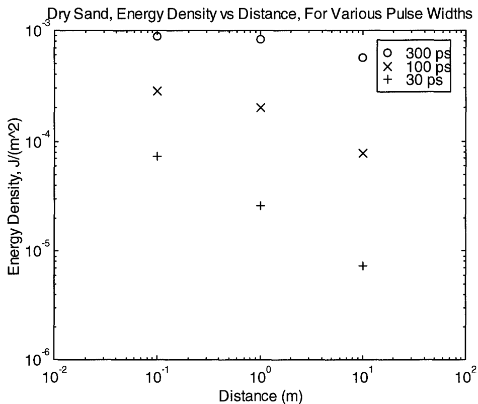
Figure 6.7. Energy density as a function of input FWHM and propagation distance.
