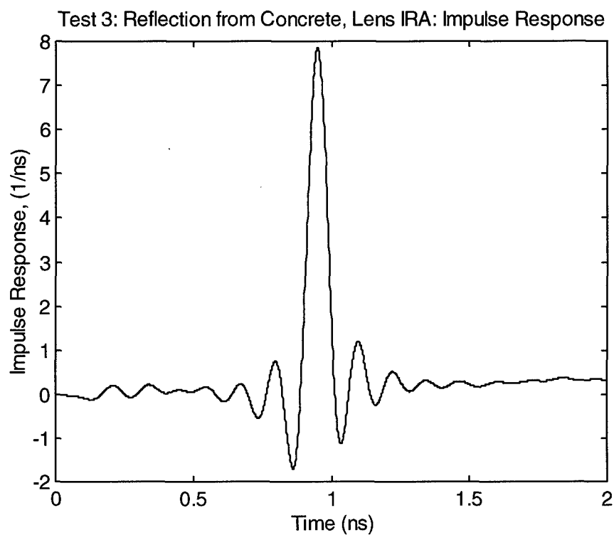
Figure 15.13. Impulse response for concrete reflection.
