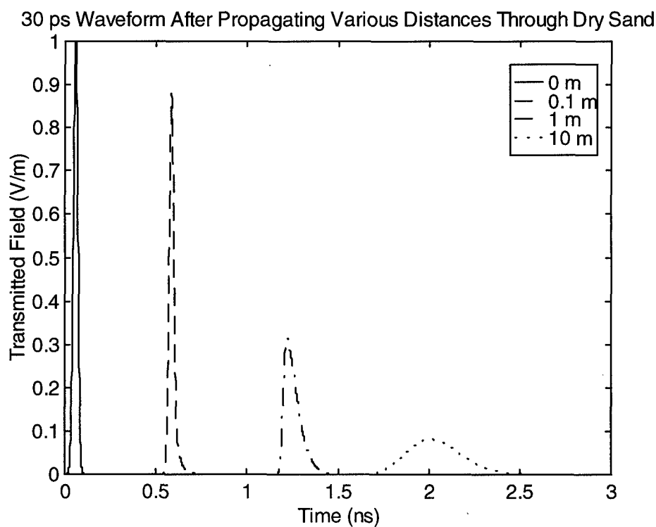
Figure 6.2. The propagated field of the 30 ps pulse at 0, 0.1, 1, and 10 meters. (Starting times shifted for clarity.)
