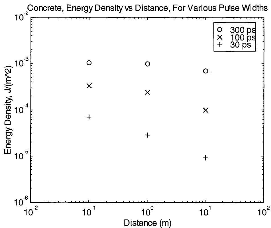
Figure 10.6. Energy density as a function of input FWHM and propagation distance.
