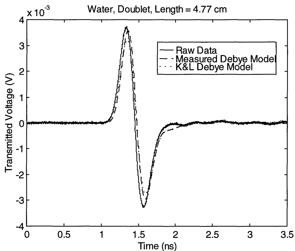
Figure 3.5. Doublet air waveform, and transmission through 4.77 cm water.
