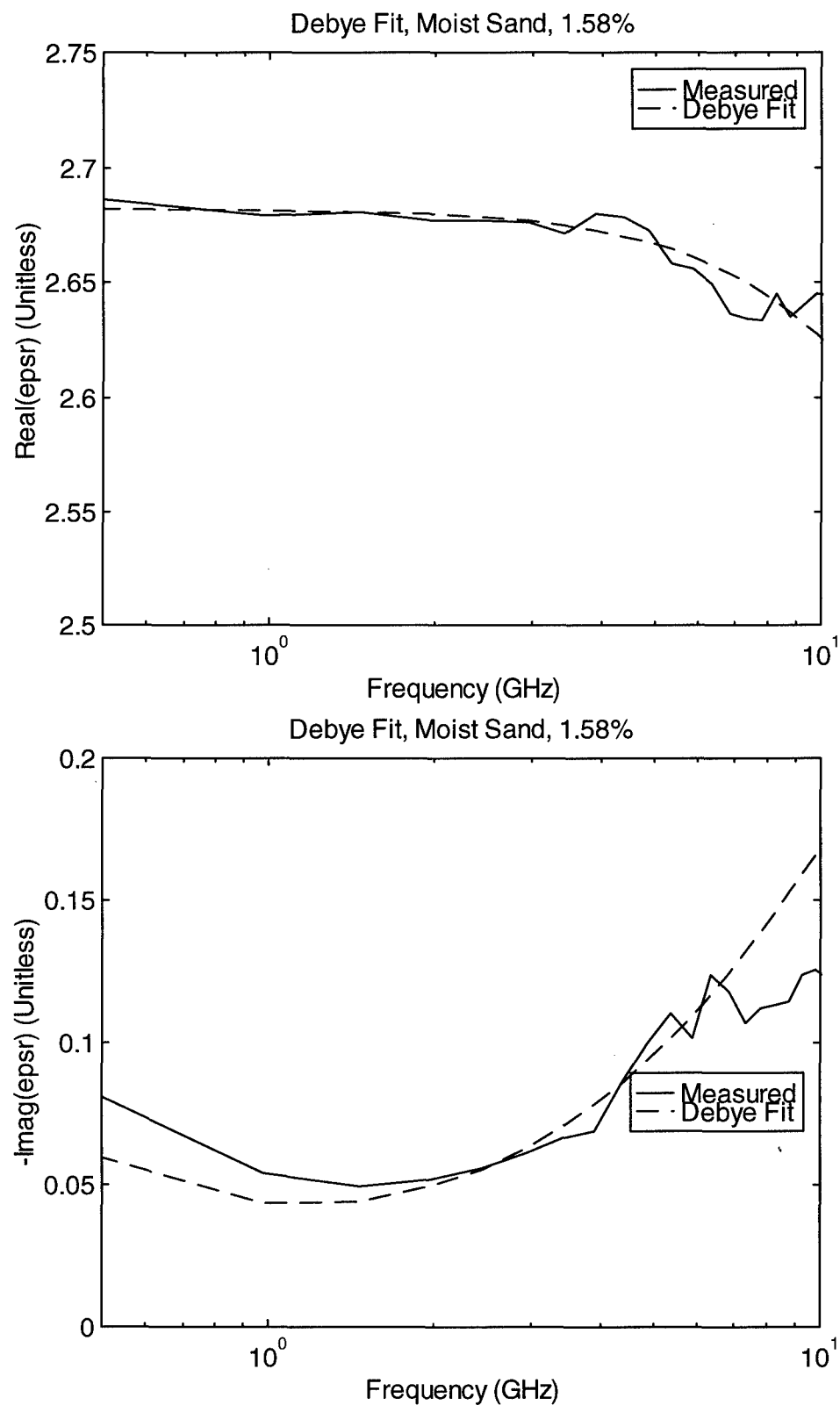
Figure 12.4. Measured dielectric constant of moist sand 1.58%, and the Debye model fit, including conductivity, real and imaginary parts.
