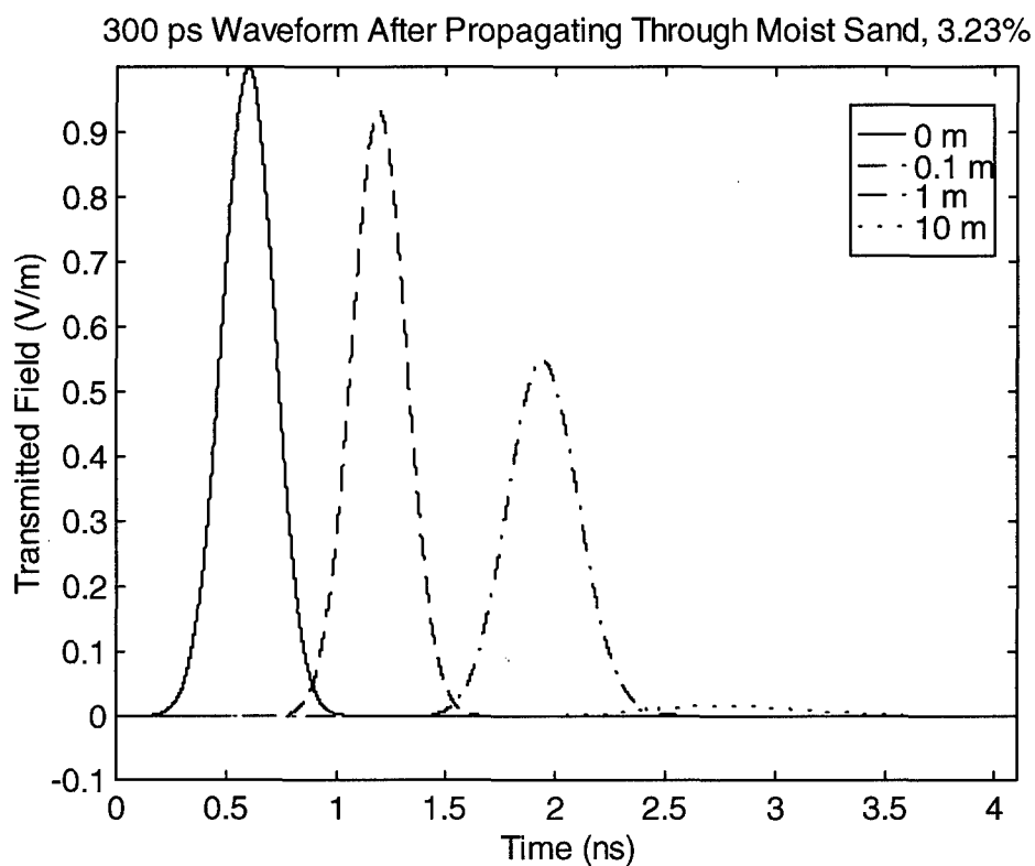
Figure 13.3. The propagated field of the 300 ps pulse at 0, 0.1, 1, and 10 meters, 1.58% top and 3.23% bottom. (Starting times shifted for clarity.)
