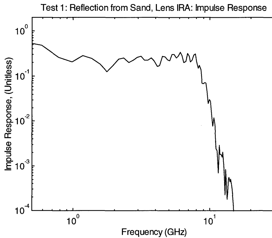
Figure 15.4. Frequency domain impulse response for sand reflection.
