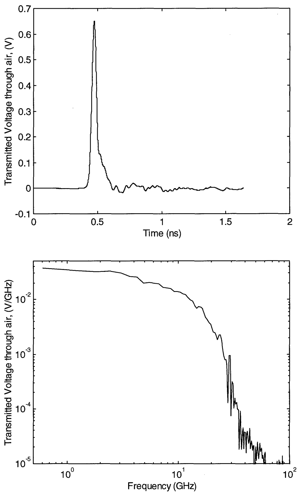
Figure 8.2. Air waveform for the concrete measurements, time domain (top) and frequency domain (bottom).
