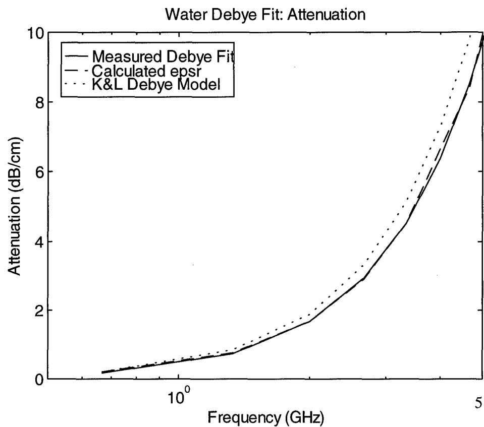
Figure 3.2. Comparison of the attenuation of water using the measured values, the Debye fit to the measurements, and the K&L Debye fit.
