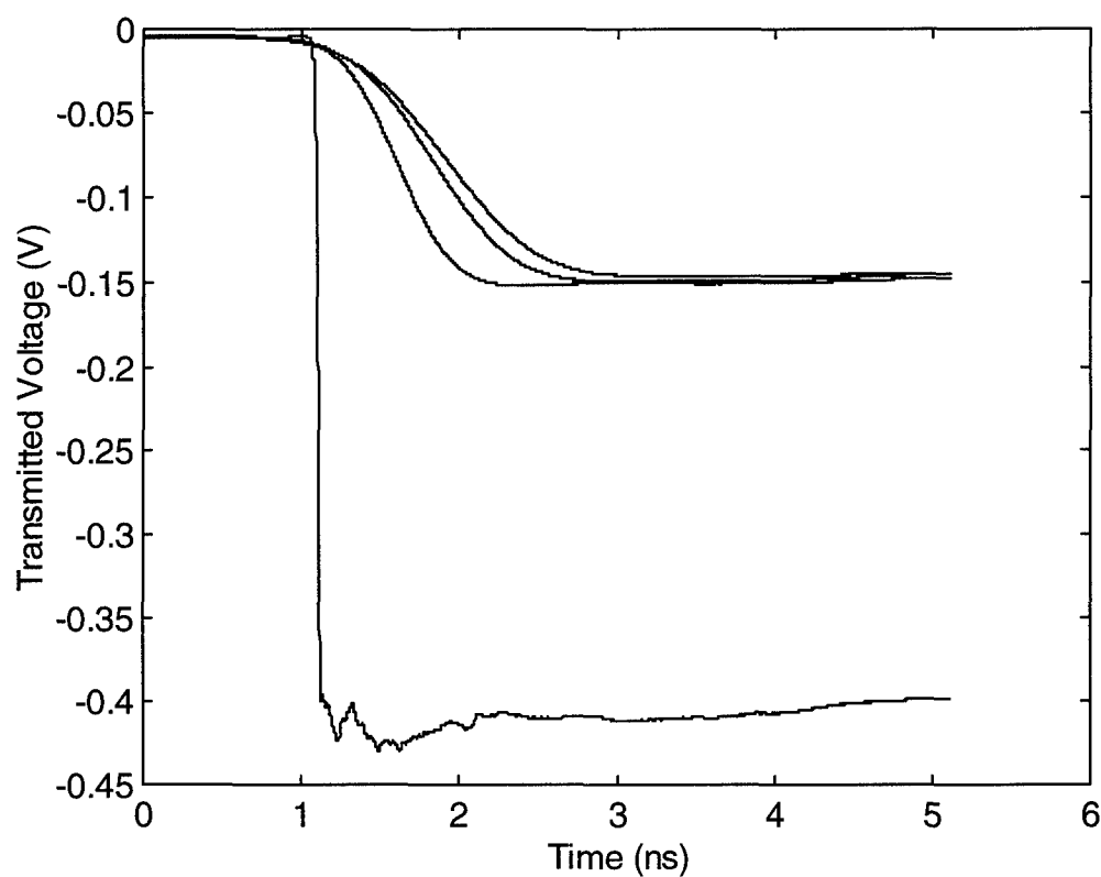
Figure 3.7. Raw data for the step transmission measurement
