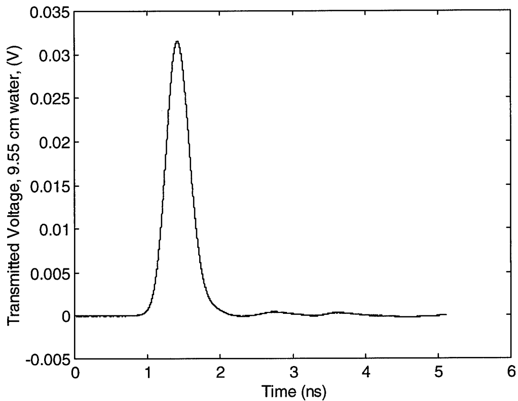
Figure 4.10. Signal transmitted through 9.55 cm of distilled water.
