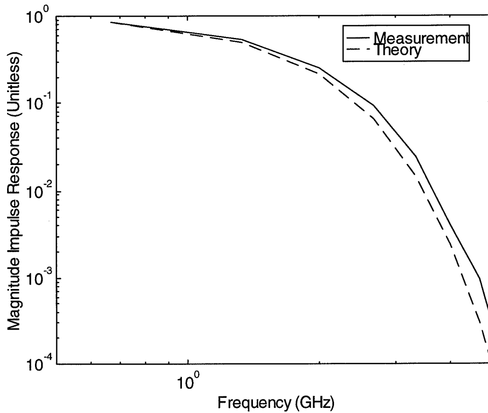
Figure 4.5 . Impulse response spectrum for propagation through 7.16 cm of water.
