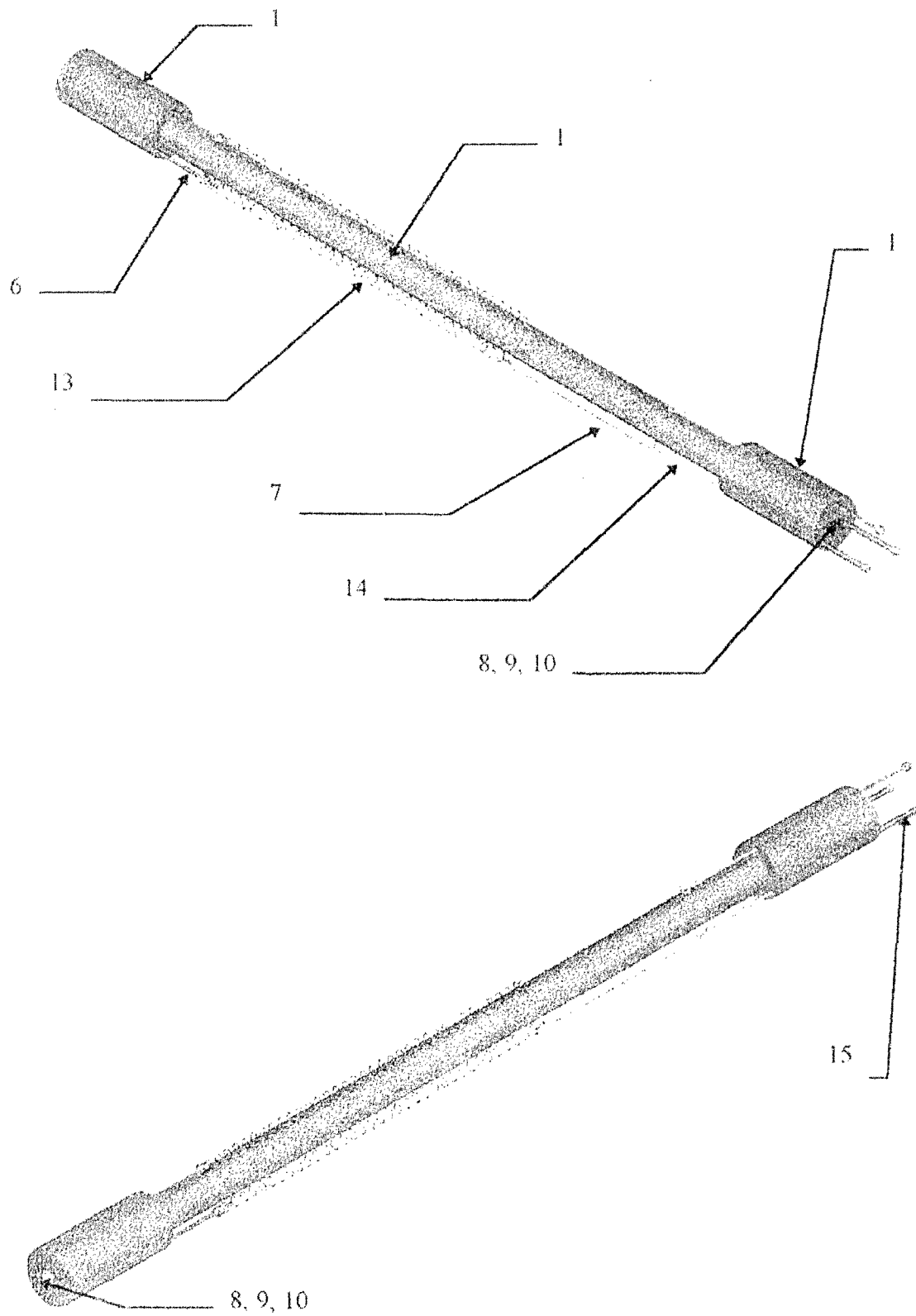
Figure 3.3. Coaxial transmission line apparatus.
