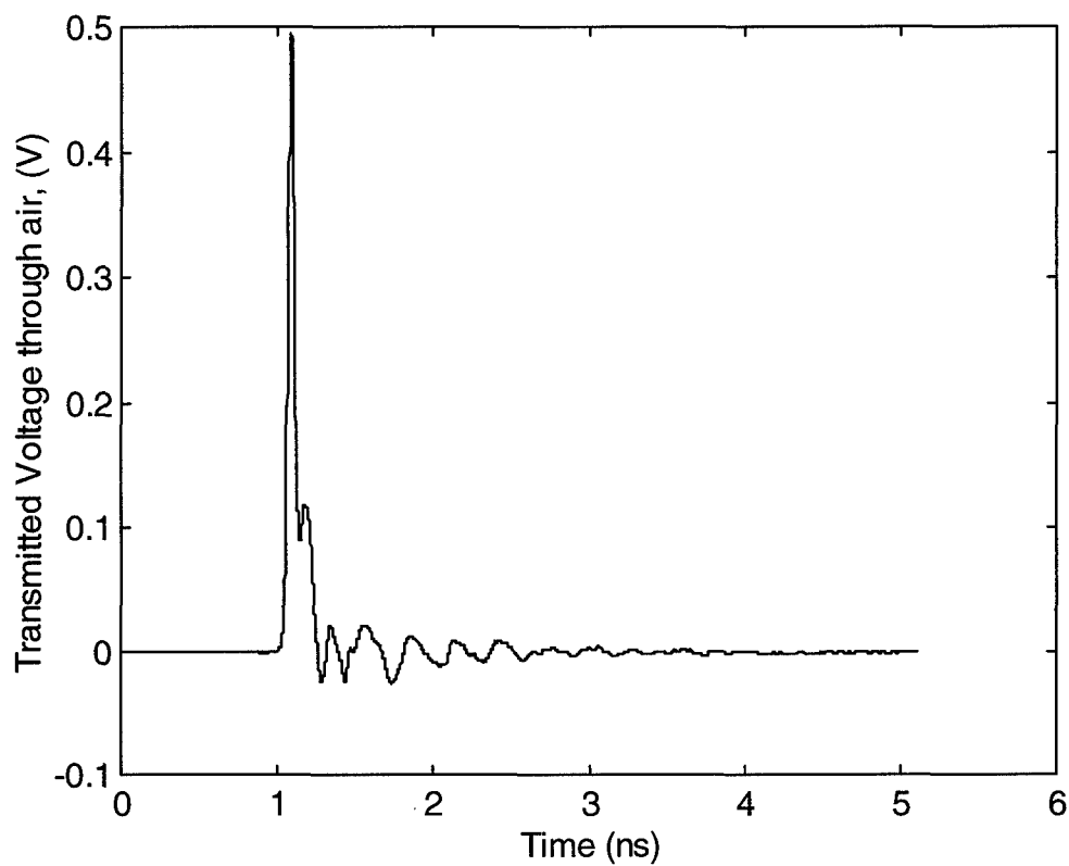
Figure 4.1. Transmitted waveform with no sample, 100 cm of air.
