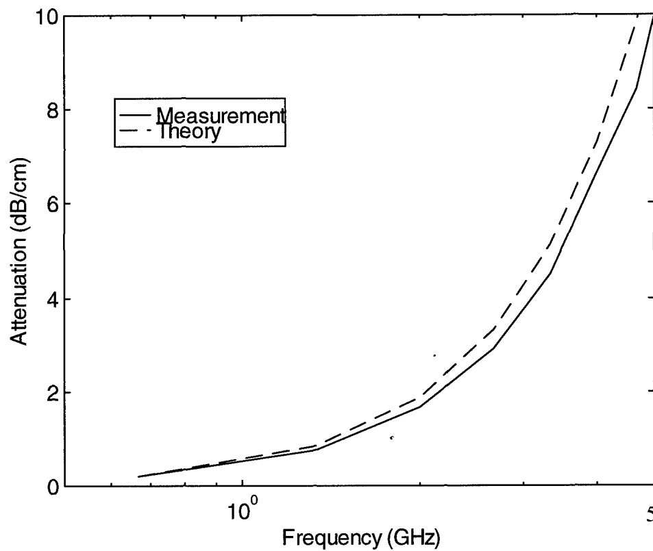
Figure 4.9. Attenuation coefficient of distilled water, measured with water columns 2.39 and 9.55 cm in length.
