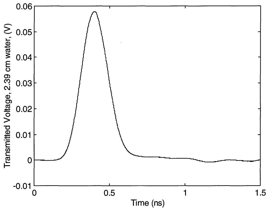
Figure 4.3. Signal transmitted through 2.39 cm of distilled water.
