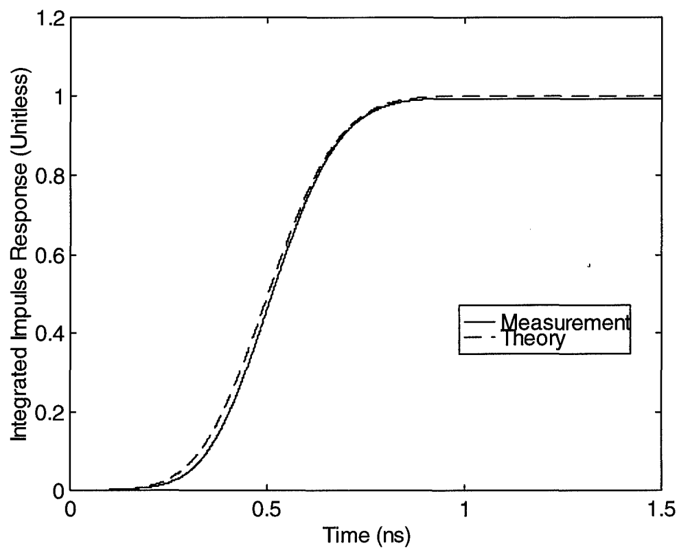
Figure 4.7. Integral of the impulse response for propagation through 7.16 of water.
