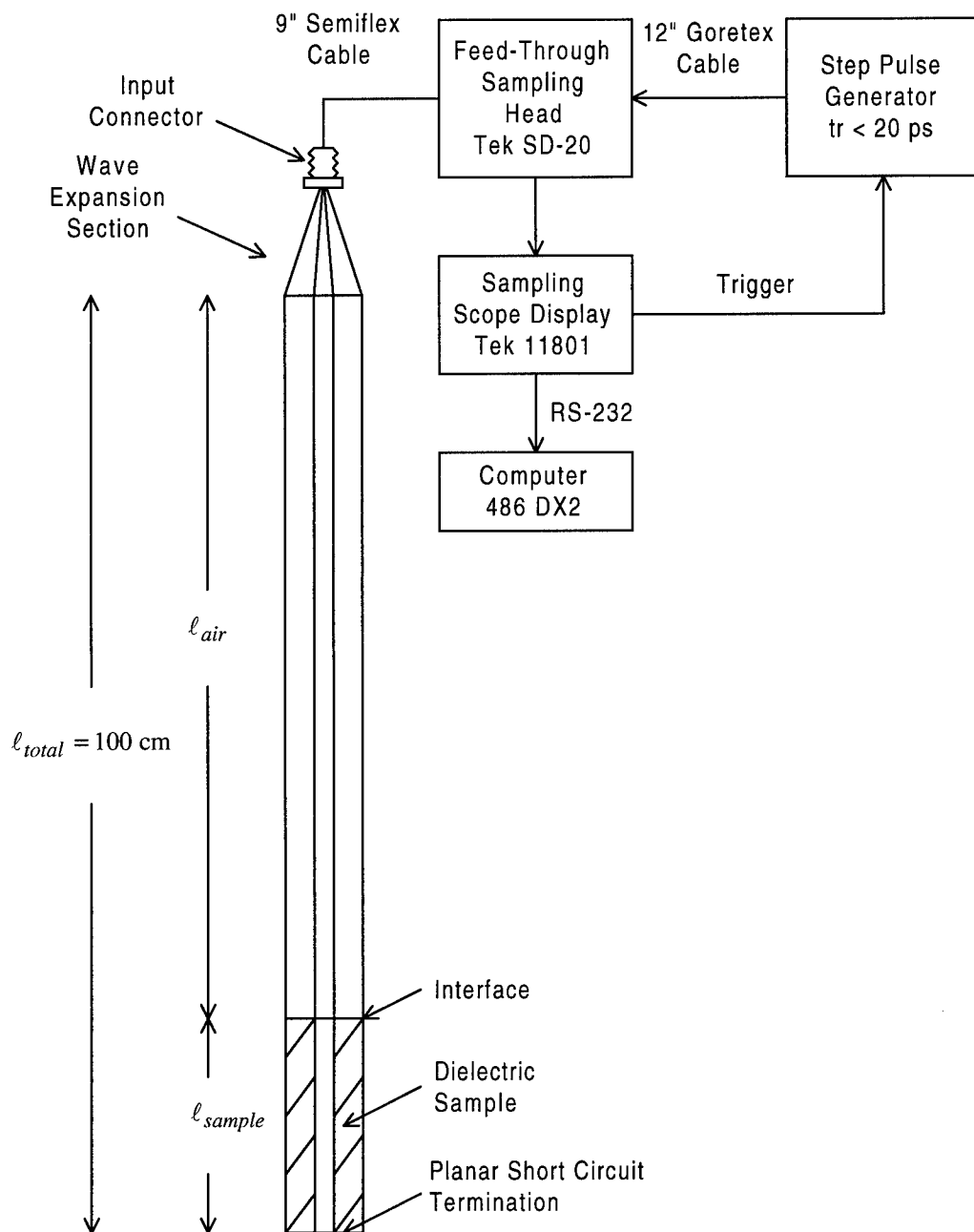
Figure 3.1. Instrumentation setup for measurements in TDR mode.
