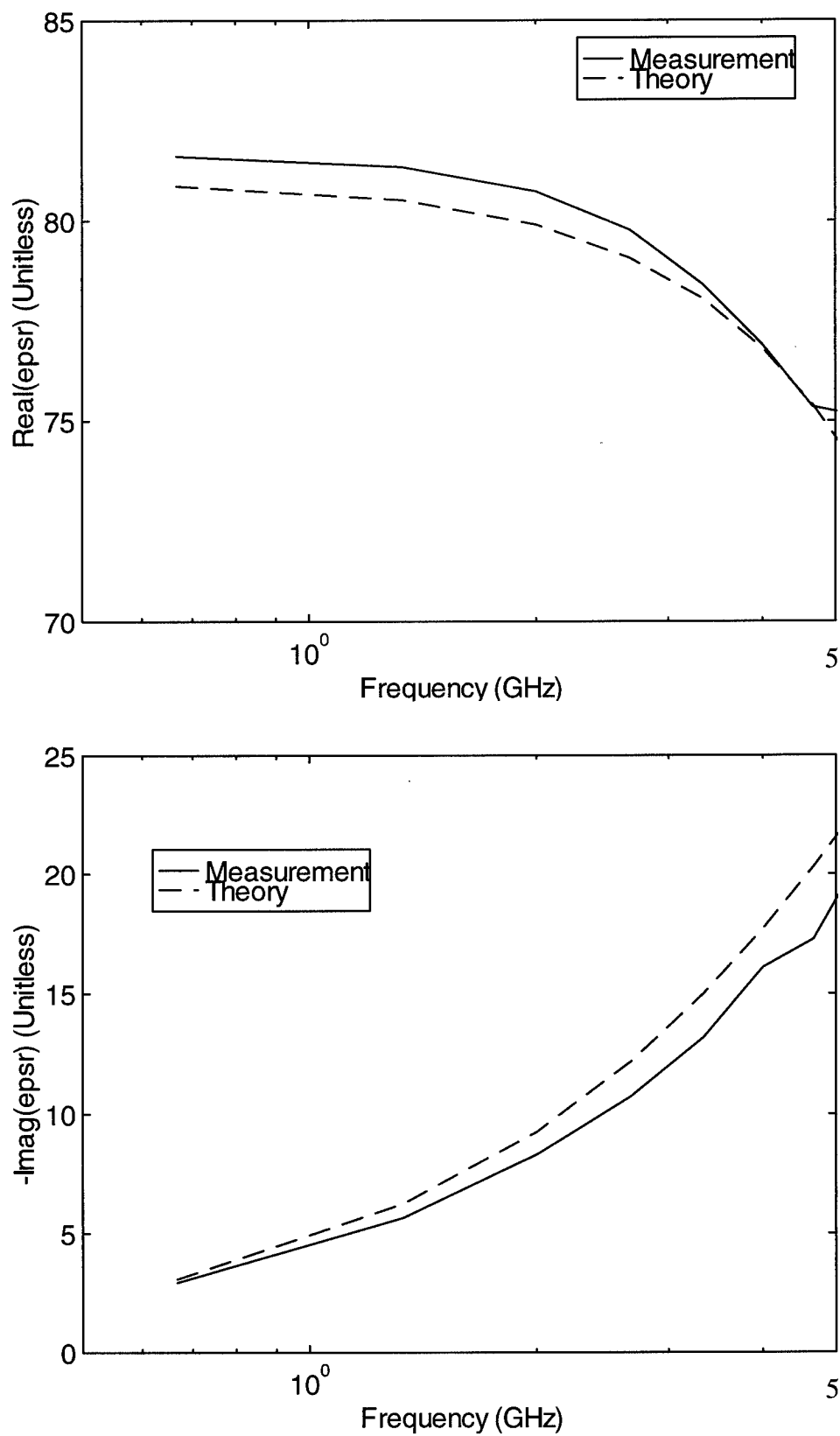
Figure 4.8. Real (top) and imaginary (bottom) parts of the measured dielectric constants of distilled water, measured with water columns 2.39 and 9.55 cm in length.
