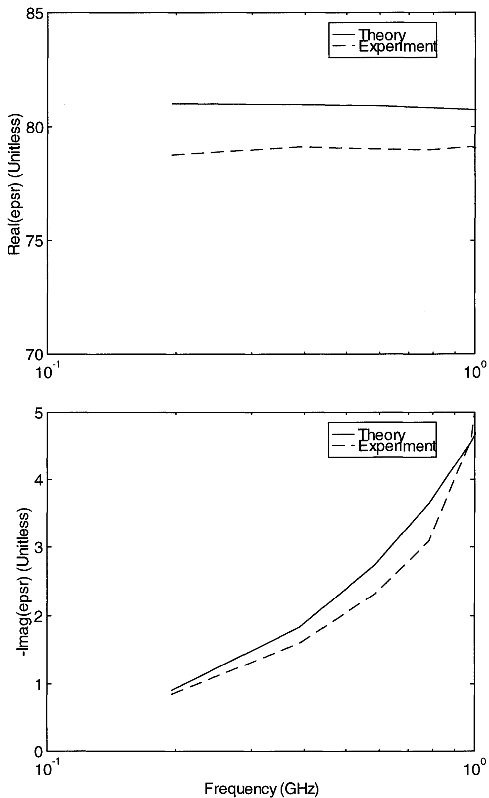
Figure 4.12. Real (top) and imaginary (bottom) parts of the measured dielectric constants of distilled water, using water columns 9.55 and 76.39 cm in length..
