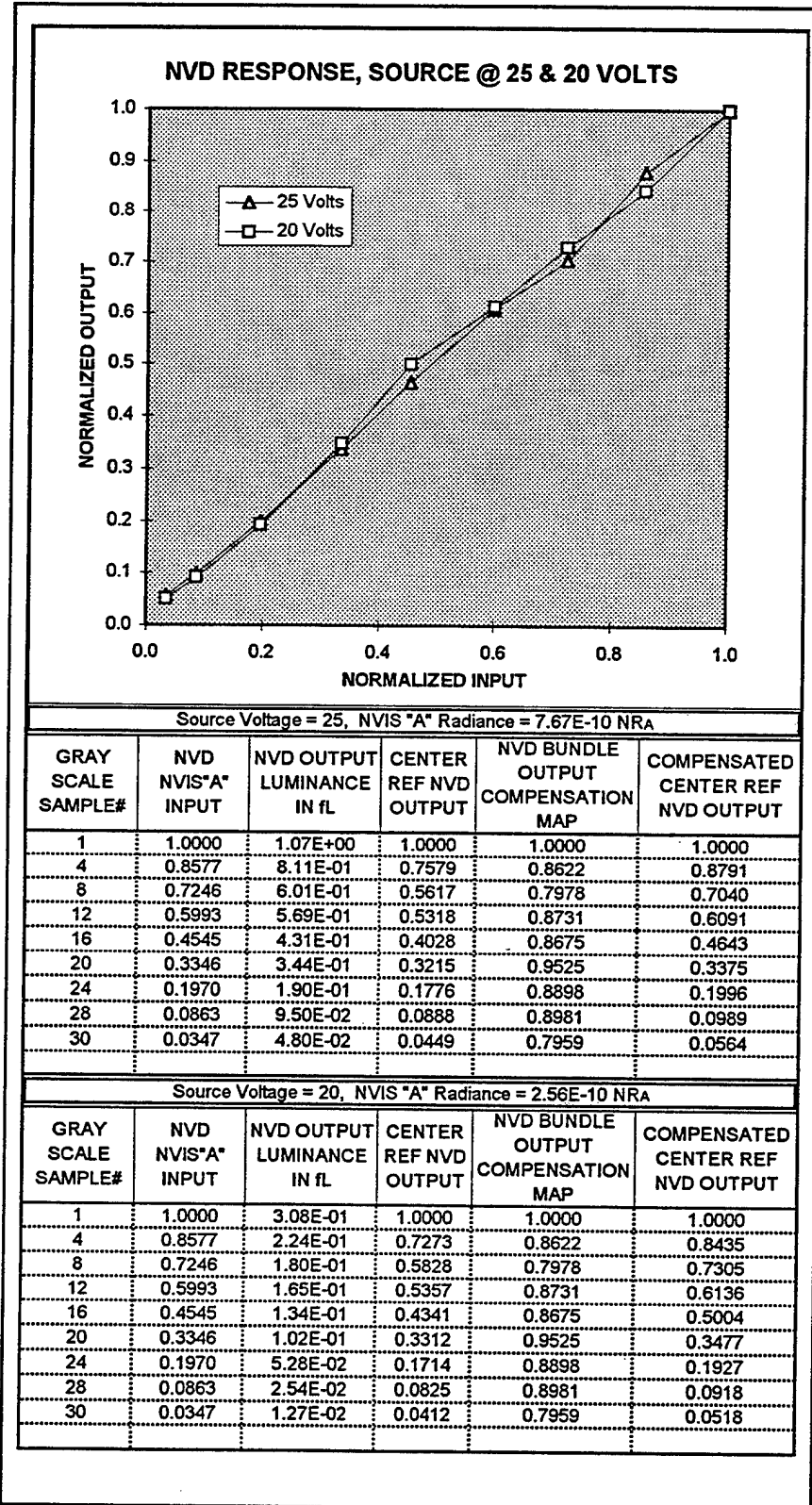
Figure 12. NVD Response, Source at 25 and 20 Volts
