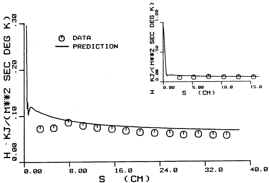
Figure 2-6. Heat transfer predictions of the experimental data of Murray and Stalling 6 R_i = 0.125 inch, M_\infty = 3.71 , Re = 9.85 \times 10^6 per meter, \Lambda = 60^\circ
