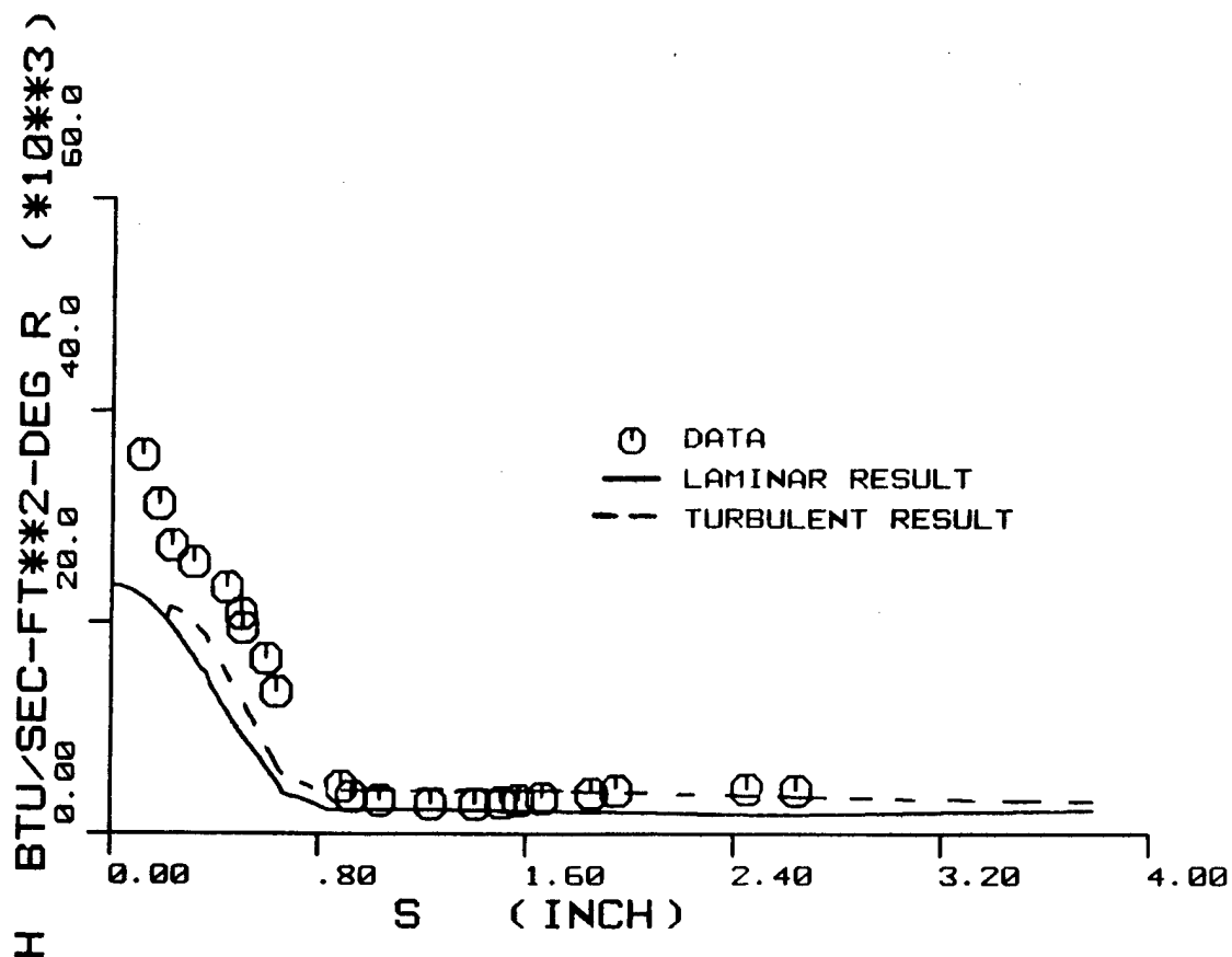
Figure 2-12. Heat transfer predictions of the experimental data of Hunt et al. 8 R_i = 0.5 inch, M_\infty = 7.98 , Re = 9.3 \times 10^5 (based on leading edge diameter), \Lambda = 60^\circ
