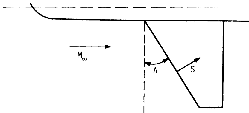
Figure 2-1. Sketch of swept wing geometry
