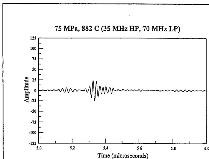
Figure 16 - A reflection of ultrasound from the back side of the substrate was recorded at a temperature of 882 °C and an argon gas pressure of 75 MPa. This signal was filtered after acquisition using 35 MHz high pass and 70 MHz low pass filters.
