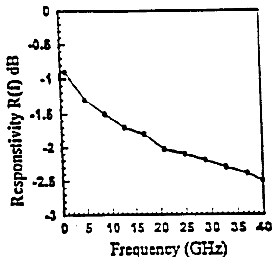
FIG. 14. Responsivity, R(f) of a polymer electro-optic modulator.
