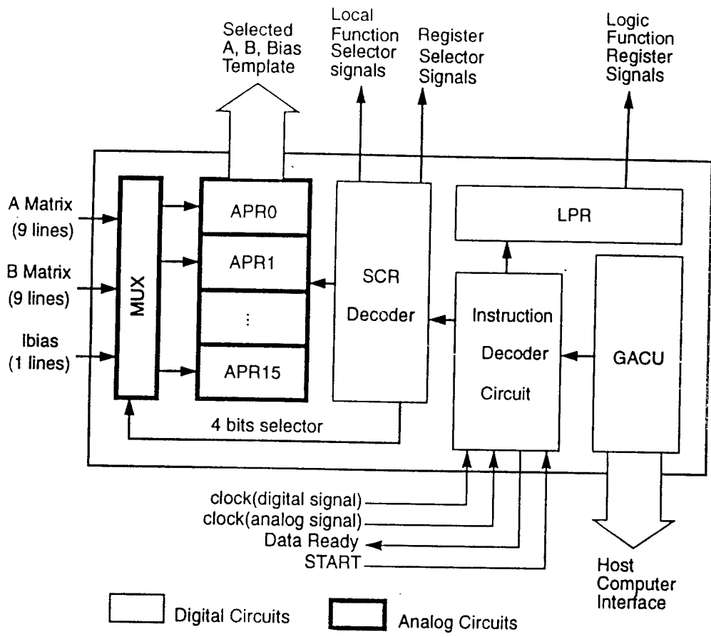
Figure 3-5 Block diagram of the GAPU.
