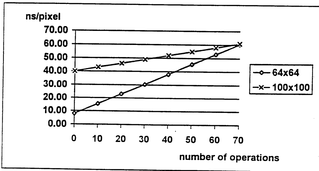
Figure 3-24 The average number of operation is from 5 to 35. In this region the 64 x 64 CNN chip with A-RAM is faster than the 100 x 100 CNN chip.
