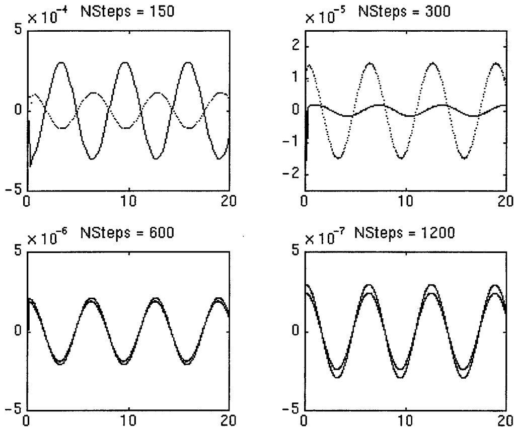
FIGURE 14. Richardson Error Estimate, \lambda = -10 , Order 2.
