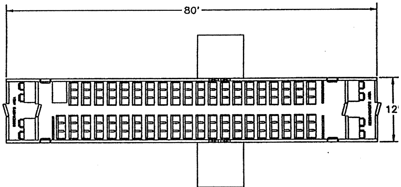
Figure 6. Narrow Body Floor Plan (No Scale)
