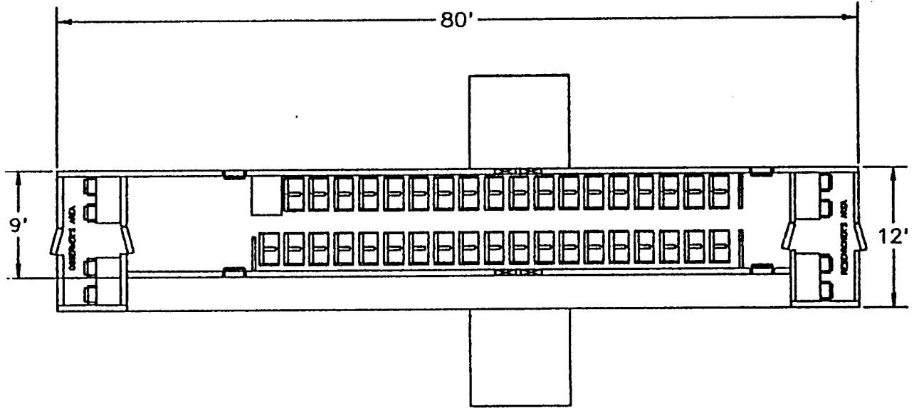
Figure 5. Commuter Body Floor Plan (No Scale)
