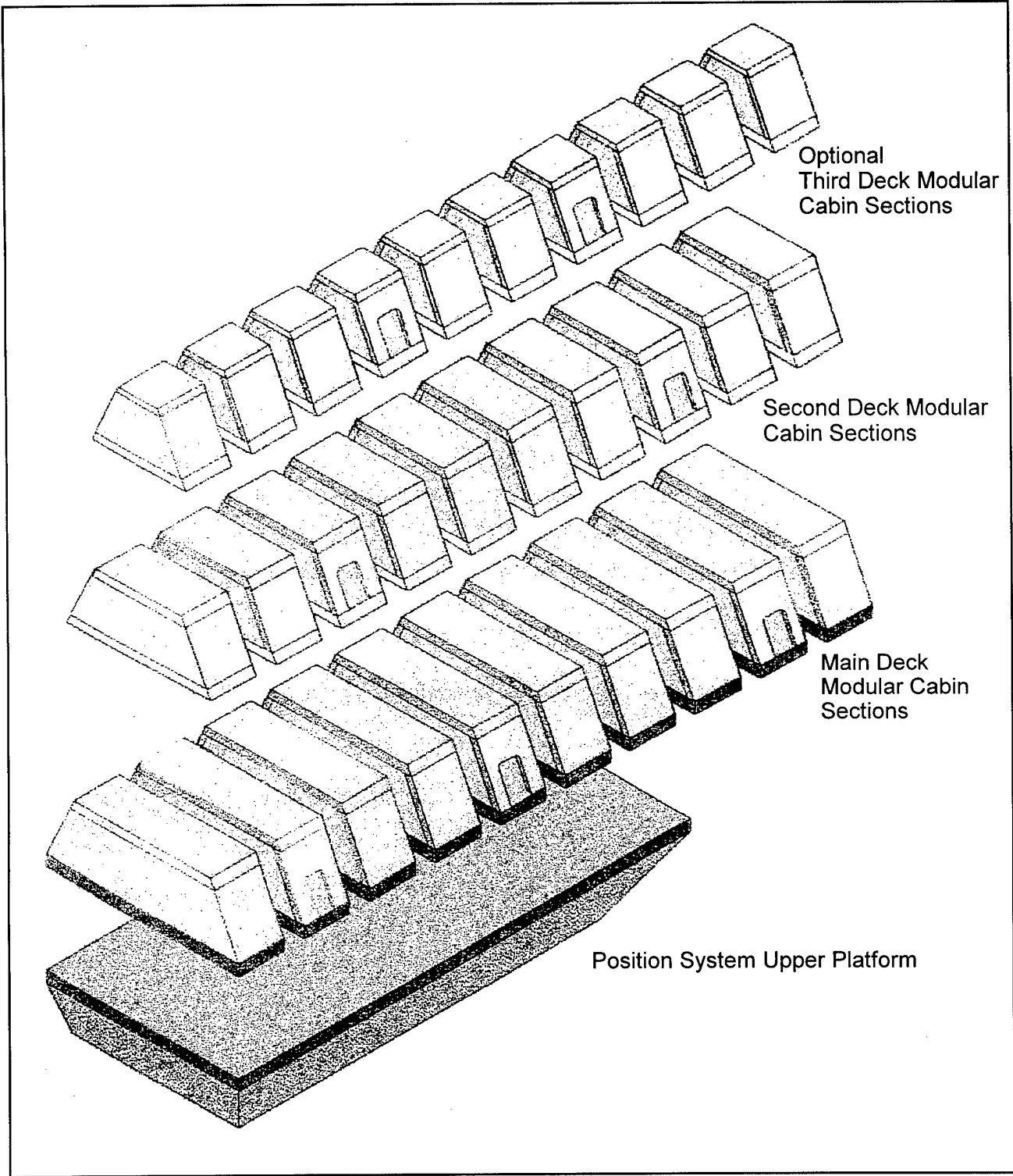
Figure 10. Artist's Concept Wide/Mega Body Simulator
