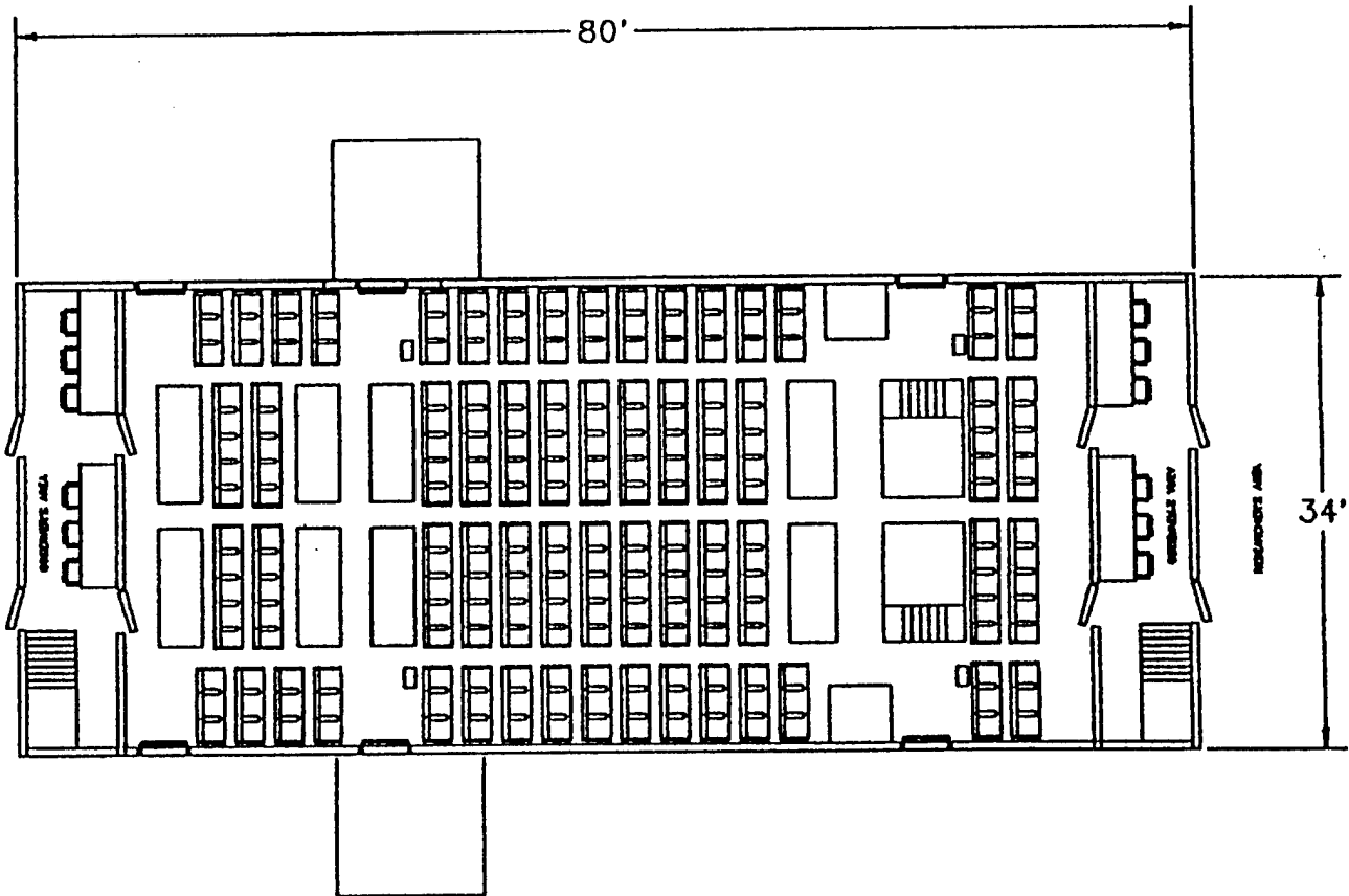
Figure 8. Mega Body Deck Floor Plan (No Scale)
