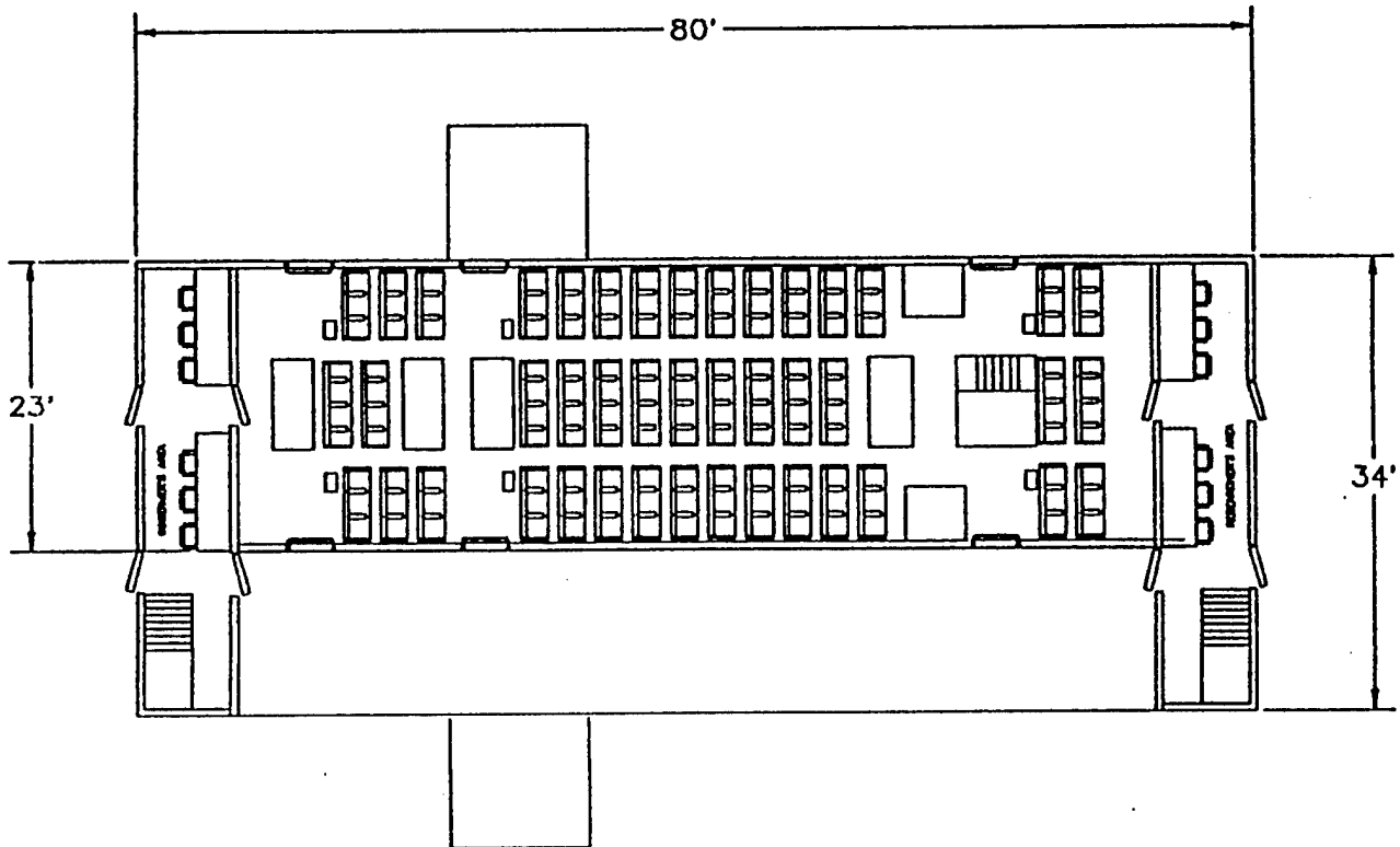
Figure 7. Wide Body Deck Floor Plan (No Scale)
