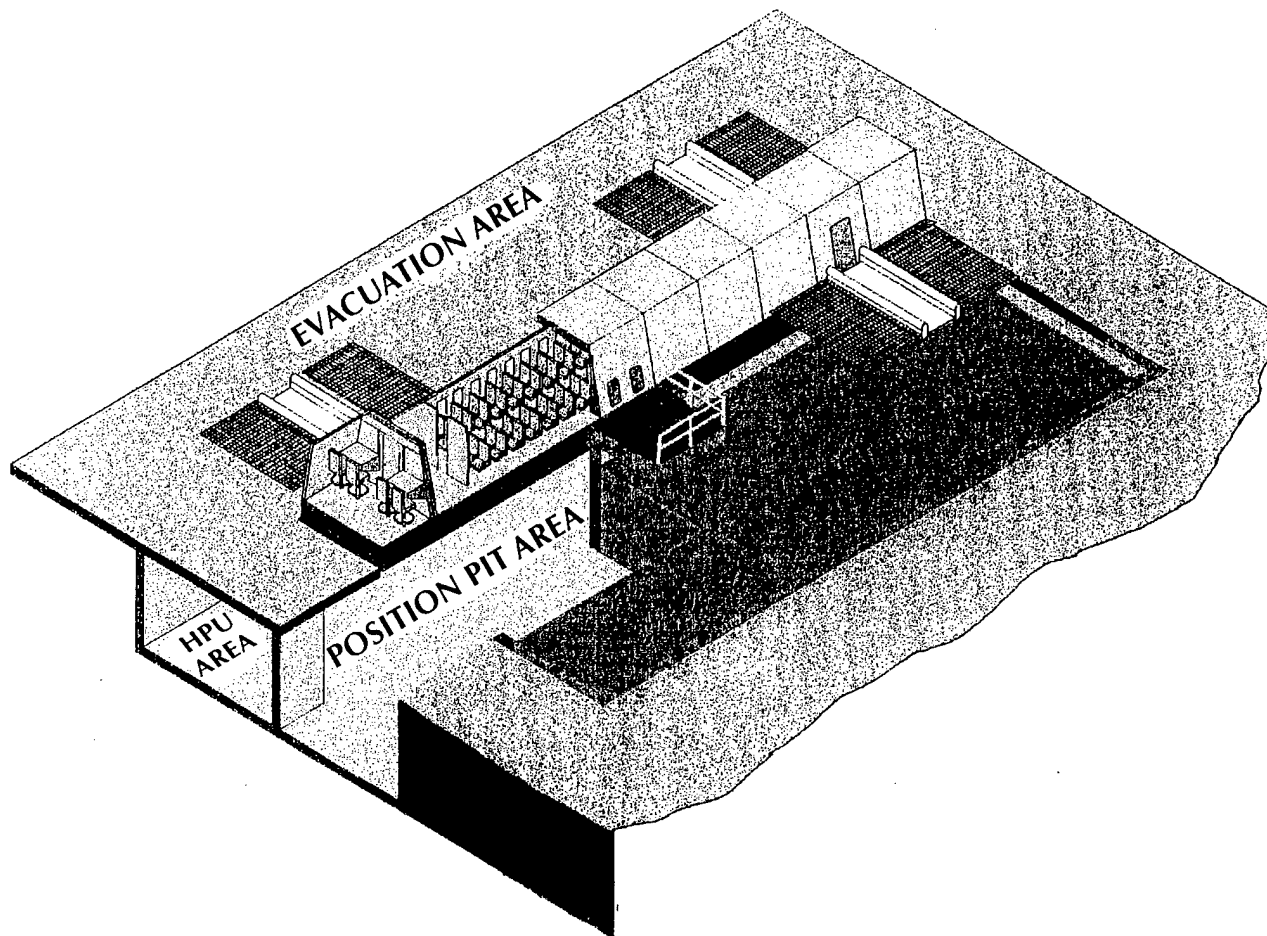
Figure 1. Artist's Concept Commuter Body Simulator (Shown at Rest Position)
