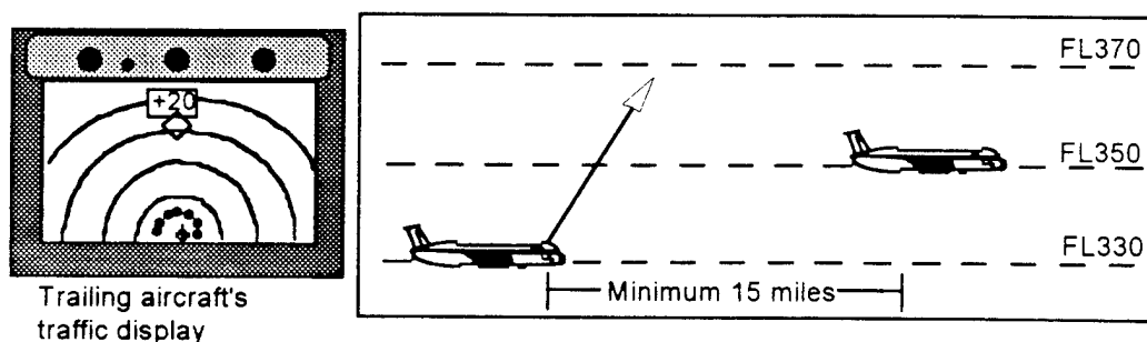
Figure 4.2-2. The ITC Concept
