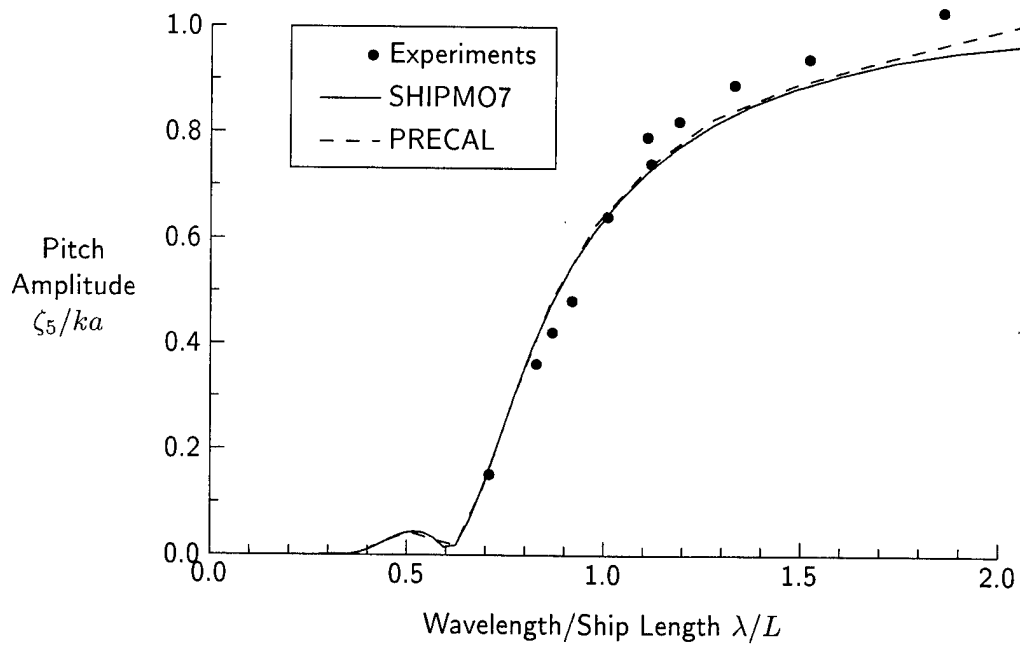
Figure 29: Pitch, F_n = 0.29 , \beta = 180 degrees
