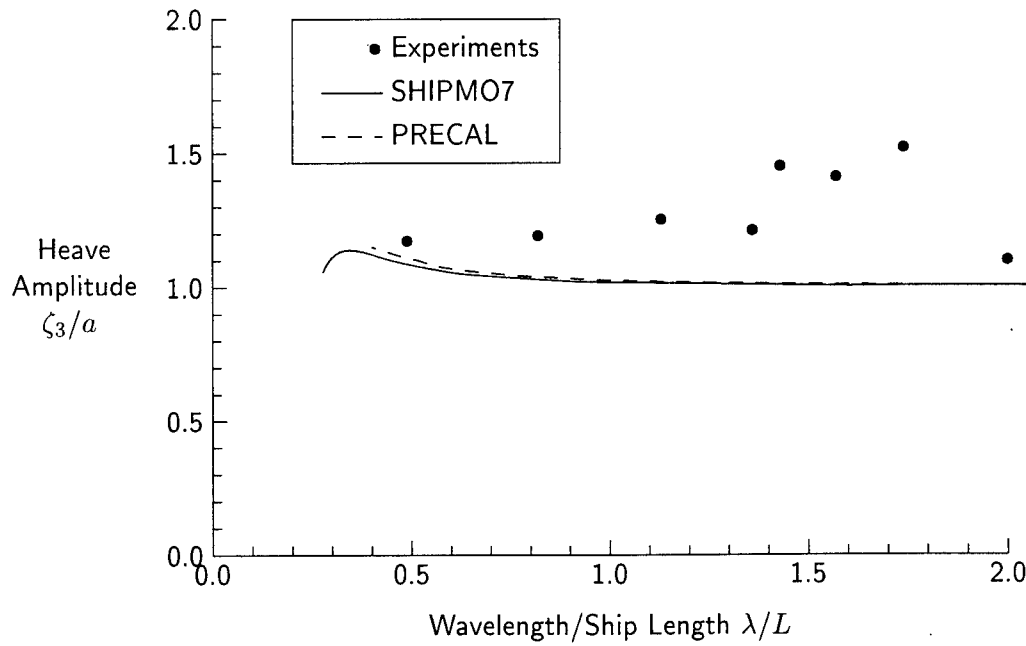
Figure 7: Heave, Fn = 0.21 , \beta = 90 degrees
