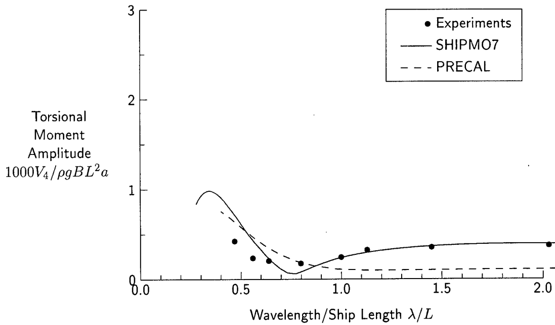
Figure 117: Torsional Moment at Station 5, Fn = 0.21 , \beta = 120 degrees
