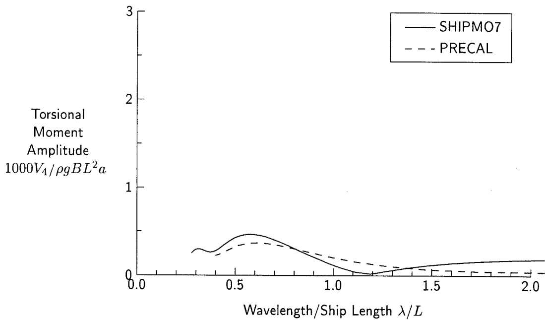
Figure 135: Torsional Moment at Station 5, Fn = 0.29 , \beta = 150 degrees
