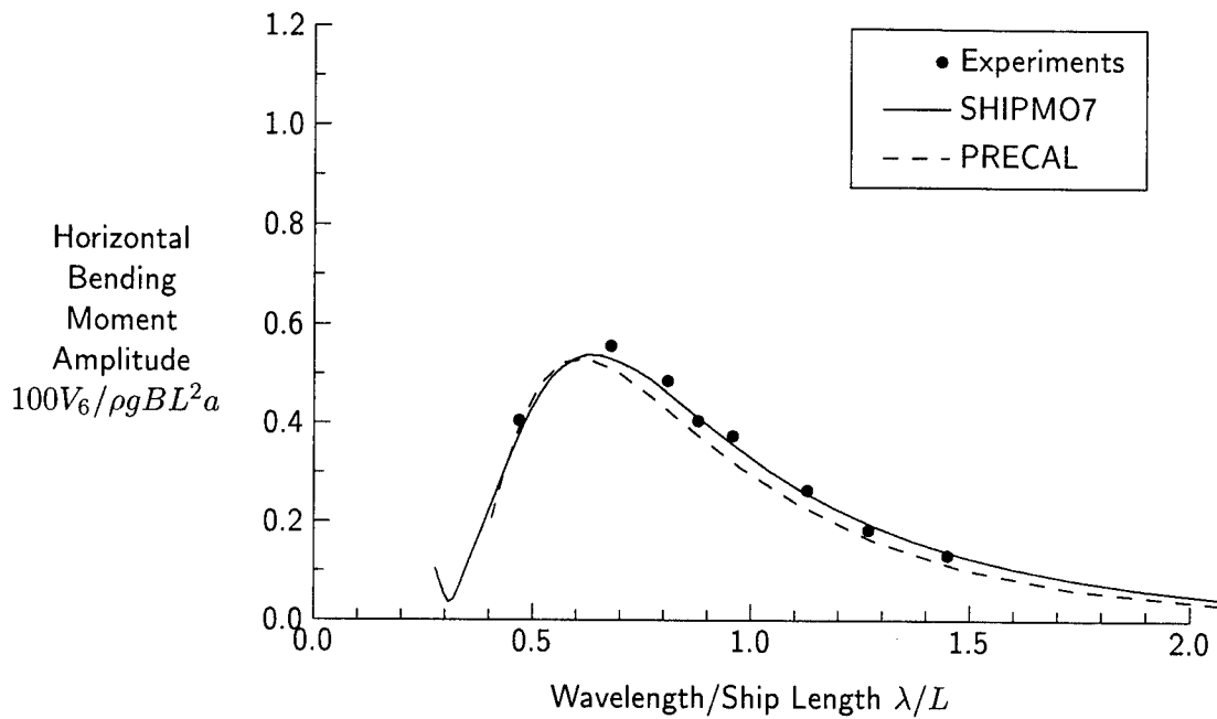
Figure 94: Horizontal Bending Moment at Station 10, F_n = 0.21 , \beta = 150 degrees
