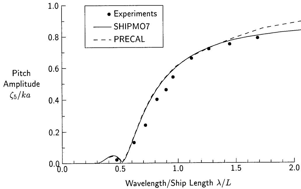
Figure 22: Pitch, Fn = 0.21 , \beta = 150 degrees
