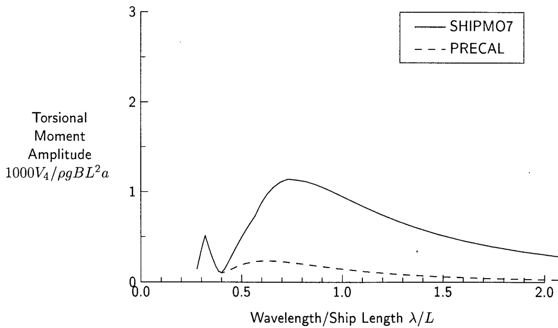
Figure 123: Torsional Moment at Station 5, Fn = 0.29 , \beta = 30 degrees
