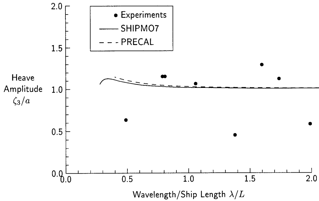
Figure 14: Heave, Fn = 0.29 , \beta = 90 degrees
