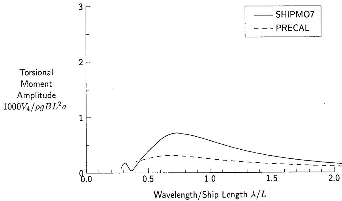
Figure 125: Torsional Moment at Station 13, F_n = 0.29 , \beta = 30 degrees
