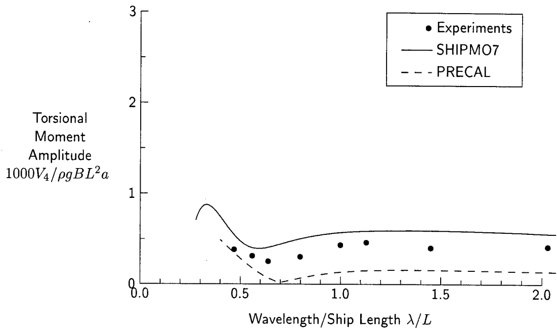
Figure 118: Torsional Moment at Station 10, F_n = 0.21 , \beta = 120 degrees
