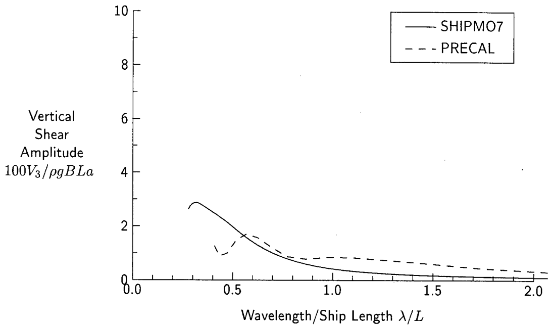
Figure 151: Vertical Shear Force at Station 10, F_n = 0.21 , \beta = 120 degrees
