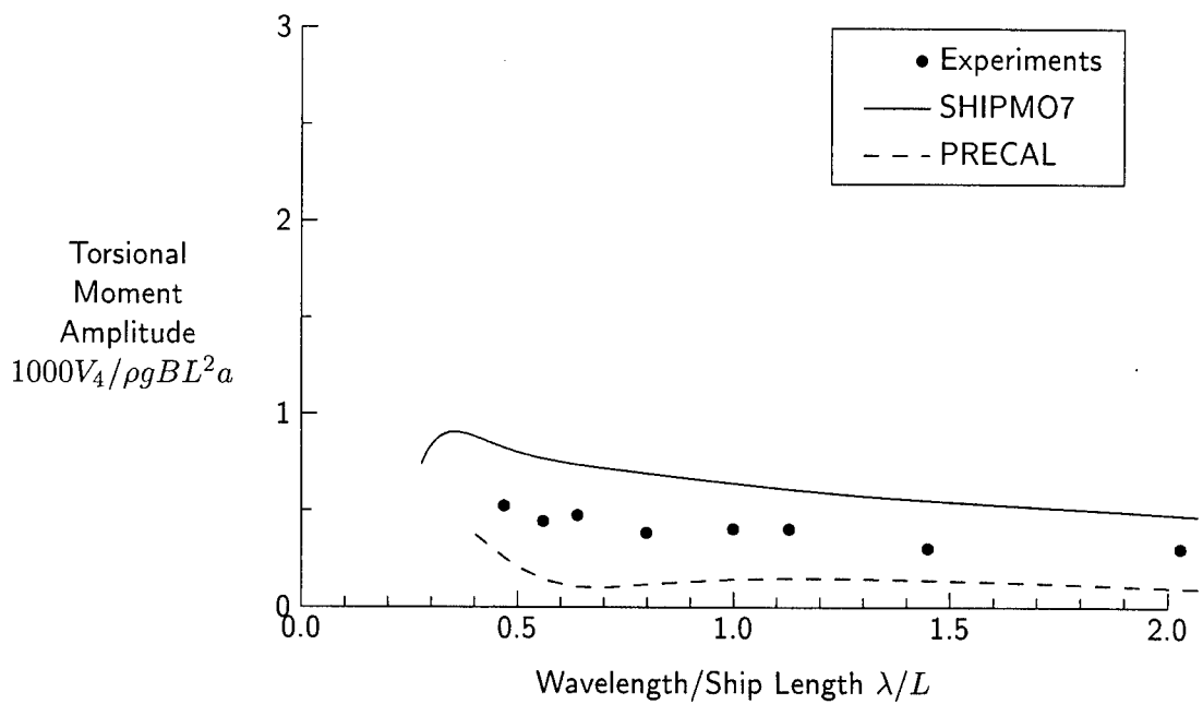
Figure 119: Torsional Moment at Station 13, F_n = 0.21 , \beta = 120 degrees
