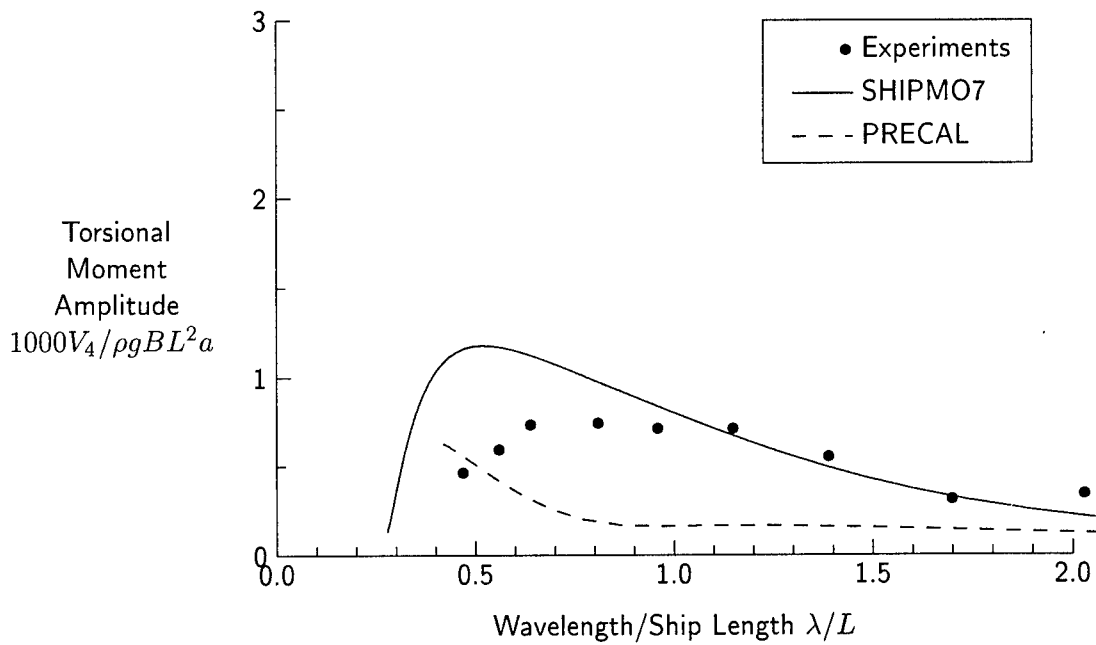
Figure 113: Torsional Moment at Station 13, F_n = 0.21 , \beta = 60 degrees
