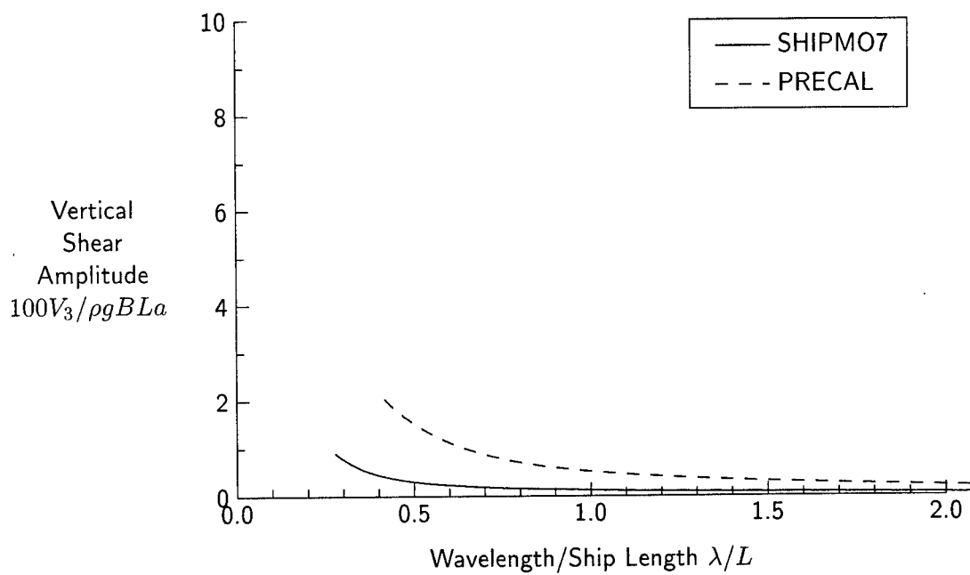
Figure 169: Vertical Shear Force at Station 10, F_n = 0.29 , \beta = 90 degrees
