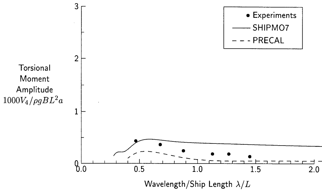
Figure 122: Torsional Moment at Station 13, Fn = 0.21 , \beta = 150 degrees
