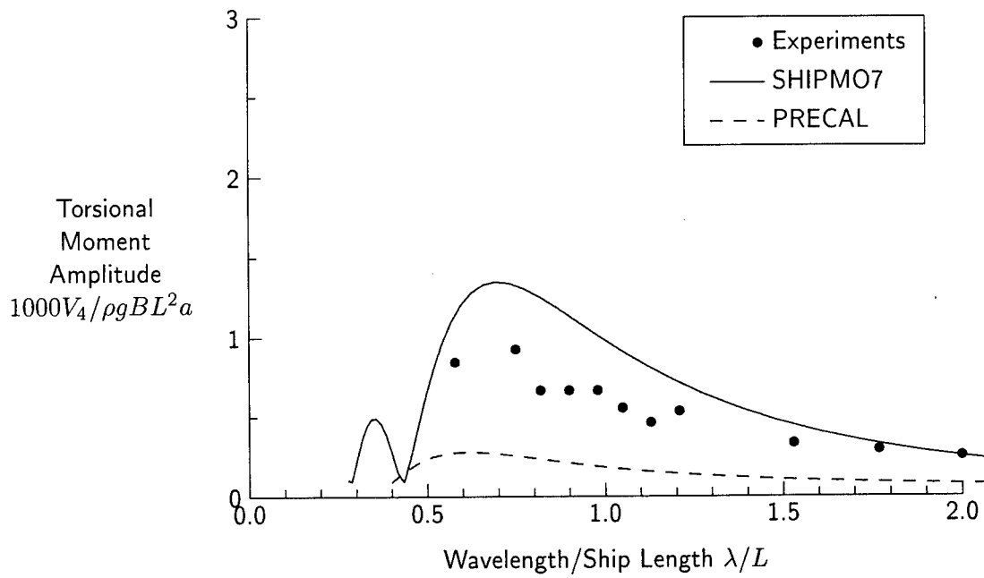
Figure 109: Torsional Moment at Station 10, Fn = 0.21 , \beta = 30 degrees
