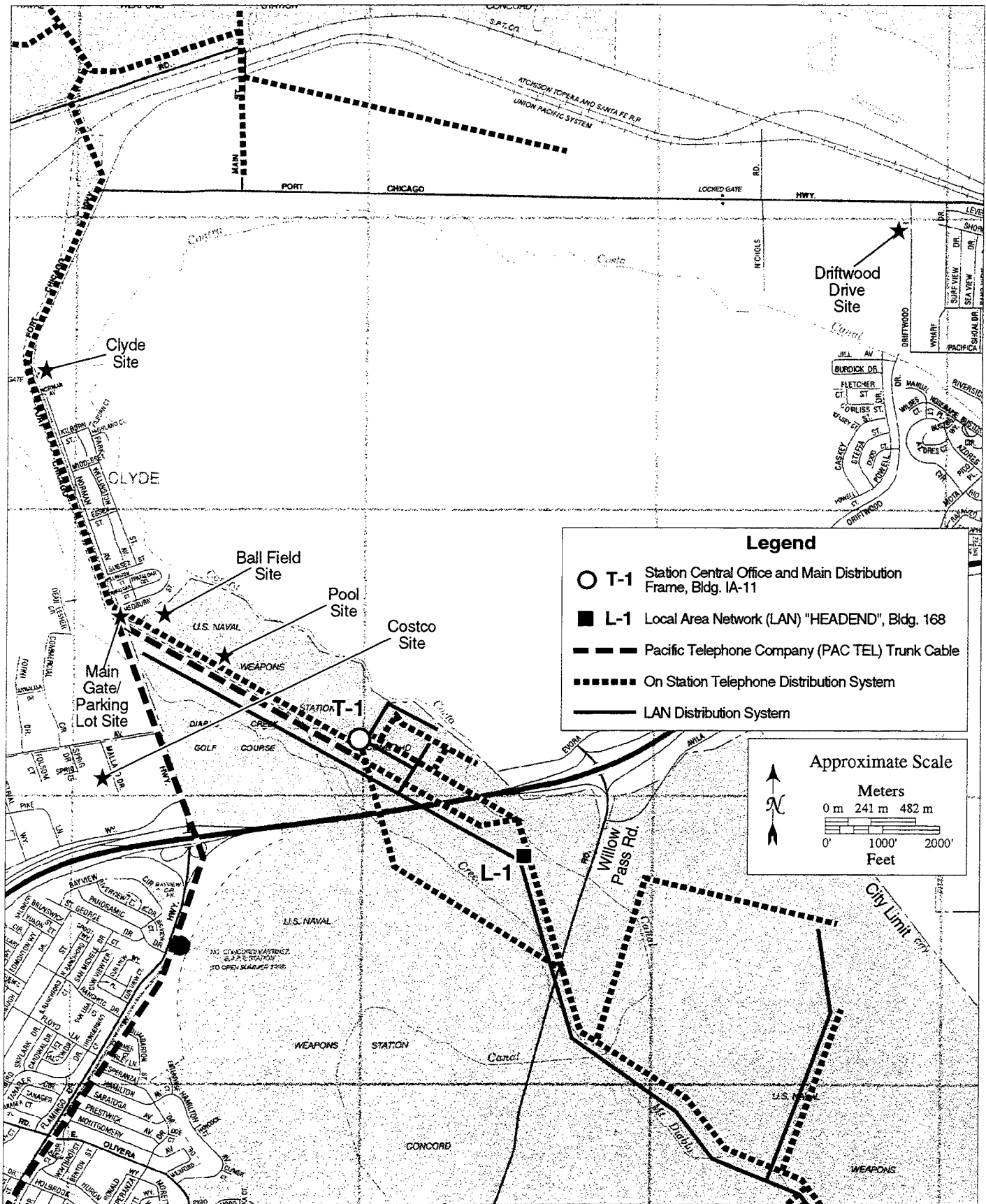
Figure 3-22. Telecommunications Distribution System
