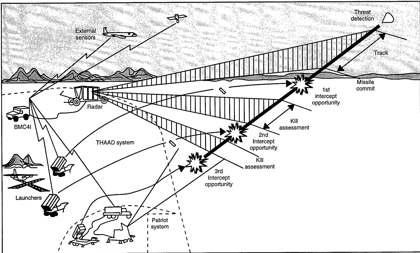
Figure 1: THAAD System
