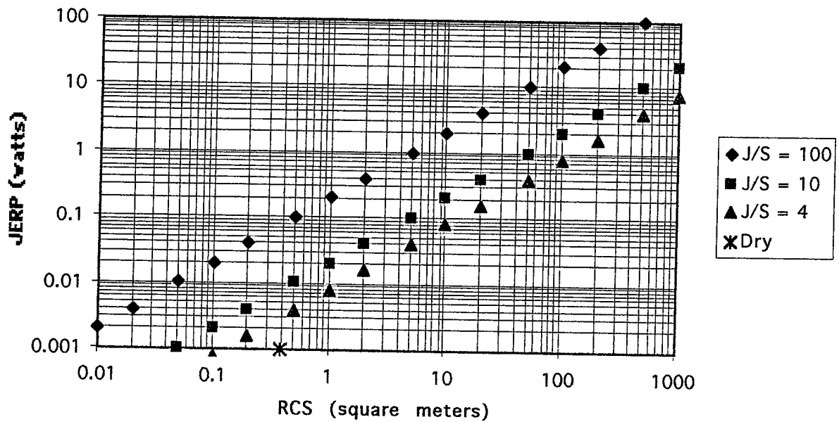
Figure V-3: Air-to-Air Scenario with Deception Jamming (Range = 35km)
