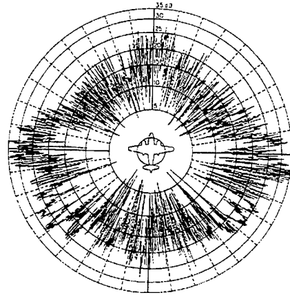
Figure III-1: Typical Aircraft RCS (after Skolnik)
