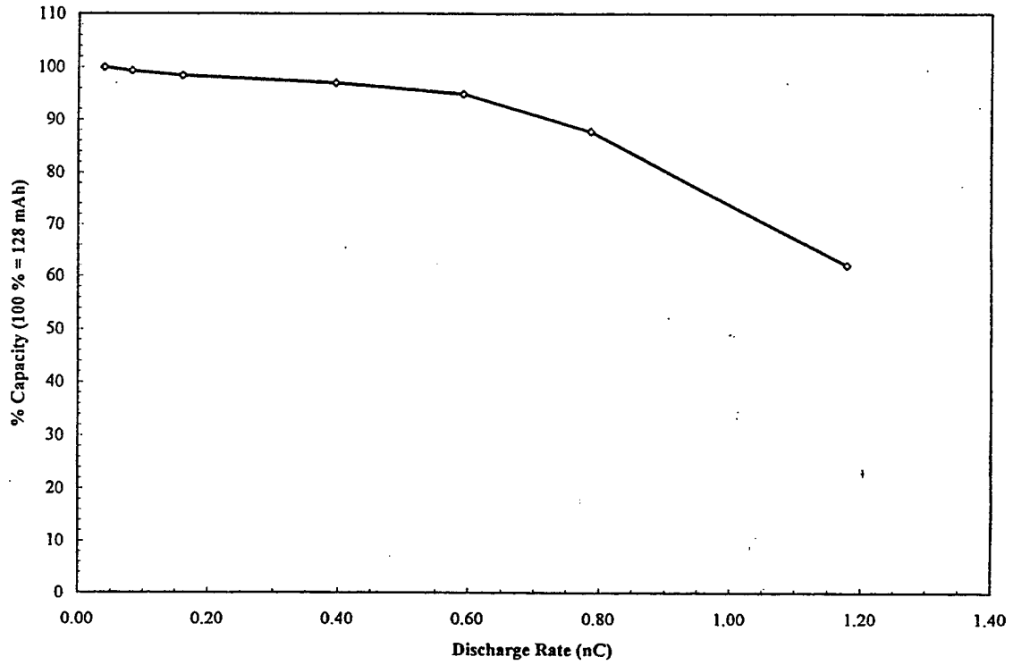
Figure 11. Power-rate curve of nose-fuse cell.
