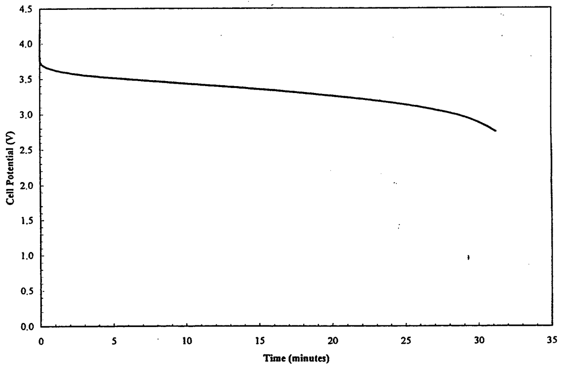
Figure 12. Discharge curve of nose-fuse cell on 150-mA (1.25 C) load.
