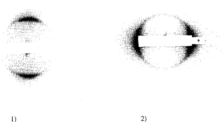
fig. 3: X-ray patterns in tangential geometry, sample a ; 1)- L_\alpha^* phase oriented perpendicularly to the Couette boundaries, \dot{\gamma}=35 \text{ s}^{-1} 2)- L_\alpha^* phase oriented mostly parallel to the Couette boundaries, \dot{\gamma}=60 \text{ s}^{-1} .
