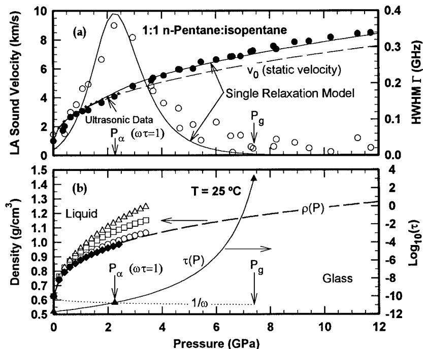
Figure 2. High-pressure Brillouin scattering results for 1:1 n-pentane:isopentane at 25 °C. (a) Sound velocity (•) and HWHM (o) data. Also shown are sound velocities below 2.5 GPa determined ultrasonically (+). 31 The solid lines represent fits using a single relaxation time model and the dashed line is the "relaxed" velocity calculated from the fits. (b) Relaxation time (solid line) determined from a modified VTF fit to the measured points (▲). Also shown are direct density measurements due to Houck (◆), 31 our calculated EOS (dashed line) which accounts for relaxation effects, EOS calculations from our Brillouin data which do not consider relaxation and where C_p (o), \gamma (□), and \alpha (Δ), respectively, are assumed constant as in several early studies.
