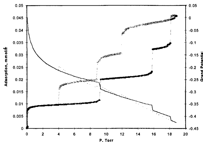
Fig. 5 NLDFT isotherm of Kr adsorbed on graphite in a 14\sigma_{\text{Kr-Kr}} slit pore at 90 K. The well depth of the Kr-graphite interaction potential has been reduced by 10 %. The lower curve (filled circles) is the adsorption branch of the isotherm with 4 layering transitions. The upper curve (open circles) is the desorption path from the 4-th layer. Thin solid line - the grand potential along the adsorption branch, thin dashed line - the grand potential along the desorption branch.
