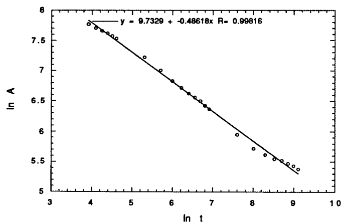
Fig.1 \ln A vs. \ln t for A+2B \rightarrow 0 reaction using the "scanning" method on a 2d lattice.
