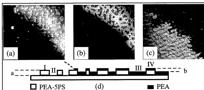
Figure 7: Partial coverage of PEA-5PS by PEA homopolymer. 40×40 μm 2 3-fold AFM measurement before annealing. Brighter contrast refer to higher values in topography, lateral force and Young's modulus (stiffness). The upper right triangular area is PEA homopolymer covered. The lower left triangular area is the bare PEA-5PS graft copolymer surface. (a) Topography image. (b) Lateral force image. (c) Elastic response exhibits stiffer graft copolymers ( bright ) than homopolymers ( dark ). (d) Sketch: Represents a topographical cross-section. The left and right side corresponds to the measured bottom and top triangular AFM area, respectively. The height differences are a = 28±2 nm and b = 8±2 nm. Areas are distinct with Roman numbers (c.f. Table II).
