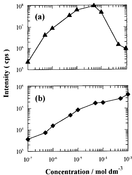
Fig 2. Dependence of the observed emission intensity of rhodamine 101 at 585 nm on concentration: (a) conventional geometry, (b) EWIFS ( \Lambda = 154 nm ).
