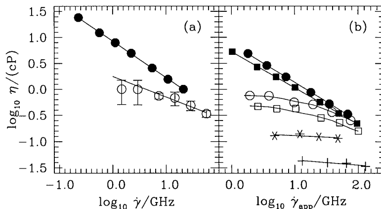
Figure 3: (a) The actual viscosities with shear rate determined from the flow profiles for hexadecane (○) at 6 layers and squalane (●) at 4 layers. Both have \epsilon_w = 0.7 kcal/mol. (b) The effective viscosities for hexadecane and squalane for various number of layers. For hexadecane symbols are at \epsilon_w = 0.7 kcal/mol, (○) 12 layers and (□) 4 layers; at \epsilon_w = 0.1 kcal/mol, (*) 9 layers and (+) 4 layers. For squalane the symbols are for \epsilon_w = 0.7 kcal/mol at (■) 4 layers and (●) 6 layers.
