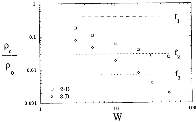
FIG. 3. The density of particles remaining on the baguette-like lattice at the dimensional crossover time normalized by the initial particle density, \frac{\rho_c}{\rho_o} , as a function of lattice width, W . For comparison, the horizontal lines represent the normalized density of particles, f_d , remaining on a regular, isotropic lattice at the crossover to the Ovchinnikov-Zeldovich regime. The values of f_d , where d is the dimension 1, 2, or 3, are taken from [15,19].
