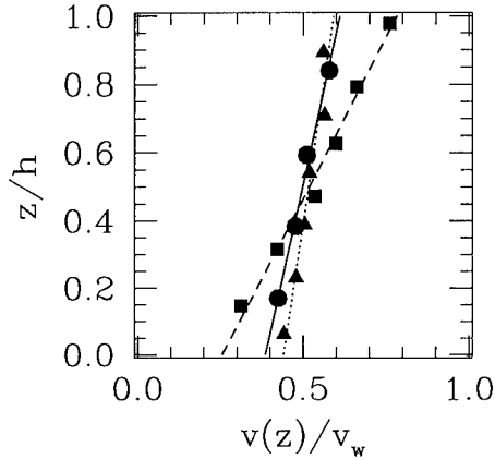
Figure 2: Velocity profiles at v_w = 200 m/s for hexadecane: at \epsilon_w = 0.1 kcal/mol ( \blacktriangle ) and \epsilon_w = 0.7 kcal/mol ( \blacksquare ) and for squalane: \epsilon_w = 0.7 kcal/mol ( \bullet ).
