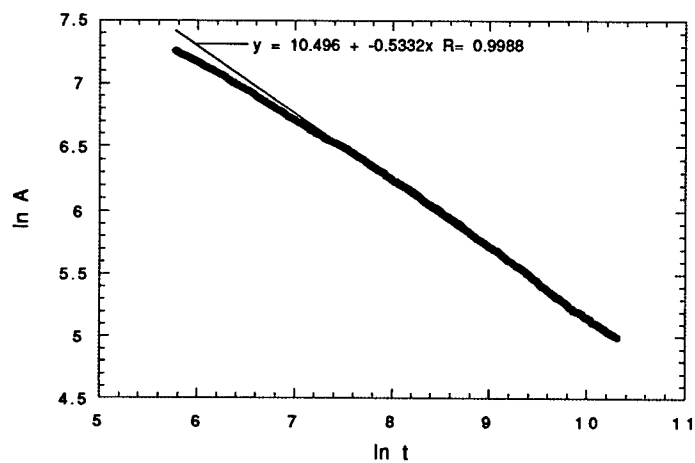
Fig.2 \ln A vs. \ln t for A+2B \rightarrow 0 reaction using the "intermediate" method on a 2d lattice.
