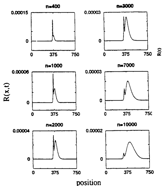
FIG. 5 Numerical results for the time evolution of the spatial profile of the local production rate R(x,t) , for k_1 = 1 , k_2 = 10^{-4} , and a_1 = 3\% , a_2 = 97\% of the total A density. The front's initial position is at 375.
