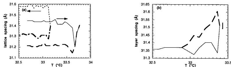
Figure 2. Values of the LC smectic layer spacing as a function of temperature: a) 0.88 \mu\text{m} , shown as a function of increasing as well as decreasing temperature; b) 9 \mu\text{m} , shown as a function of increasing temperature for clarity.
