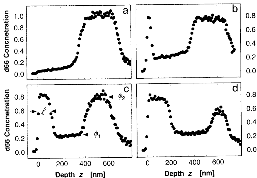
FIG. 3. Concentration-depth profiles for the d66/h52 couple annealed at 110^\circ\text{C} , determined by nuclear reaction analysis; (a) unannealed, (b) after 18h, (c) after 190h and (d) after 720h. The glass transition temperature for this couple is ca. -60^\circ\text{C} , and some interdiffusion can be observed in the unannealed sample due to the sample handling at room temperature.
