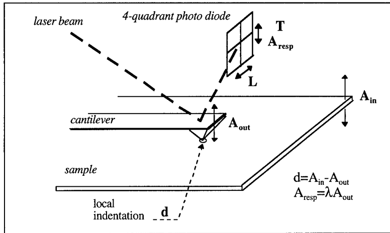
Figure 1: Laser Beam Detection Scheme of a 3-fold AFM Set-up. Topography (T), lateral forces (L) and viscoelastic response ( A_{\text{resp}} ) are measured simultaneously while scanning the cantilever. The input modulation ( A_{\text{in}} ) is either applied at the sample stage (sketched) or cantilever stage. The force modulation response amplitude is calibrated with \lambda . Amplitude and phase relation between the modulation signals provide local information about the viscoelastic properties of the sample surface.
