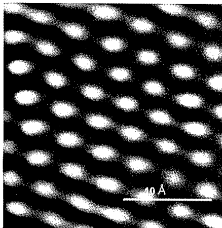
Figure 2. STM image of bulk MoS 2 basal plane.
