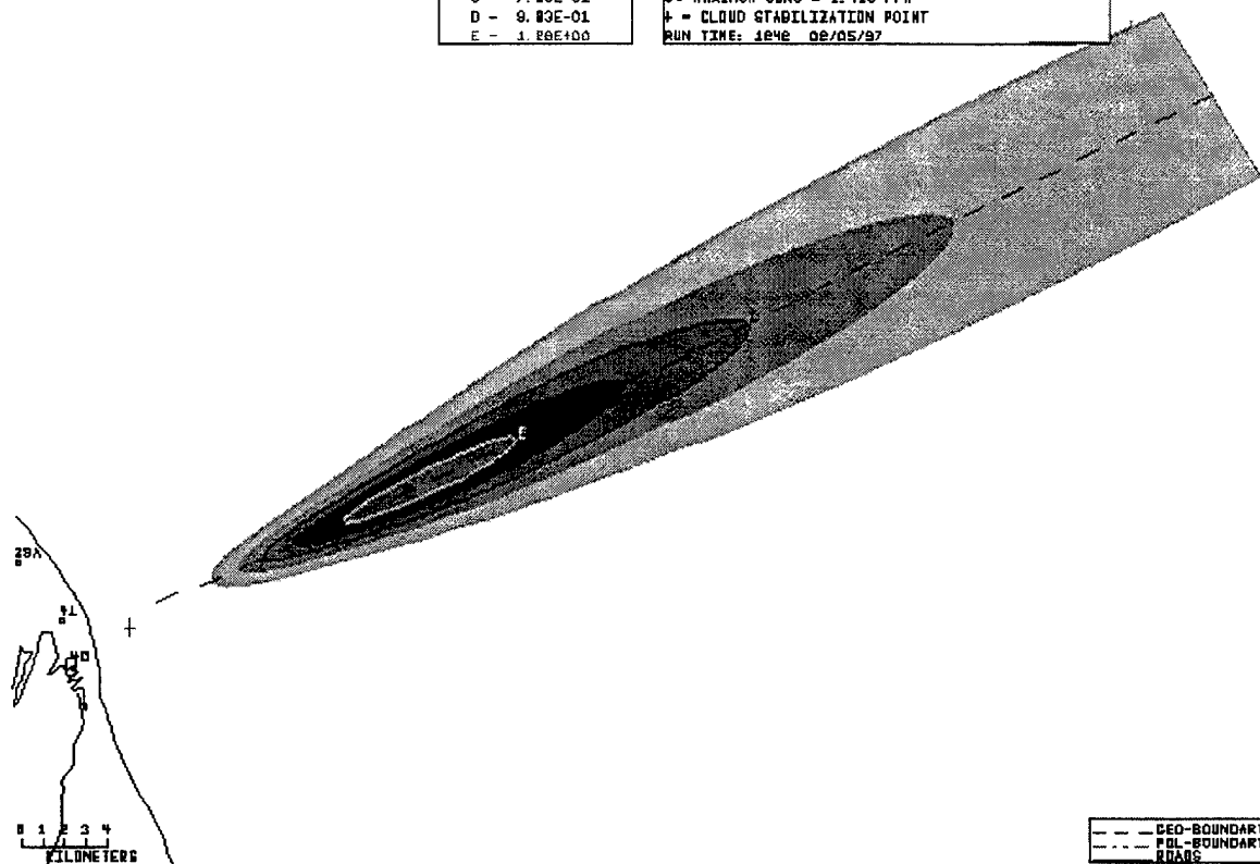
Figure A6. HCl surface height concentration isopleth predictions from REEDM Version 7.07 for #K2 mission using T-0.8h rawinsonde data.
