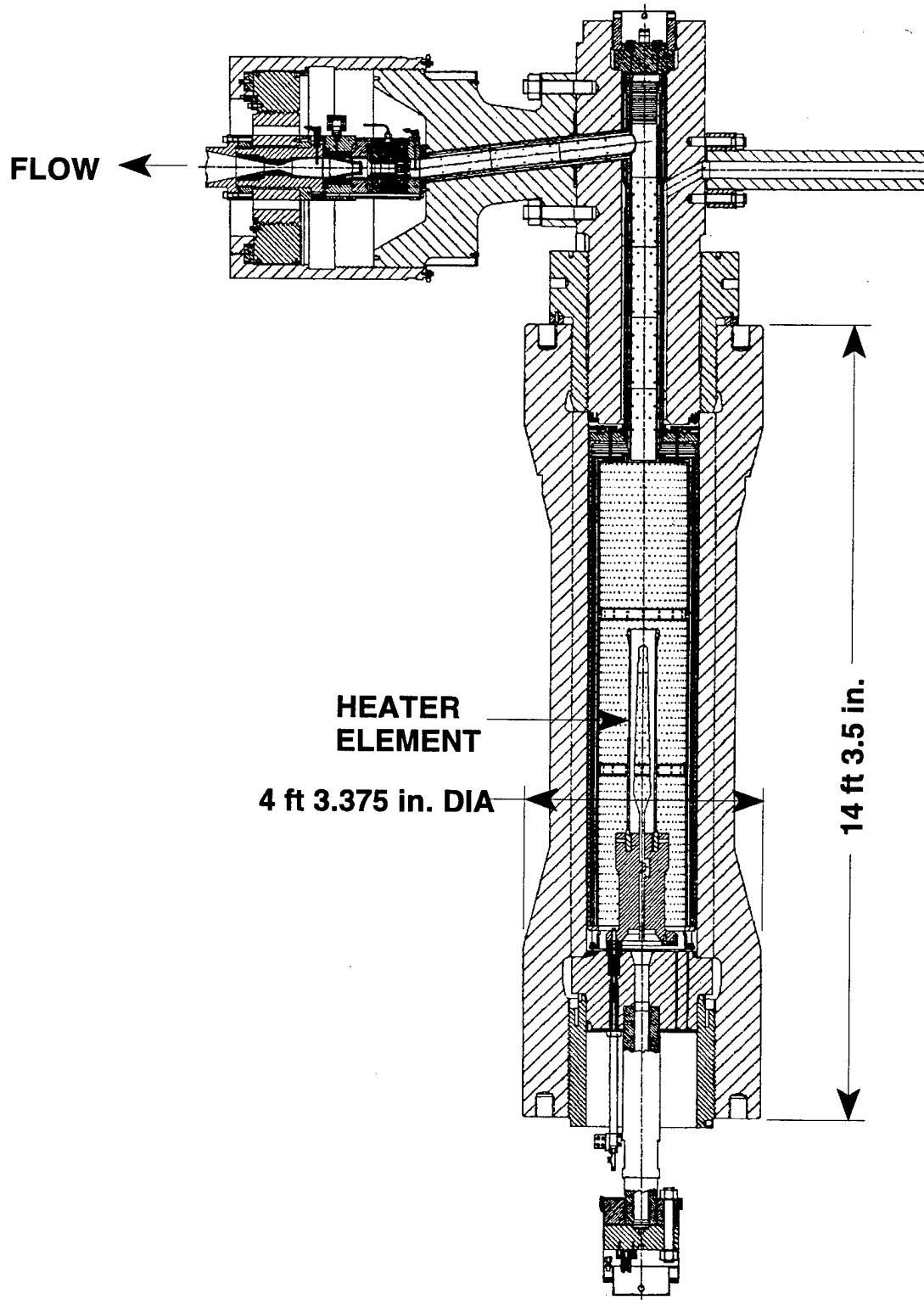
FIGURE 1. VERTICAL HEATER AND DIAPHRAGM SECTION
