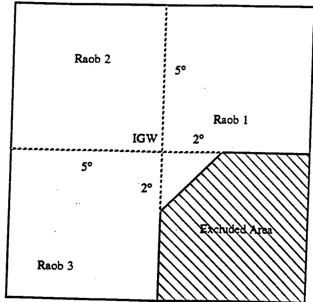
Figure 2. Diagram showing the 10° x 10° area in which the 3 closest soundings to the IGW are identified.
