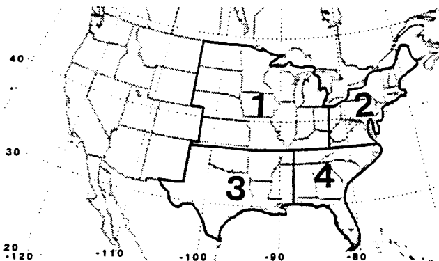
Fig. 3 Composite Regions: 1=Midwest, 2=Northeast, 3=S. Plains, 4=Southeast
