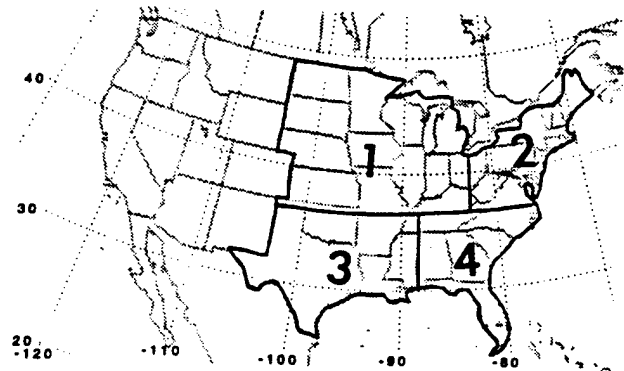
Fig. 3 Composite Regions: 1=Midwest, 2=Northeast, 3=S. Plains, 4=Southeast
