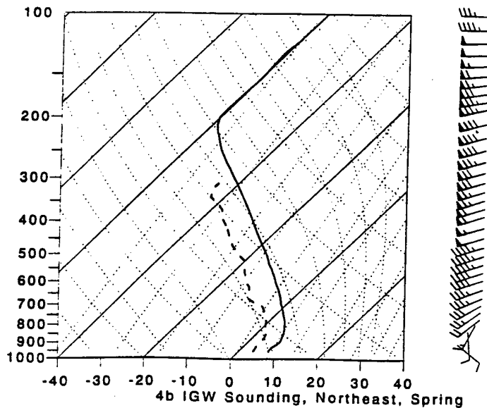
Figure 4. Skew-T Log-P diagram of IGW composite soundings. Temperature ( ^{\circ}\text{C} , solid), dewpoint ( ^{\circ}\text{C} , dashed), wind barbs (kts): (a) winter Midwest; (b) spring Northeast.
