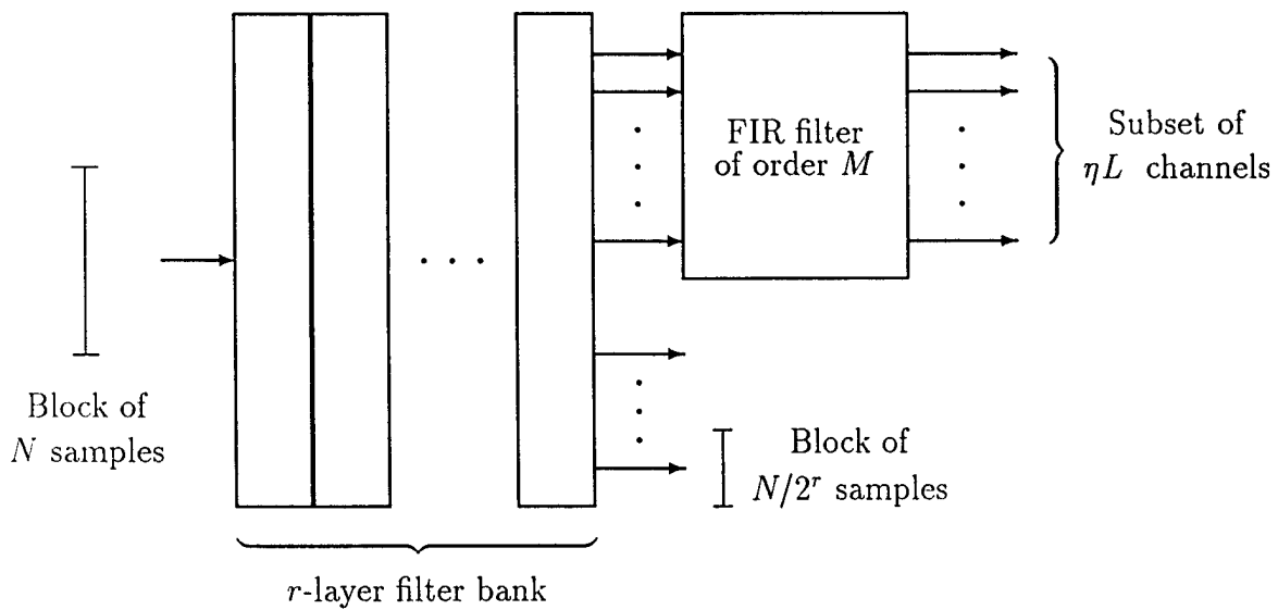
Figure 10: Structure of subband-domain (suboptimal) estimator.
